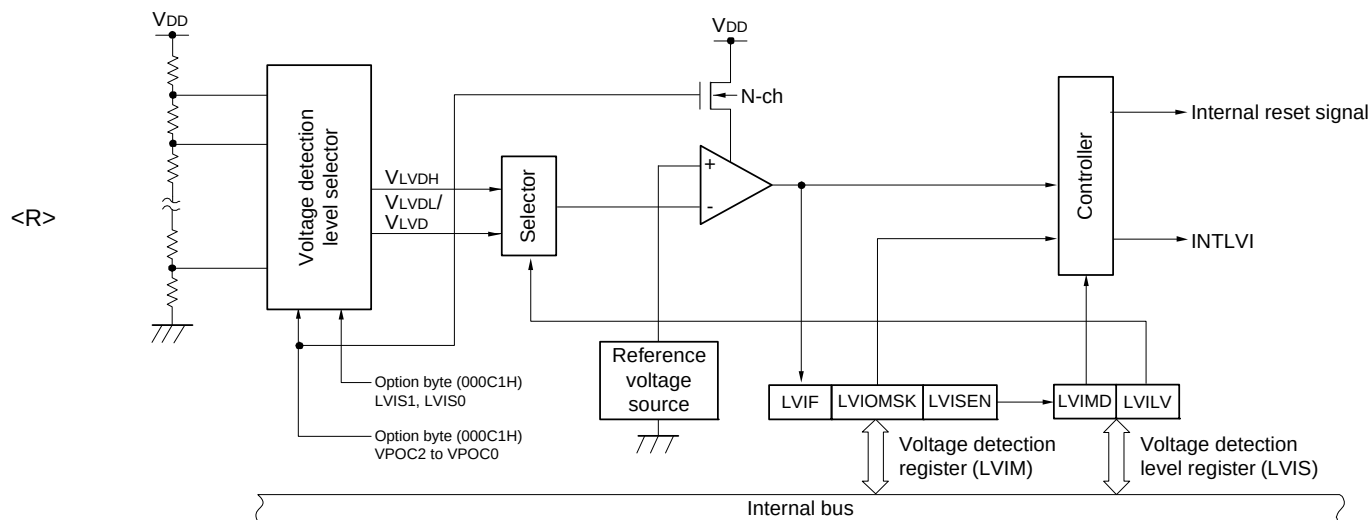
Figure 23 - 1 Block Diagram of Voltage Detector
