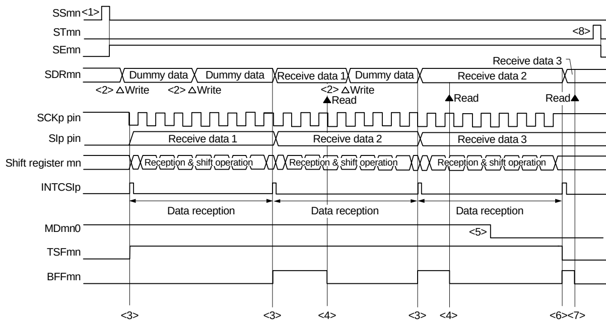
<R> Figure 14 - 42 Timing Chart of Master Reception (in Continuous Reception Mode) (Type 1: DAPmn = 0, CKPmn = 0)
