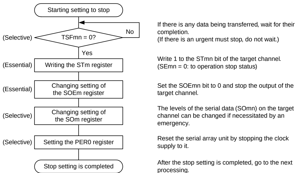
Figure 14 - 110 Procedure for Stopping UART Transmission
