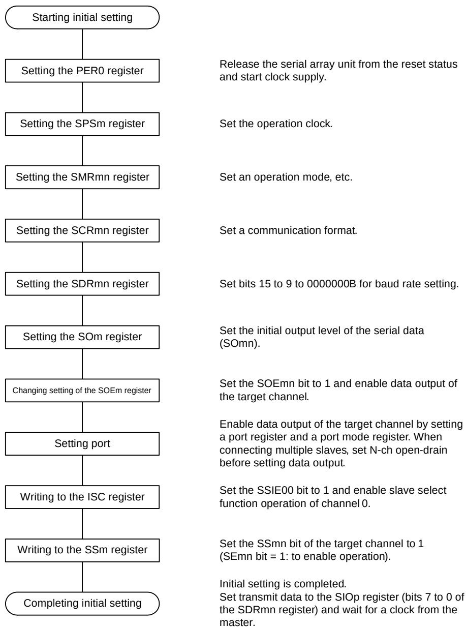
Figure 14 - 83 Initial Setting Procedure for Slave Transmission
