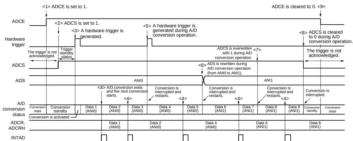
<R> Figure 13 - 23 Example of Hardware Trigger No-Wait Mode (Select Mode, Sequential Conversion Mode) Operation Timing
