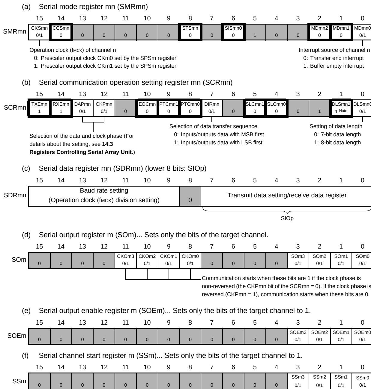
Figure 14 - 44 Example of Contents of Registers for Master Transmission/Reception of 3-Wire Serial I/O (CSI00, CSI01, CSI10, CSI11, CSI20, CSI21)
