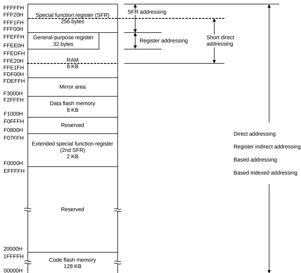
Figure 3 - 3 Correspondence Between Data Memory and Addressing
