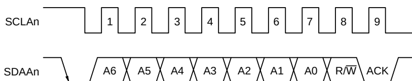
Figure 15 - 24 ACK
