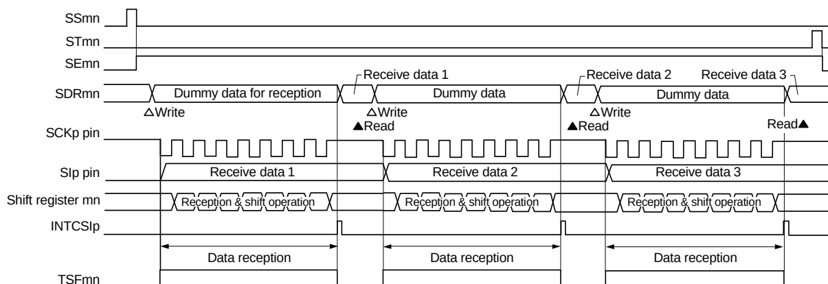
Figure 14 - 40 Timing Chart of Master Reception (in Single-Reception Mode)
