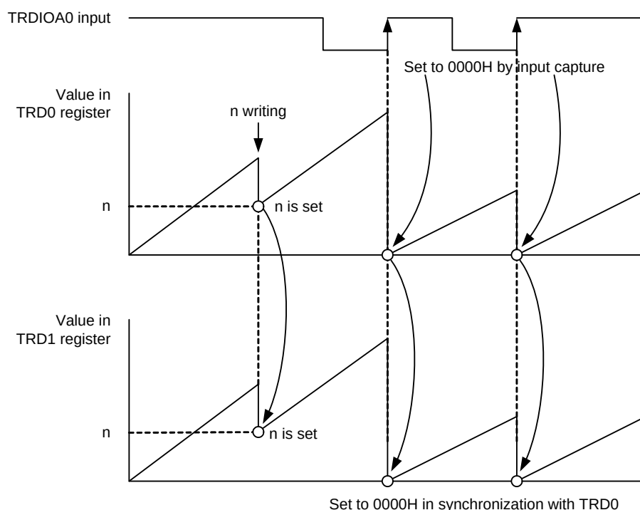
Figure 8 - 44 Synchronous Operation
