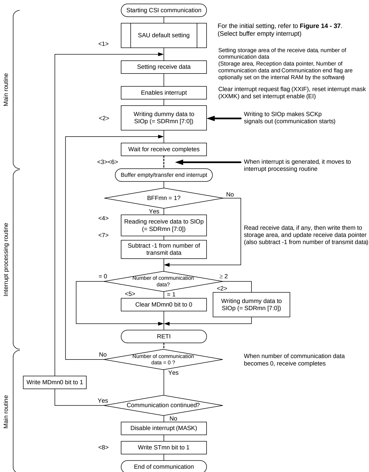
<R> Figure 14 - 43 Flowchart of Master Reception (in Continuous Reception Mode)
