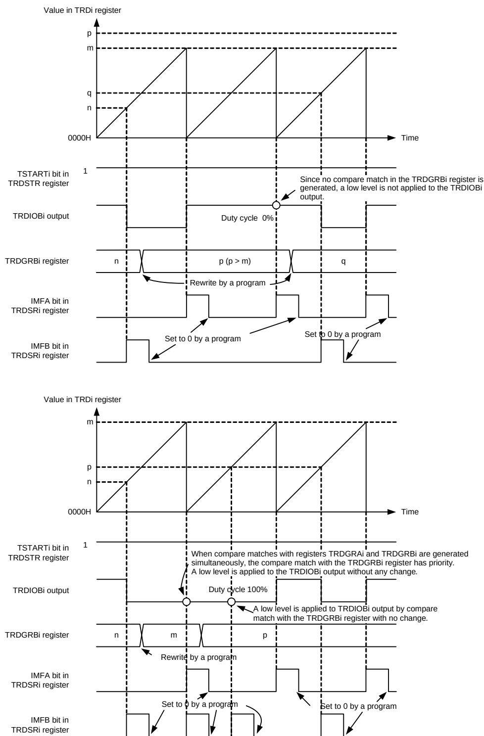
Figure 8 - 55 Operation Example in PWM Function (Duty Cycle 0%, Duty Cycle 100%)
