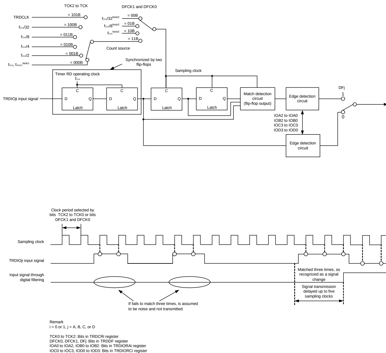
Figure 8 - 48 Block Diagram of Digital Filter
