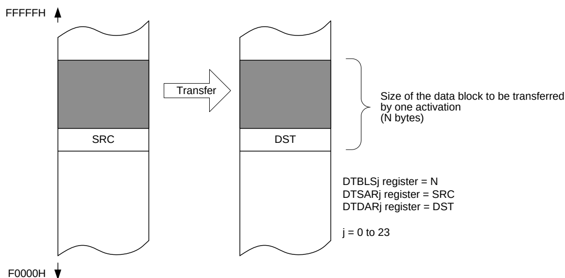
Figure 16 - 14 Data Transfers in Normal Mode
