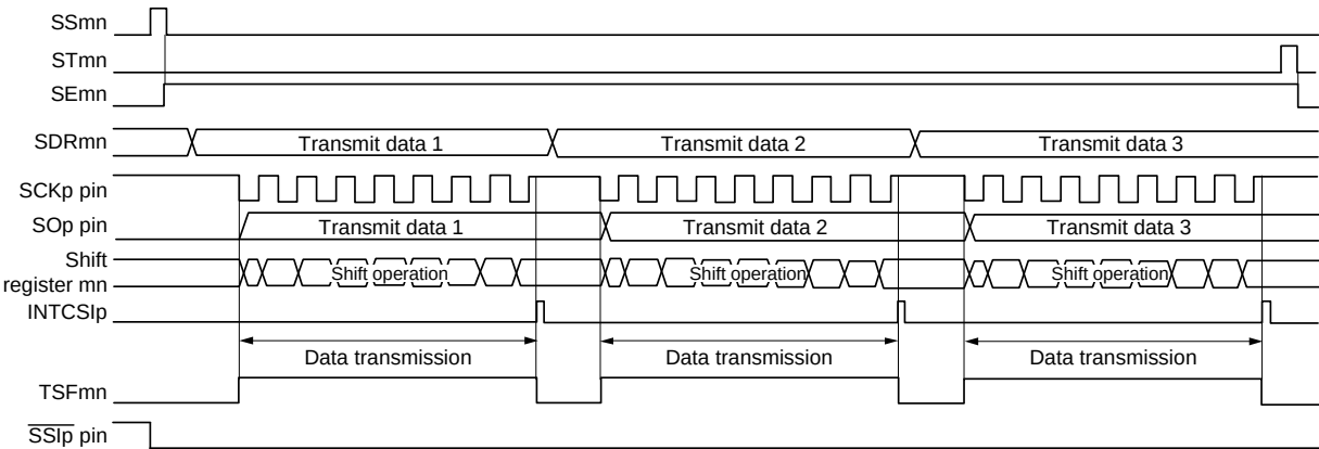
Figure 14 - 86 Timing Chart of Slave Transmission (in Single-Transmission Mode) (Type 1: DAPmn = 0, CKPmn = 0)
