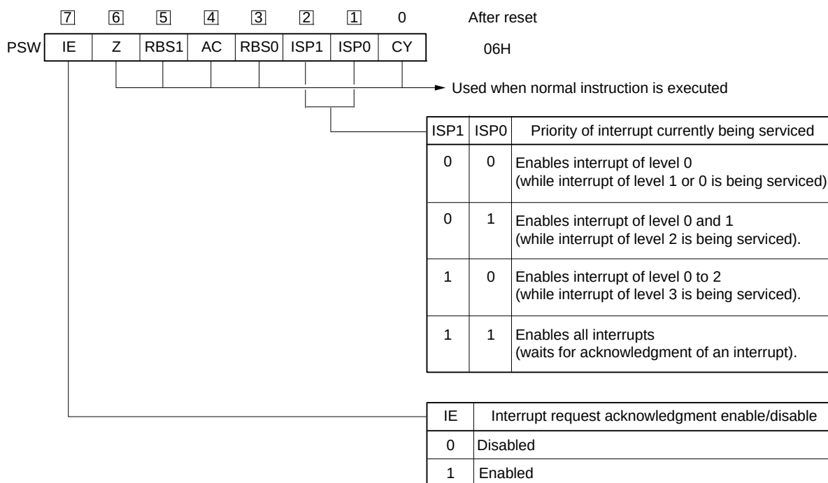
Figure 18 - 11 Configuration of Program Status Word
