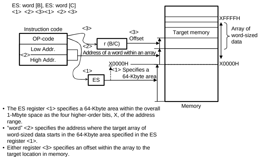
Figure 3 - 28 Example of ES:word[B], ES:word[C]
