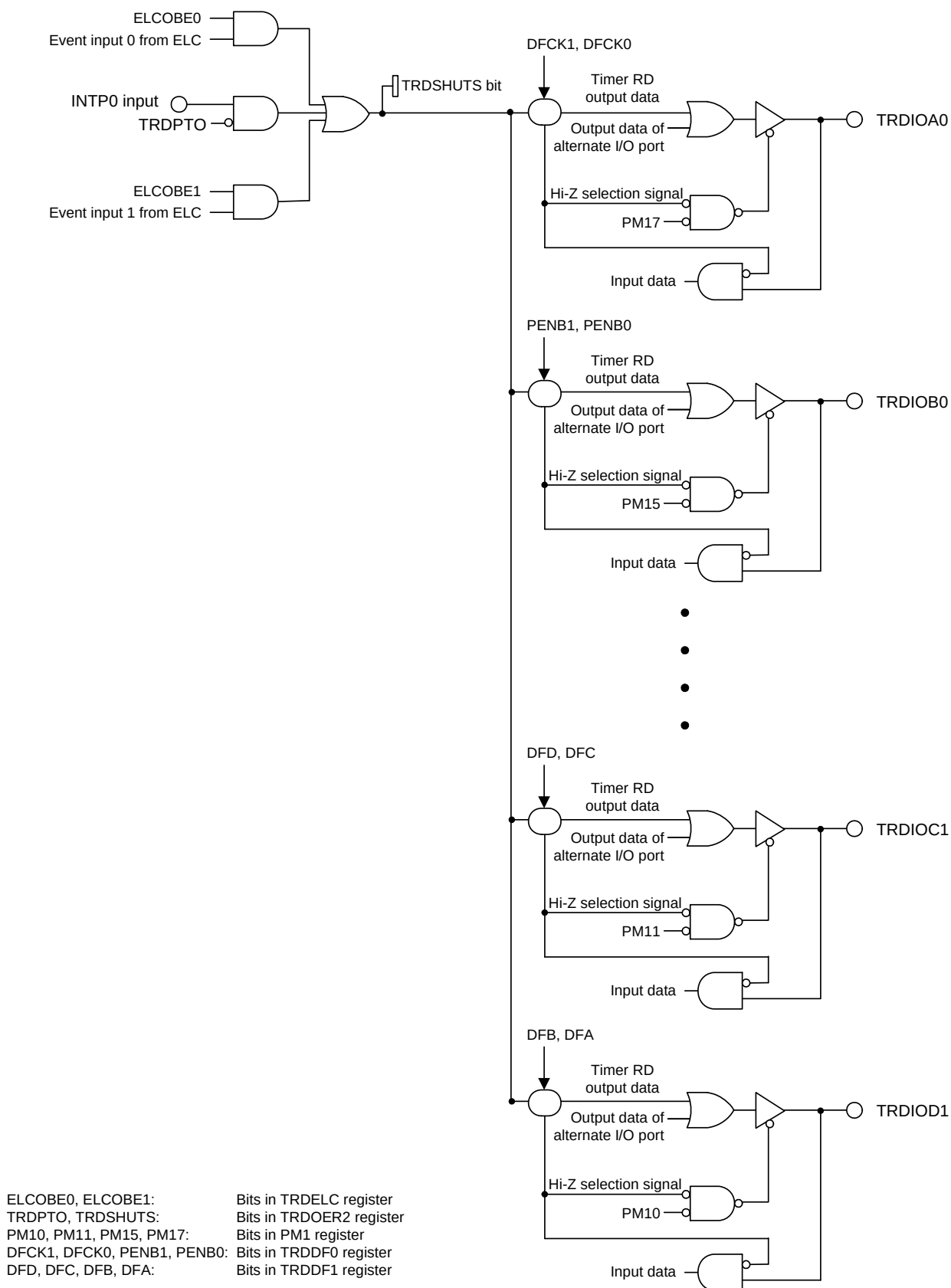
Figure 8 - 45 Pulse Output Forced Cutoff
