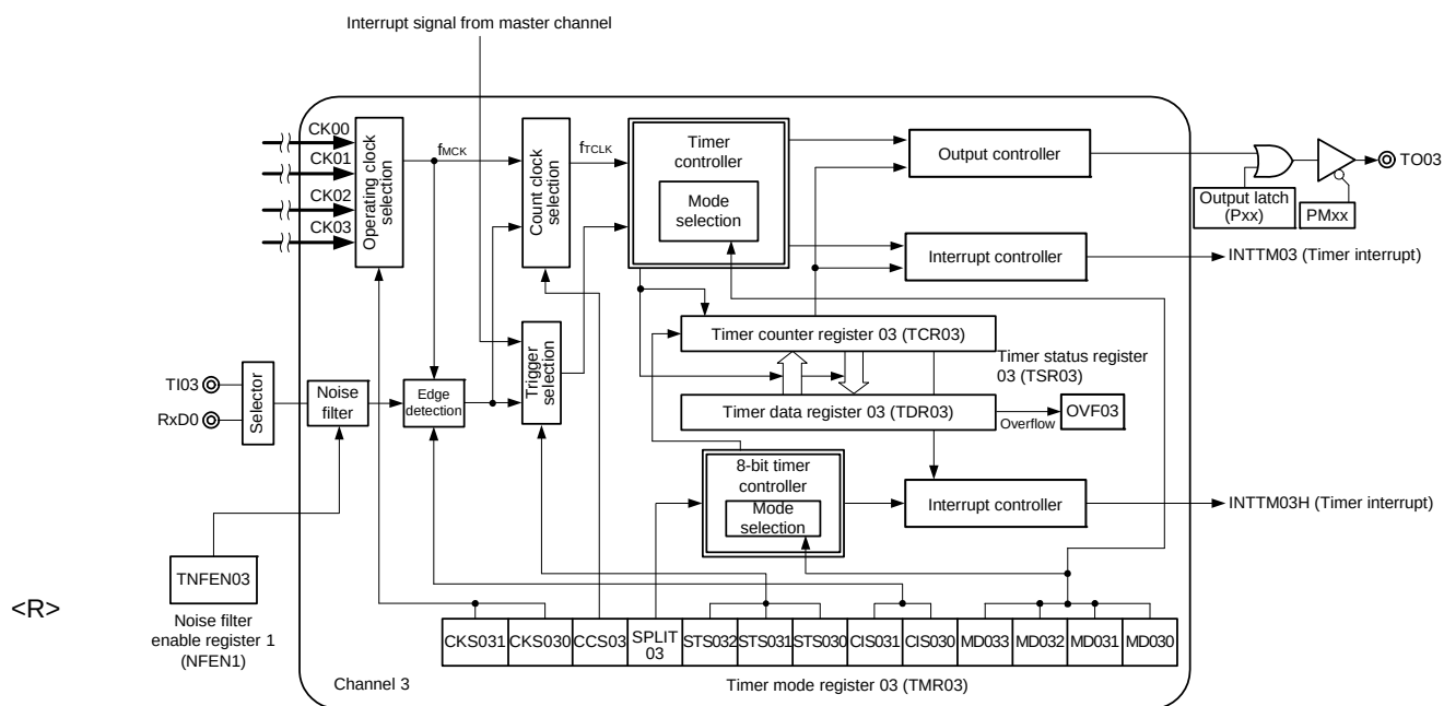
Figure 6 - 5 Internal Block Diagram of Channel 3 of Timer Array Unit 0
