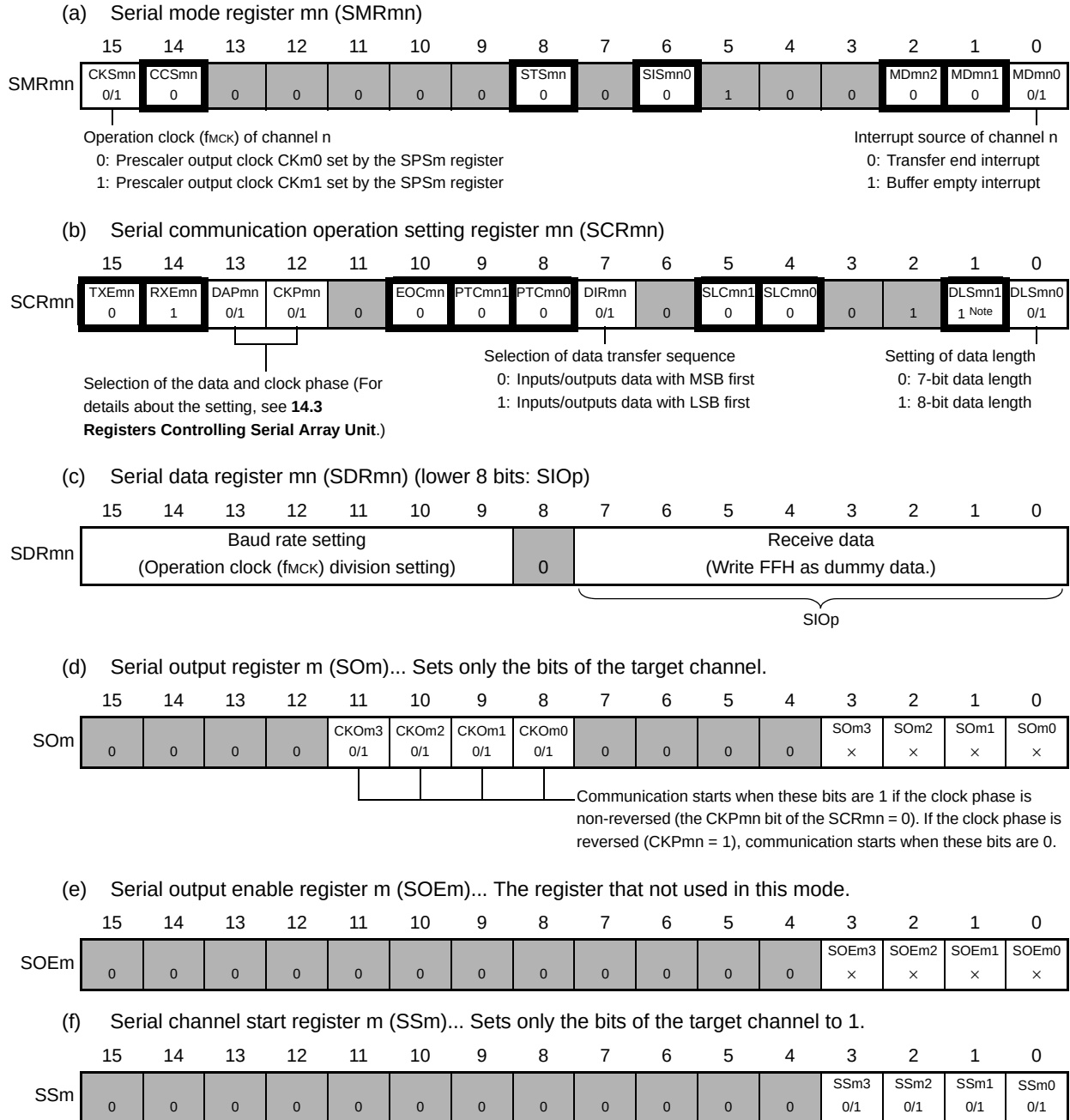
Figure 14 - 36 Example of Contents of Registers for Master Reception of 3-Wire Serial I/O (CSI00, CSI01, CSI10, CSI11, CSI20, CSI21)
