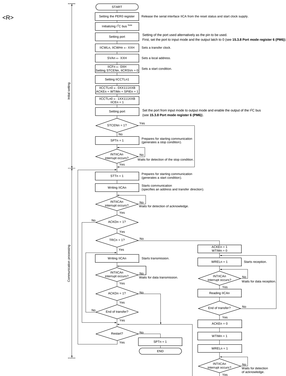
Figure 15 - 35 Master Operation in Single-Master System
