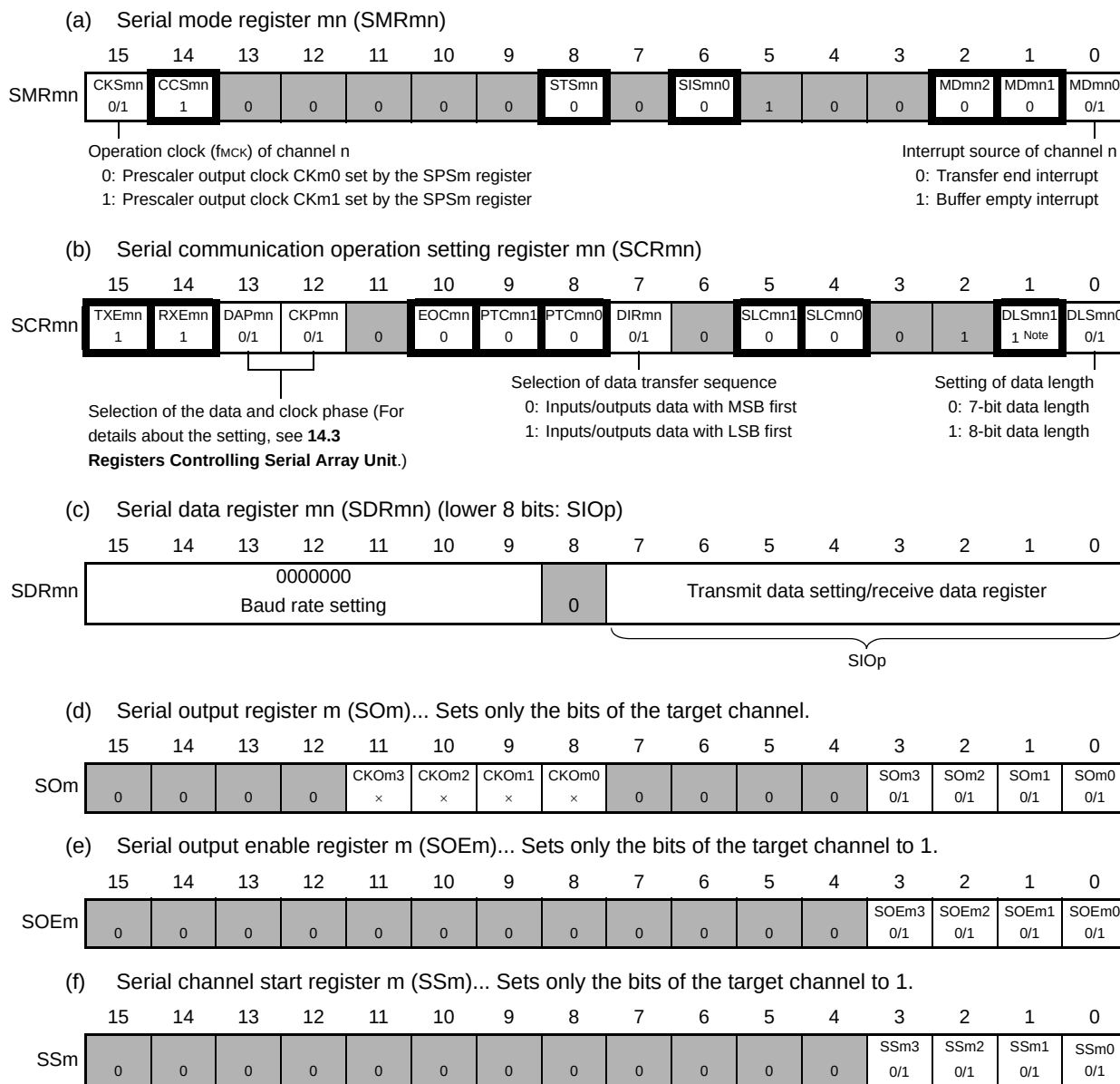
Figure 14 - 66 Example of Contents of Registers for Slave Transmission/Reception of 3-Wire Serial I/O (CSI00, CSI01, CSI10, CSI11, CSI20, CSI21)
