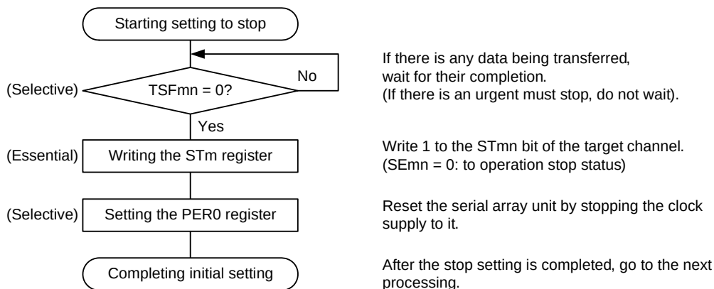
Figure 14 - 119 Procedure for Stopping UART Reception
