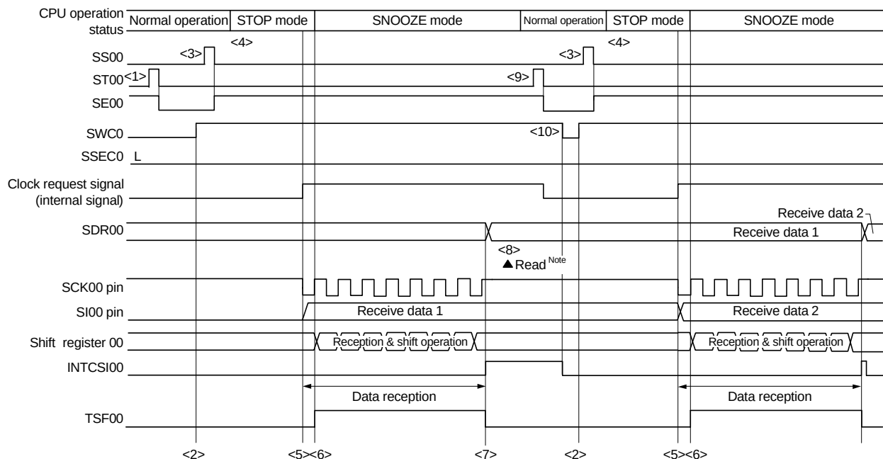
<R> Figure 14 - 76 Timing Chart of SNOOZE Mode Operation (continuous startup) (Type 1: DAPmn = 0, CKPmn = 0)
