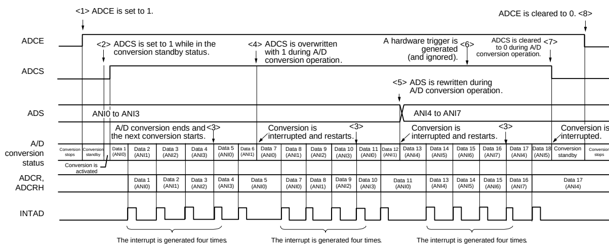
Figure 13 - 21 Example of Software Trigger Mode (Scan Mode, Sequential Conversion Mode) Operation Timing
