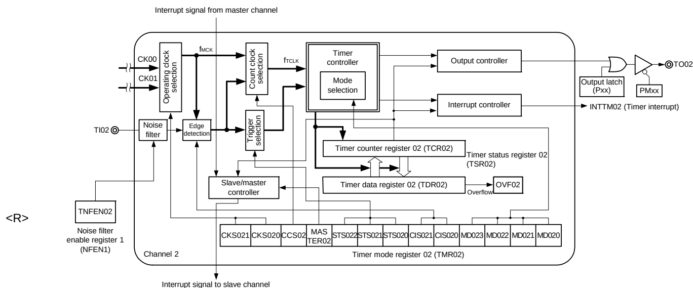
Figure 6 - 4 Internal Block Diagram of Channel 2 of Timer Array Unit 0
