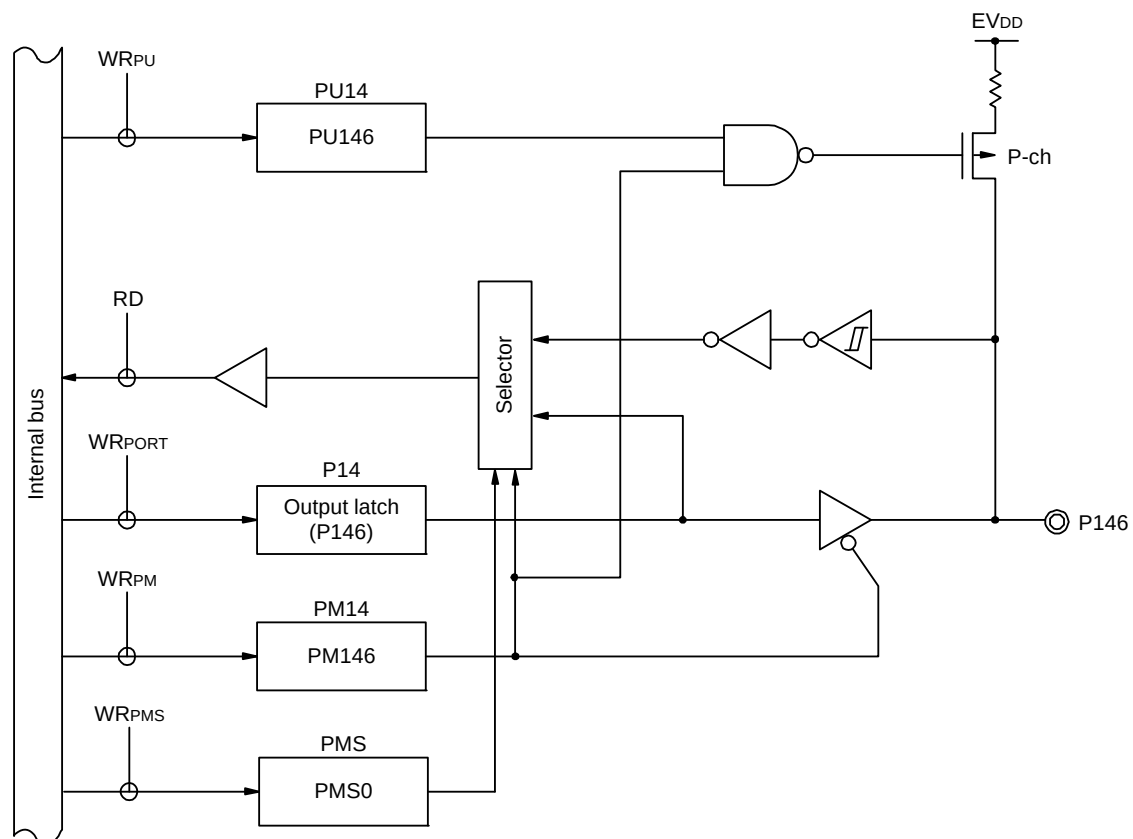
Figure 4 - 41 Block Diagram of P146
