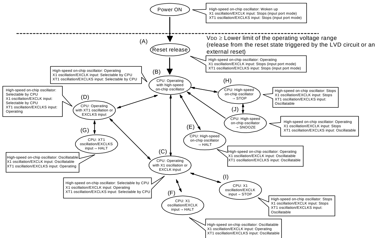
Figure 5 - 20 CPU Clock Status Transition Diagram
