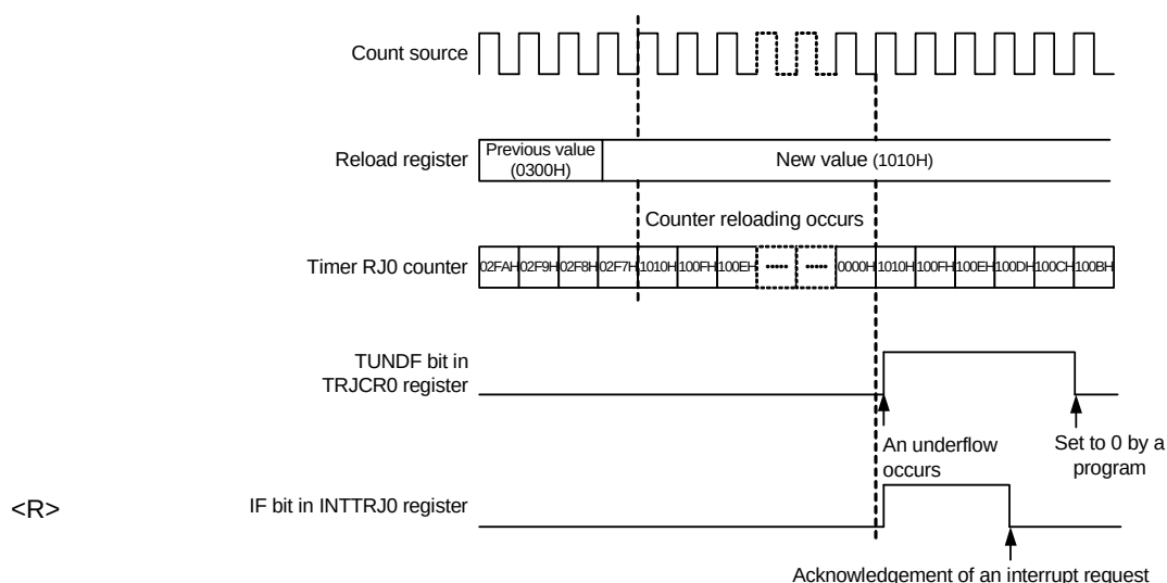
Figure 7 - 11 Operation Example in Timer Mode
