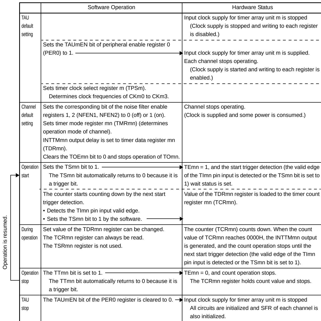
Figure 6 - 69 Operation Procedure When Delay Counter Function Is Used
