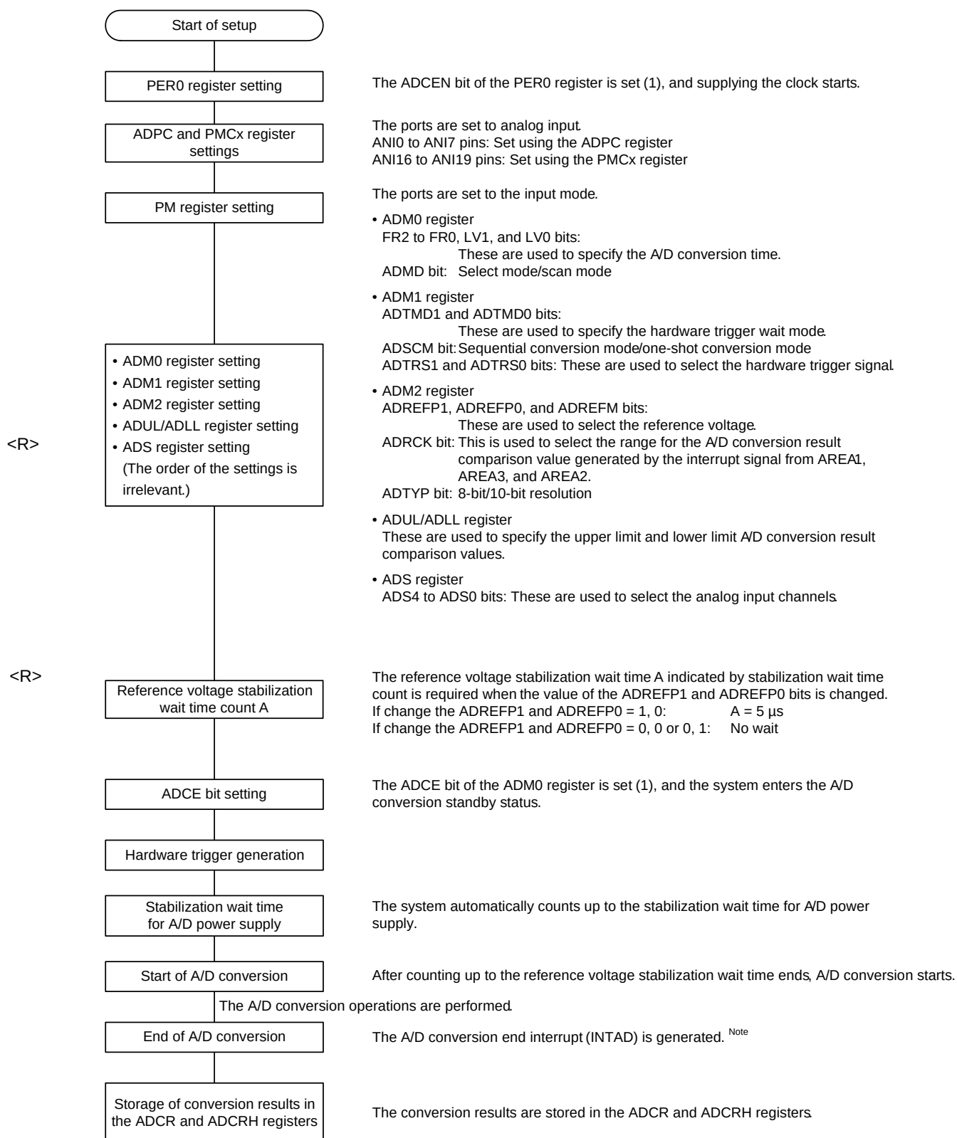
Figure 13 - 33 Setting up Hardware Trigger Wait Mode
