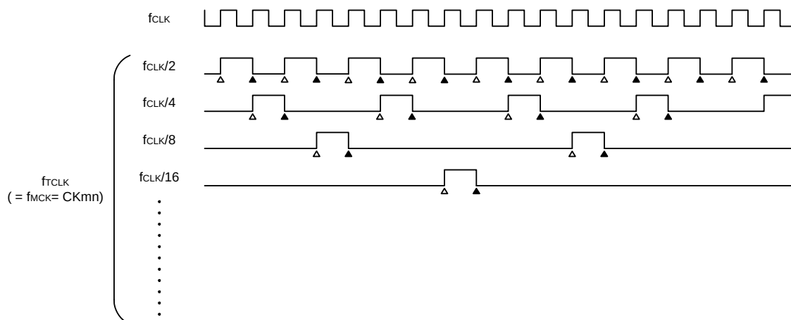
Figure 6 - 27 Timing of f CLK and count clock (f CLK ) (When CCS mn = 0)
