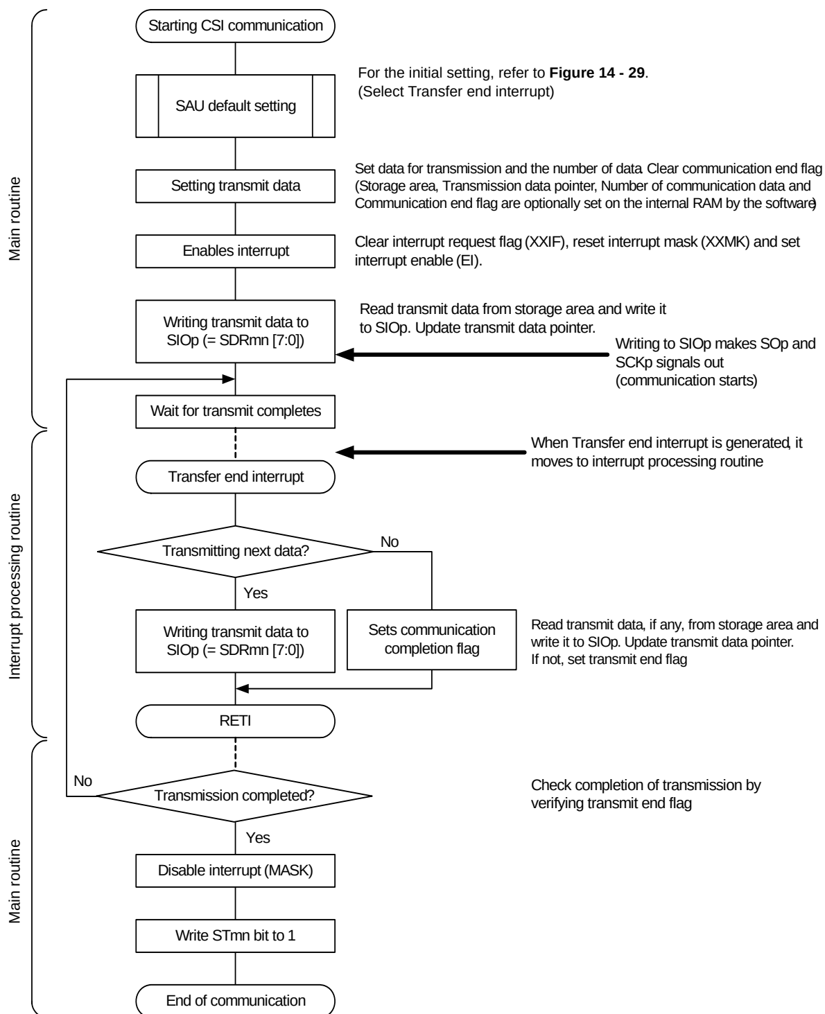
<R> Figure 14 - 33 Flowchart of Master Transmission (in Single-Transmission Mode)
