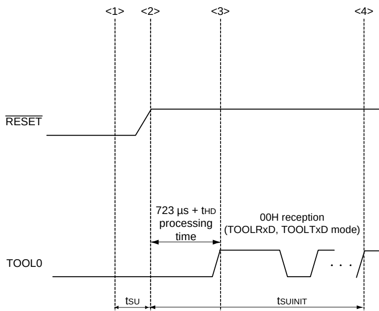
Figure 27 - 7 Setting of Flash Memory Programming Mode
