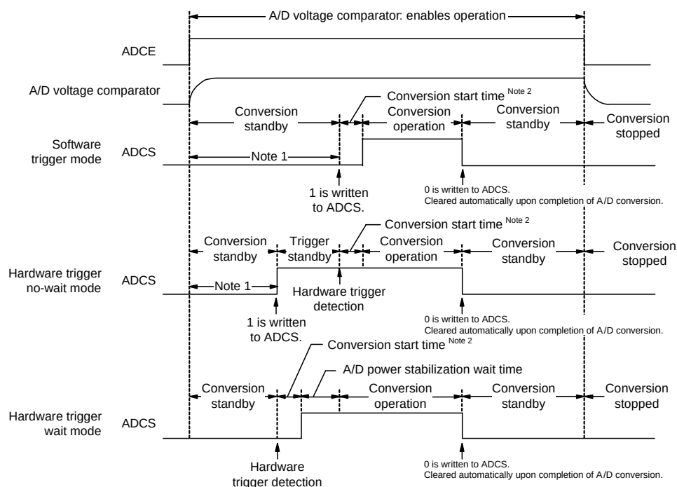
<R> Figure 13 - 4 Timing Chart When A/D Voltage Comparator Is Used
