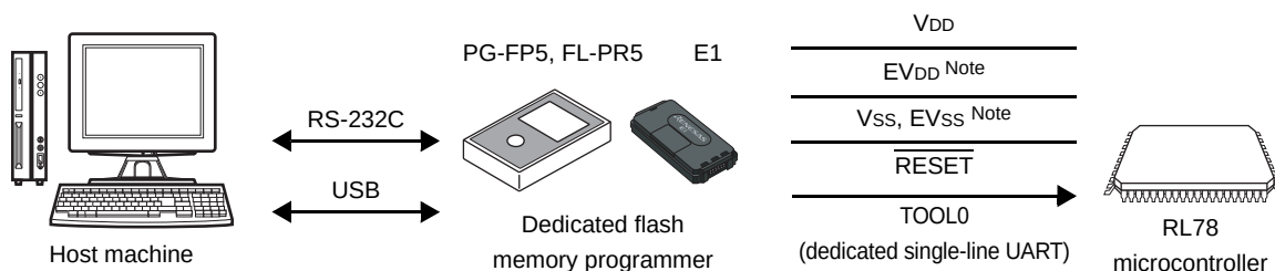
Figure 27 - 1 Environment for Writing Program to Flash Memory
