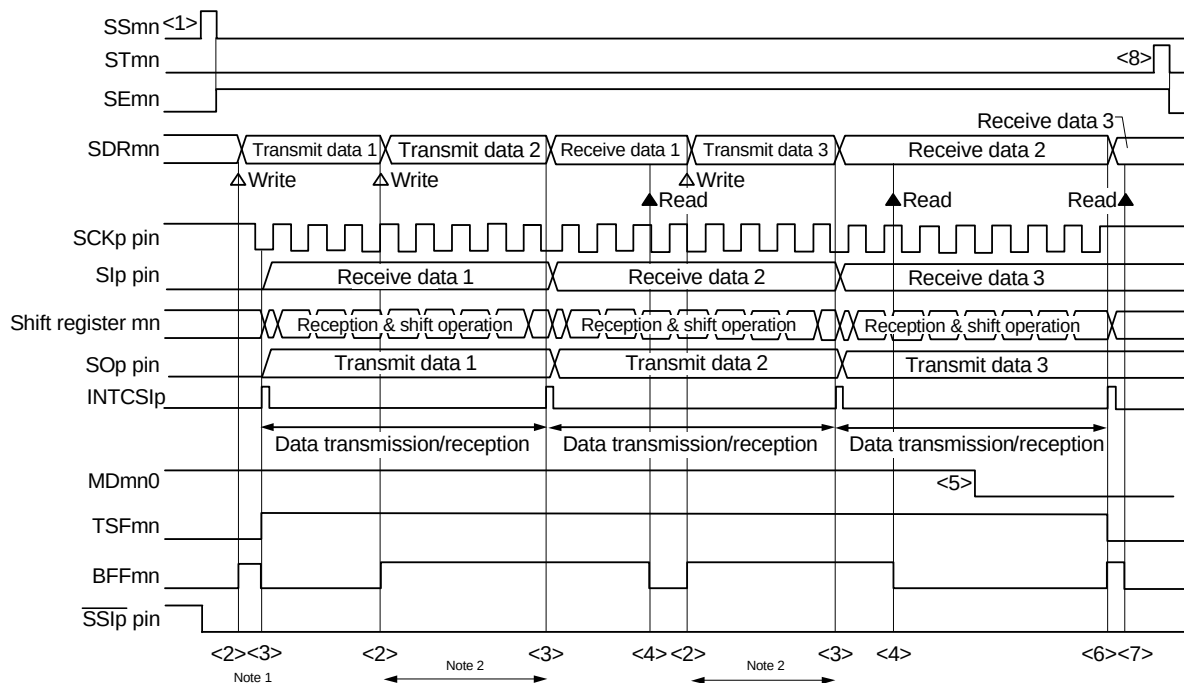
<R> Figure 14 - 104 Timing Chart of Slave Transmission/Reception (in Continuous Transmission/Reception Mode) (Type 1: DAPmn = 0, CKPmn = 0)
