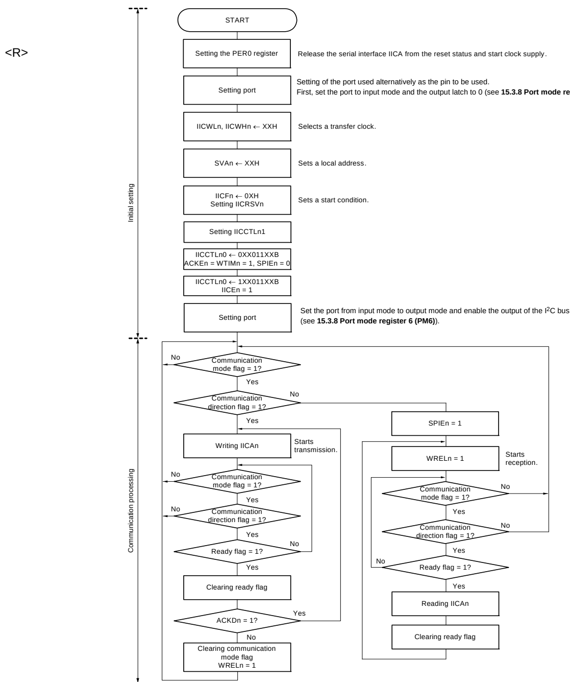
Figure 15 - 39 Slave Operation Flowchart (1)
