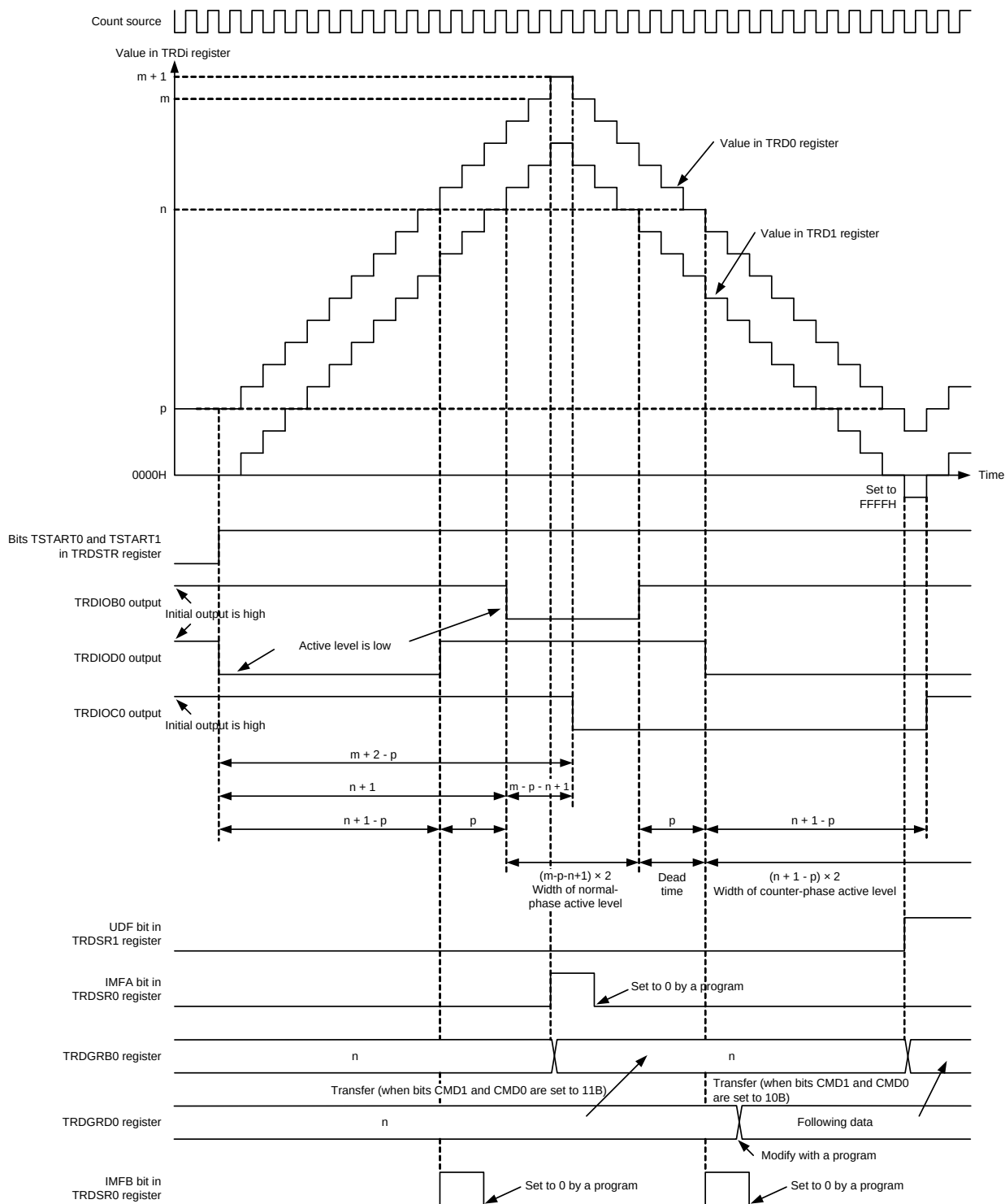
Figure 8 - 60 Operation Example in Complementary PWM Mode
