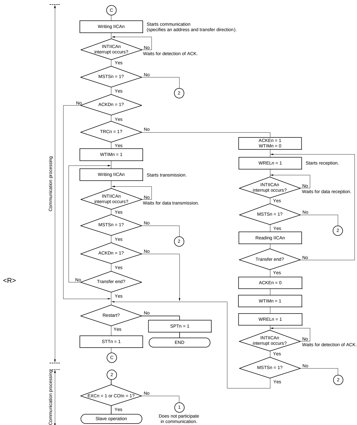
Figure 15 - 38 Master Operation in Multi-Master System (3/3)
