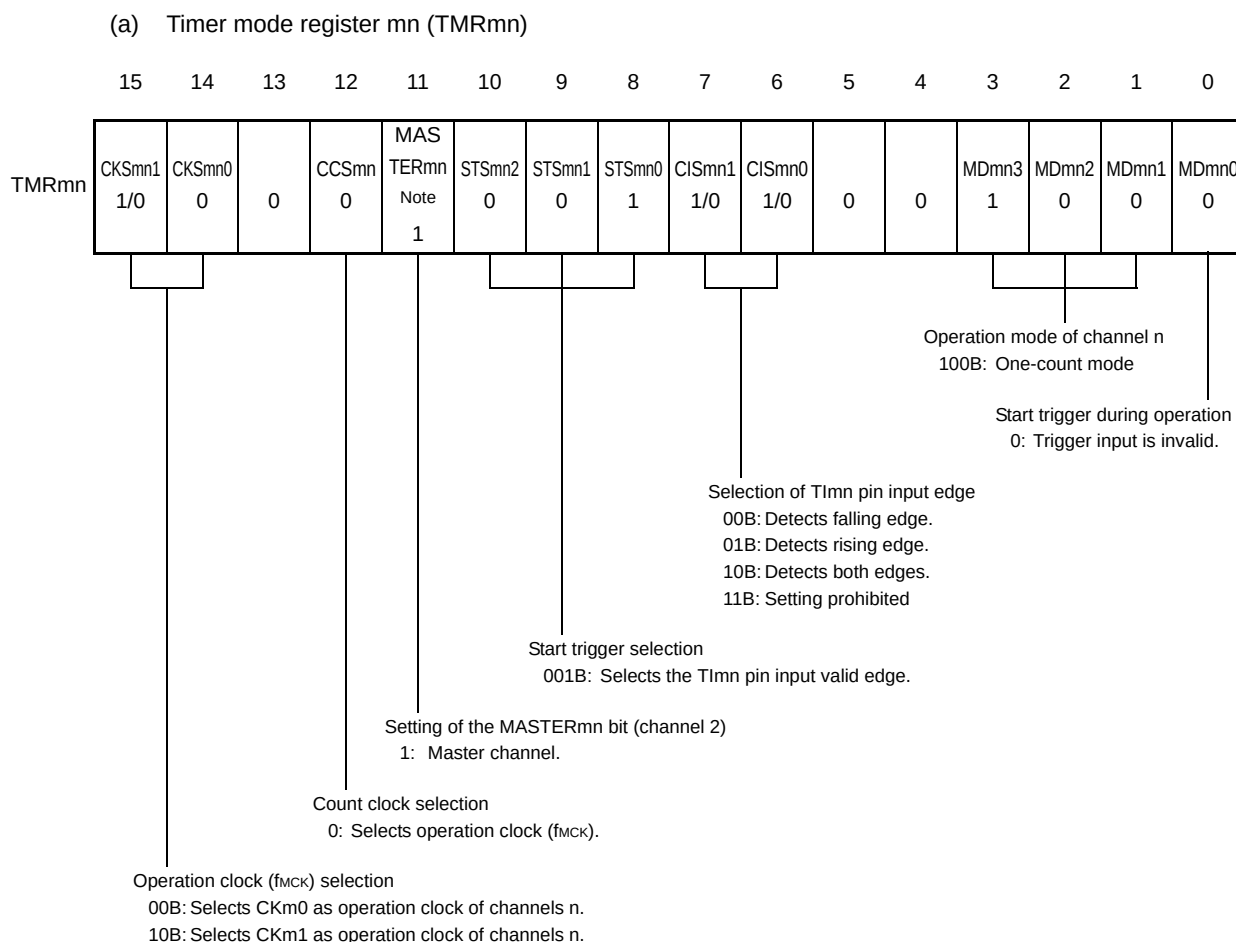
Figure 6 - 72 Example of Set Contents of Registers When One-Shot Pulse Output Function Is Used (Master Channel)
