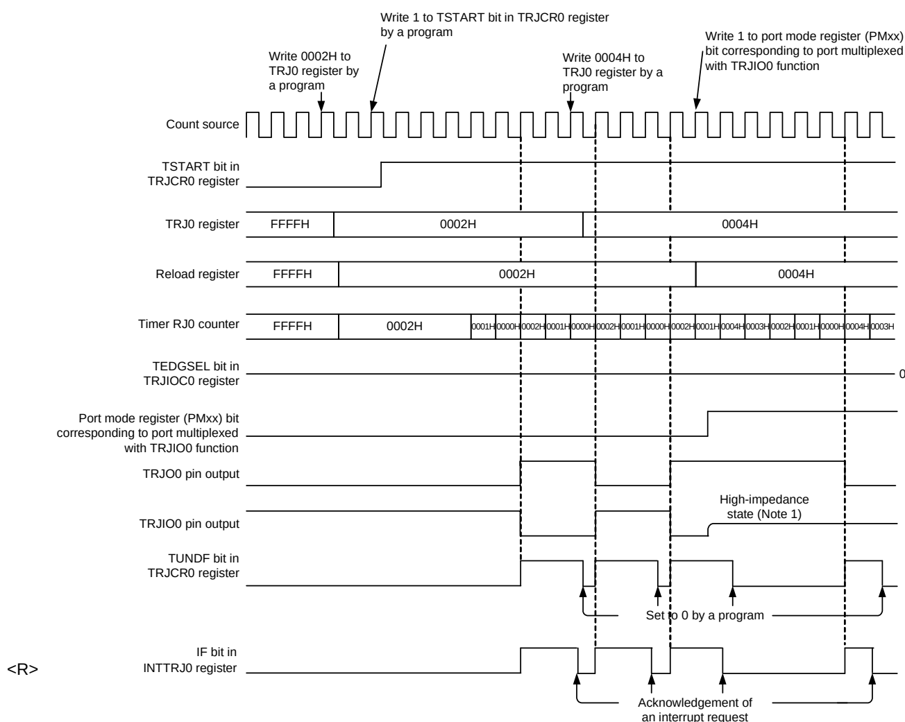
Figure 7 - 12 Operation Example in Pulse Output Mode
