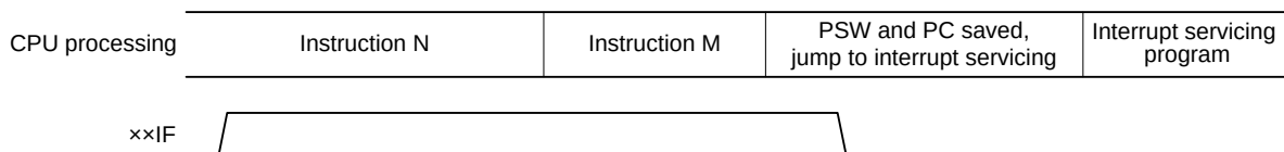
Figure 18 - 17 Interrupt Request Hold
