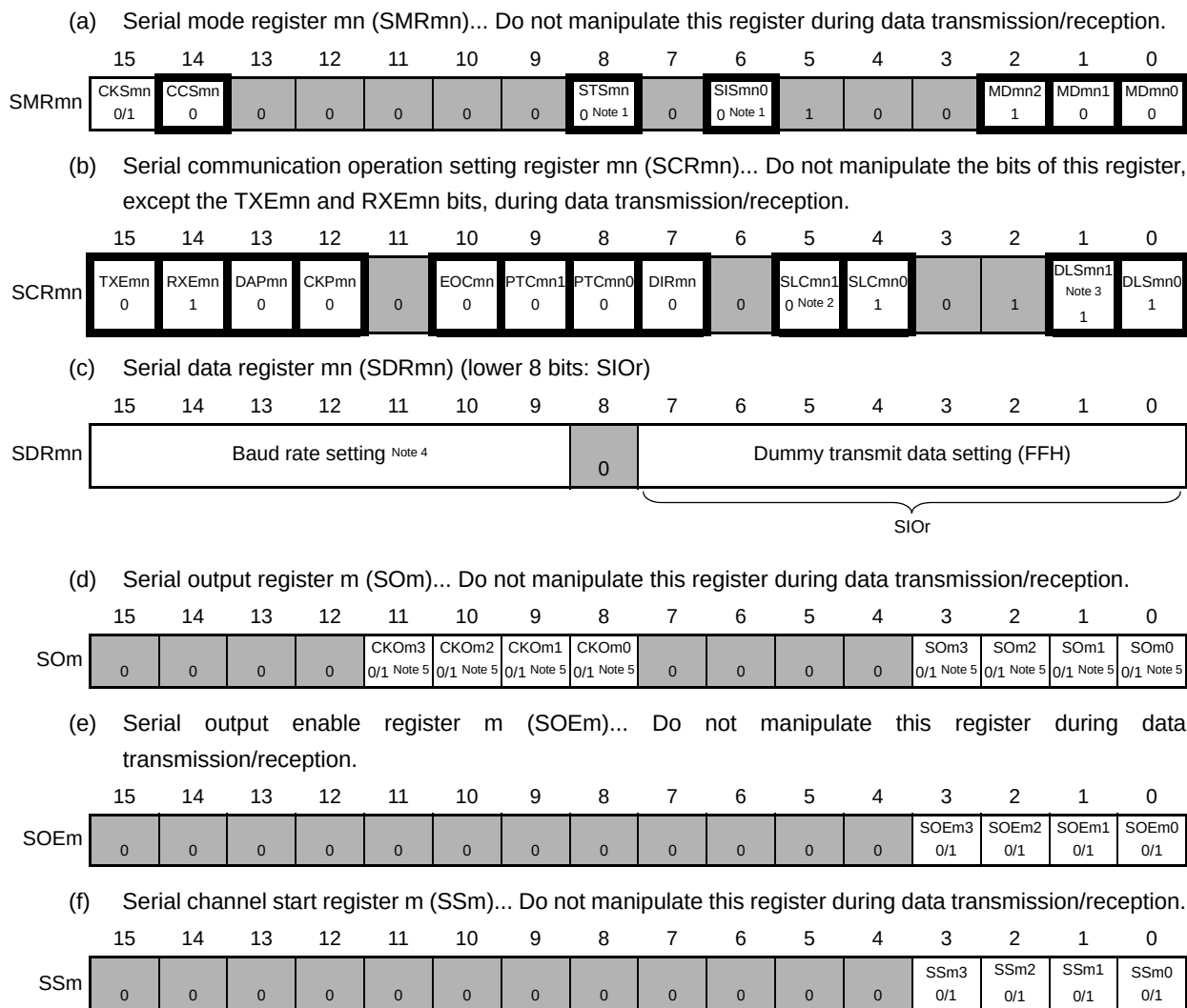
Figure 14 - 143 Example of Contents of Registers for Data Reception of Simplified I 2 C (IIC00, IIC01, IIC10, IIC11, IIC20, IIC21)
