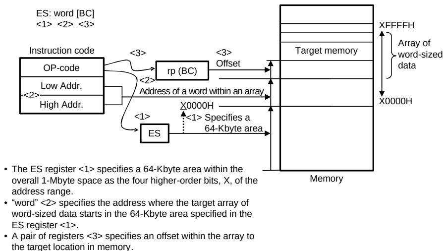
Figure 3 - 29 Example of ES:word[BC]
