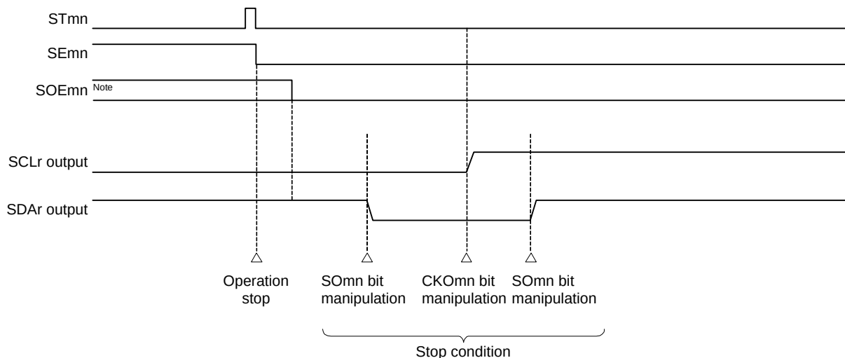
Figure 14 - 146 Timing Chart of Stop Condition Generation
