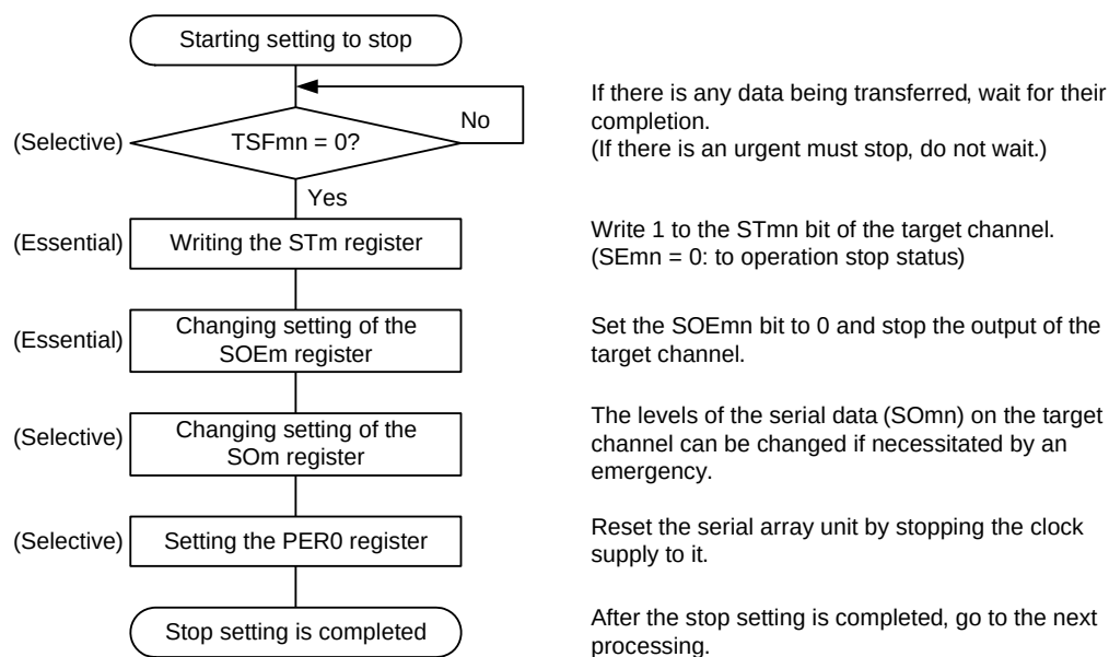
Figure 14 - 100 Procedure for Stopping Slave Transmission/Reception
