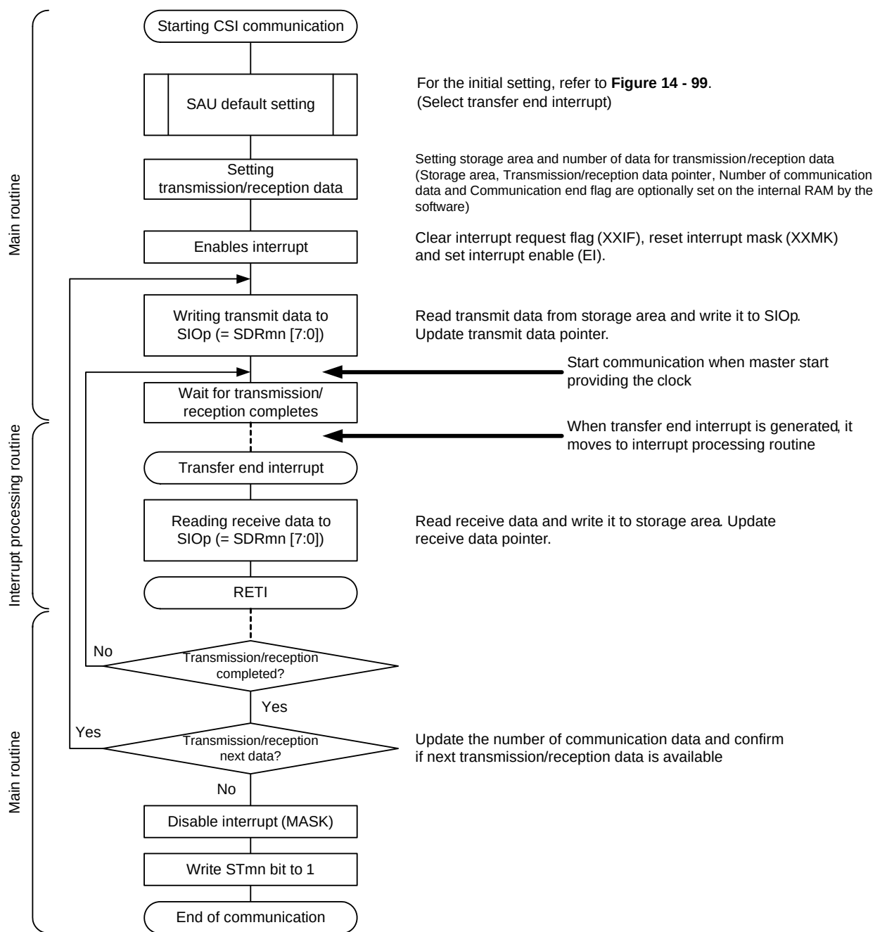
<R> Figure 14 - 103 Flowchart of Slave Transmission/Reception (in Single- Transmission/Reception Mode)
