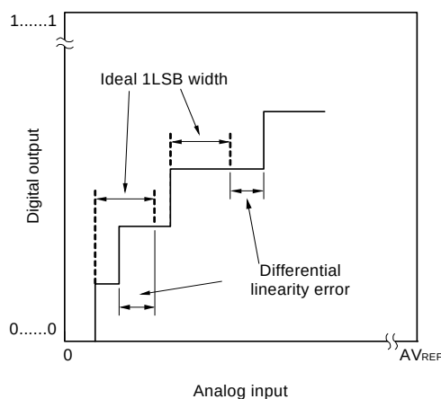
Figure 13 - 45 Differential Linearity Error
