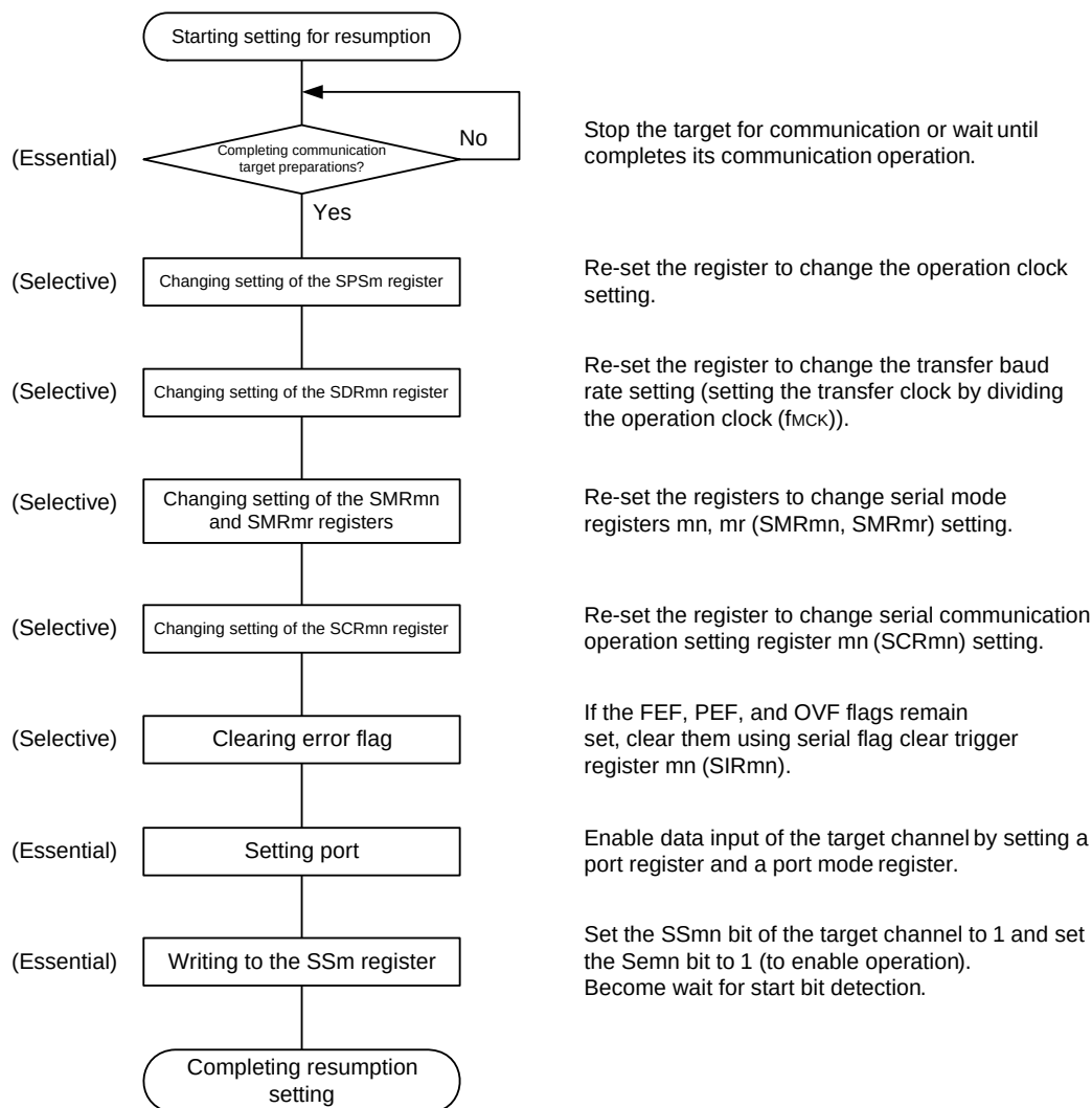
Figure 14 - 120 Procedure for Resuming UART Reception
