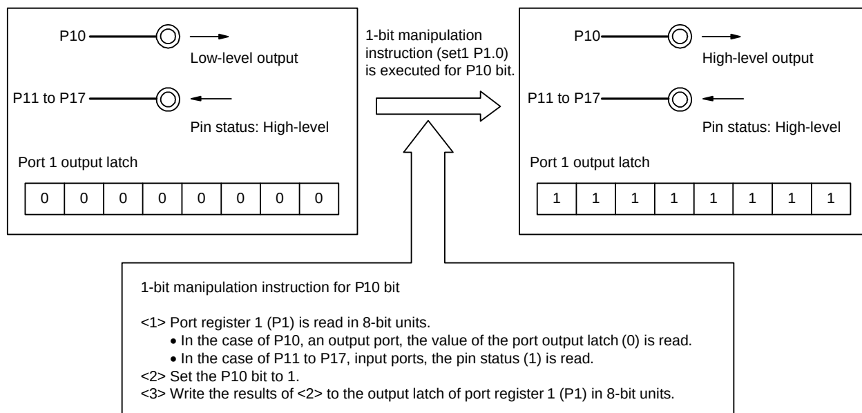
Figure 4 - 53 Bit Manipulation Instruction (P10)
