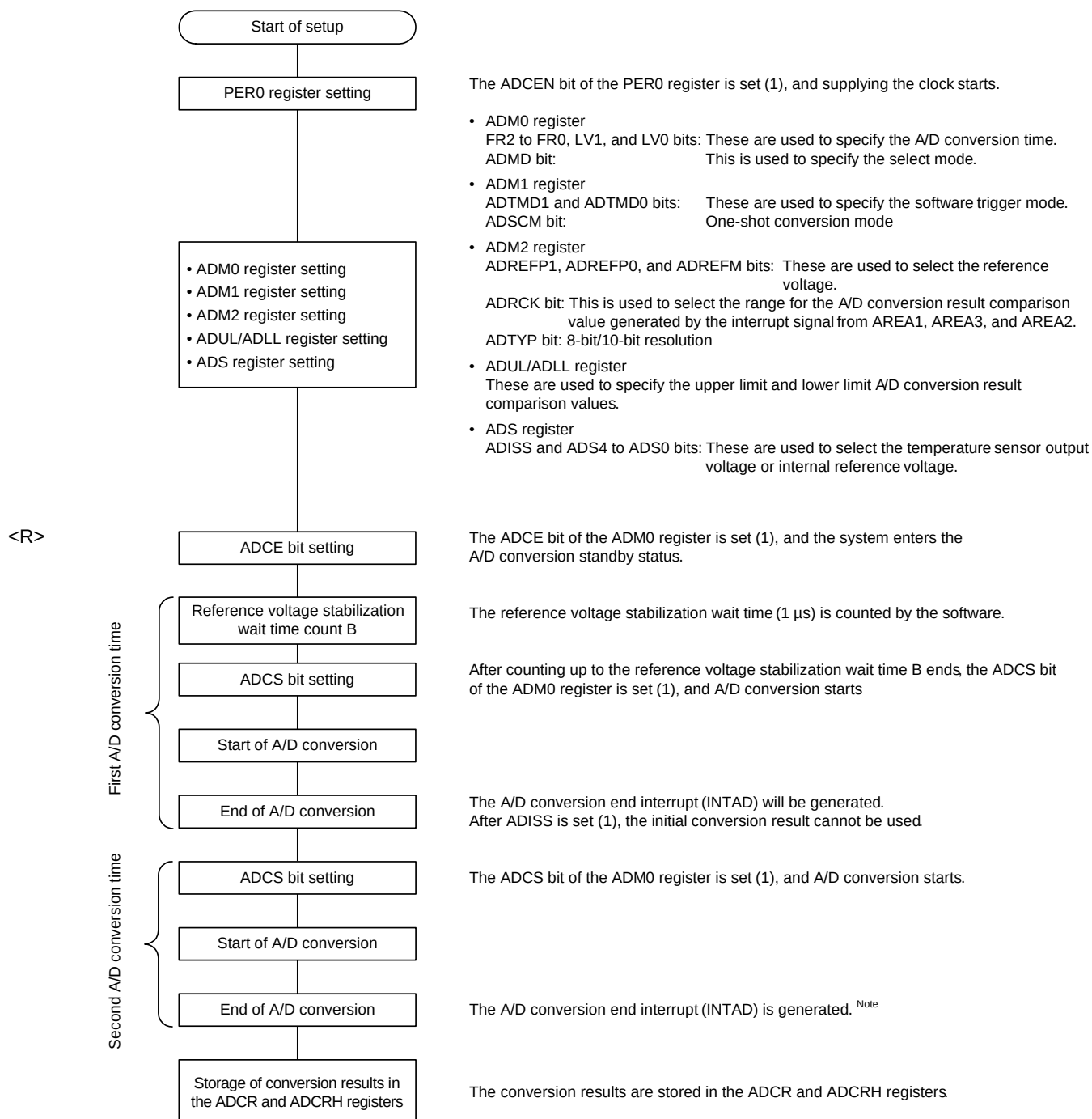
<R> Figure 13 - 34 Setup when temperature sensor output voltage/internal reference voltage is selected
