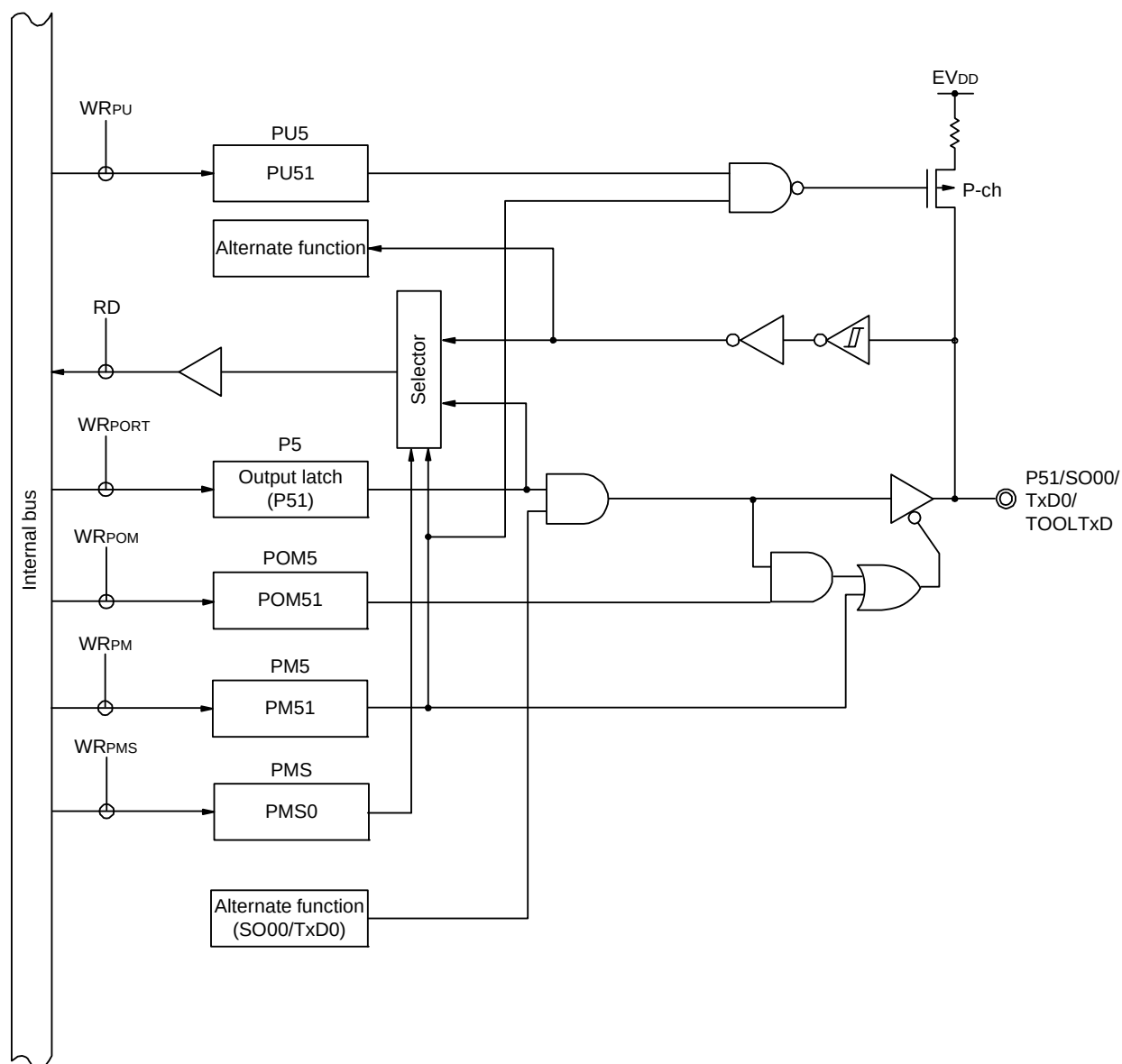
Figure 4 - 24 Block Diagram of P51
