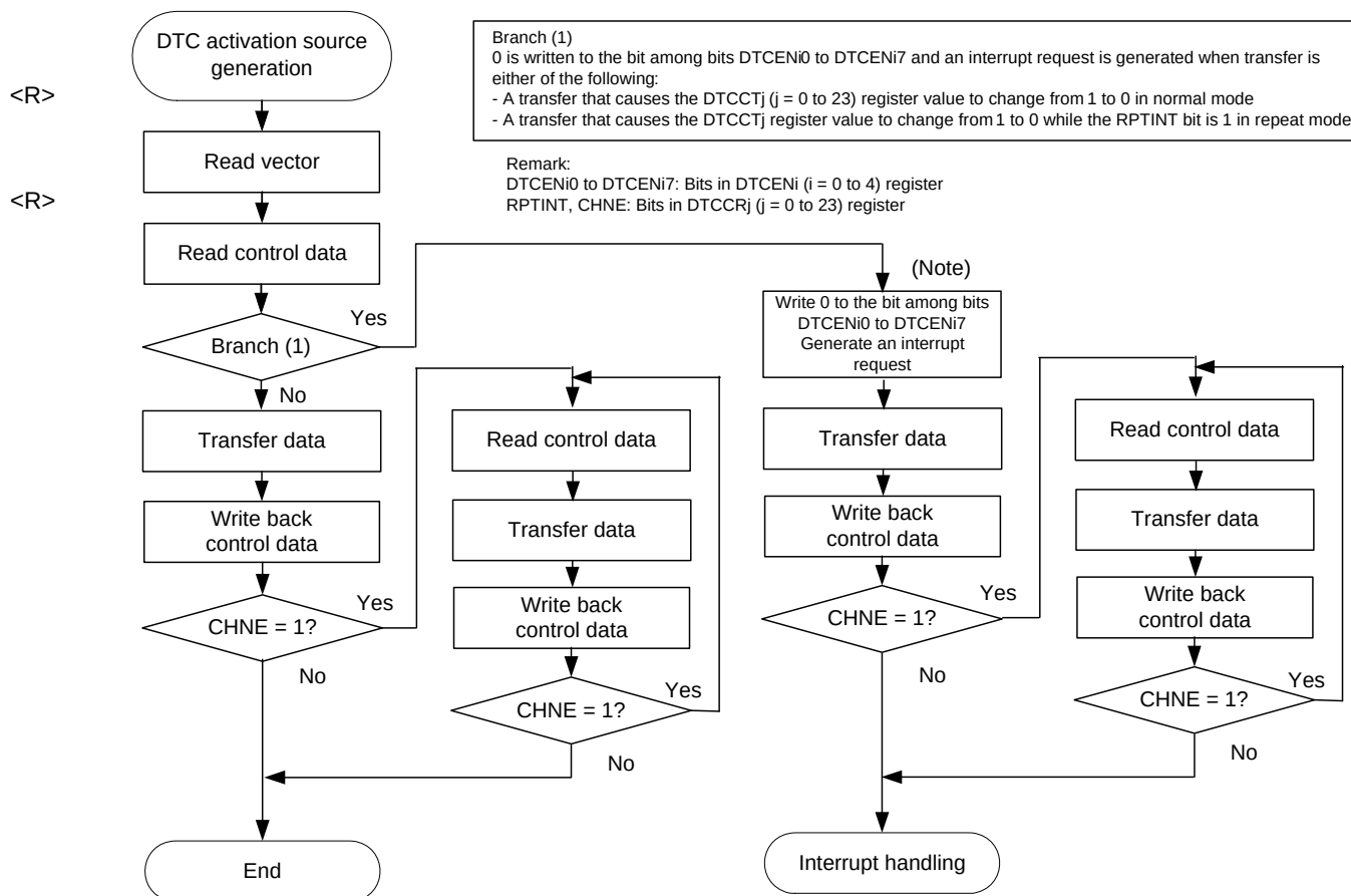
Figure 16 - 13 DTC Internal Operation Flowchart
