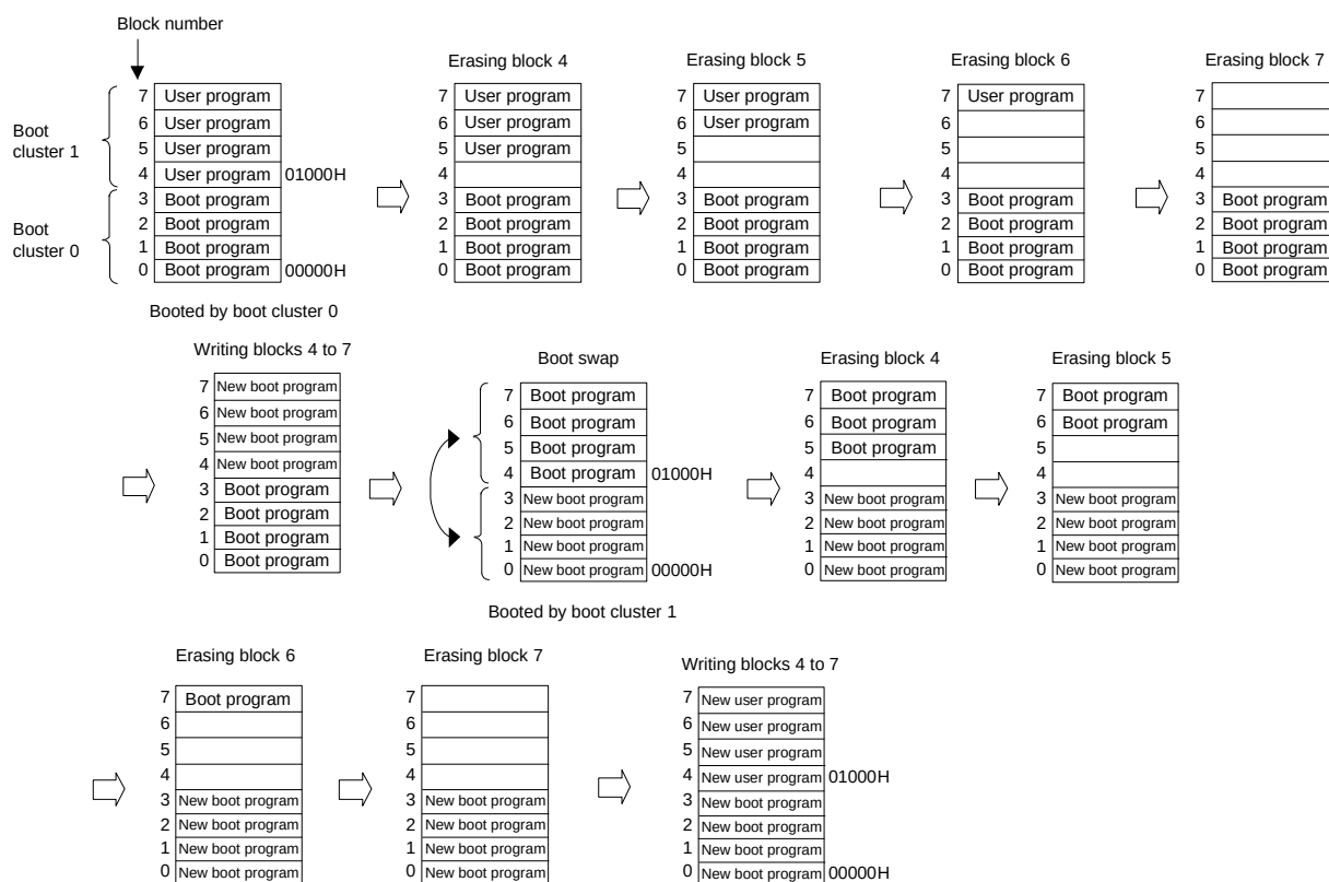
Figure 27 - 10 Example of Executing Boot Swapping
