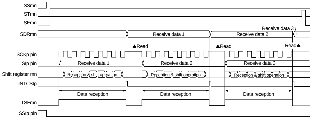
Figure 14 - 95 Timing Chart of Slave Reception (in Single-Reception Mode) (Type 1: DAPmn = 0, CKPmn = 0)
