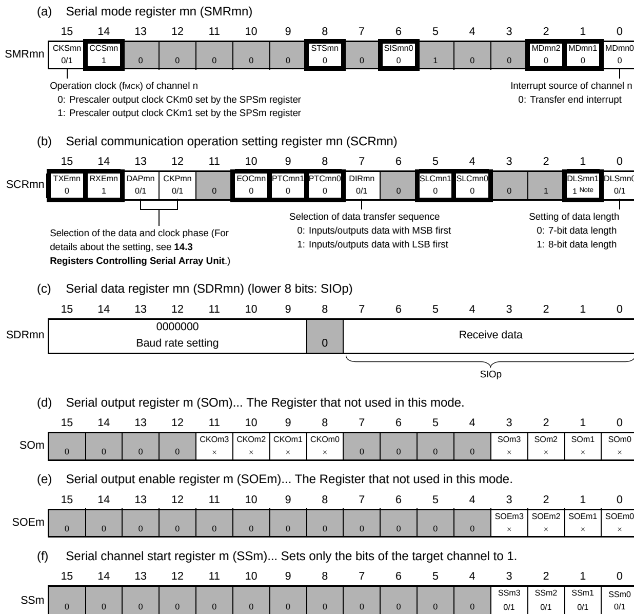
Figure 14 - 60 Example of Contents of Registers for Slave Reception of 3-Wire Serial I/O (CSI00, CSI01, CSI10, CSI11, CSI20, CSI21)
