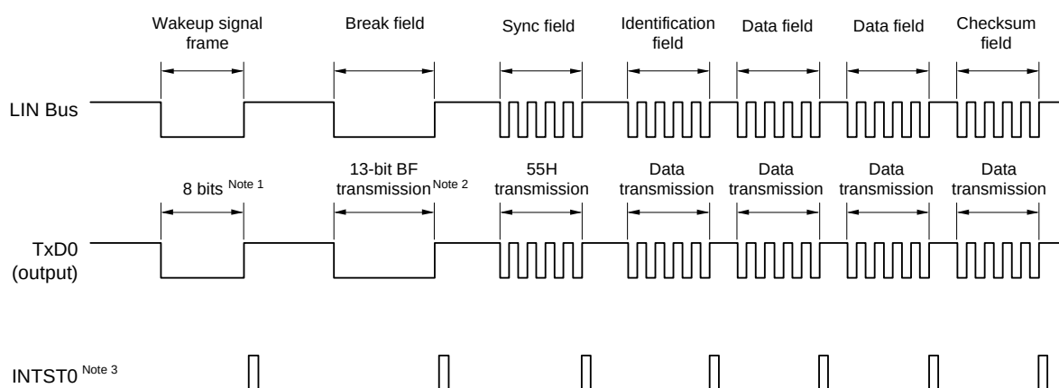
Figure 14 - 131 Transmission Operation of LIN
