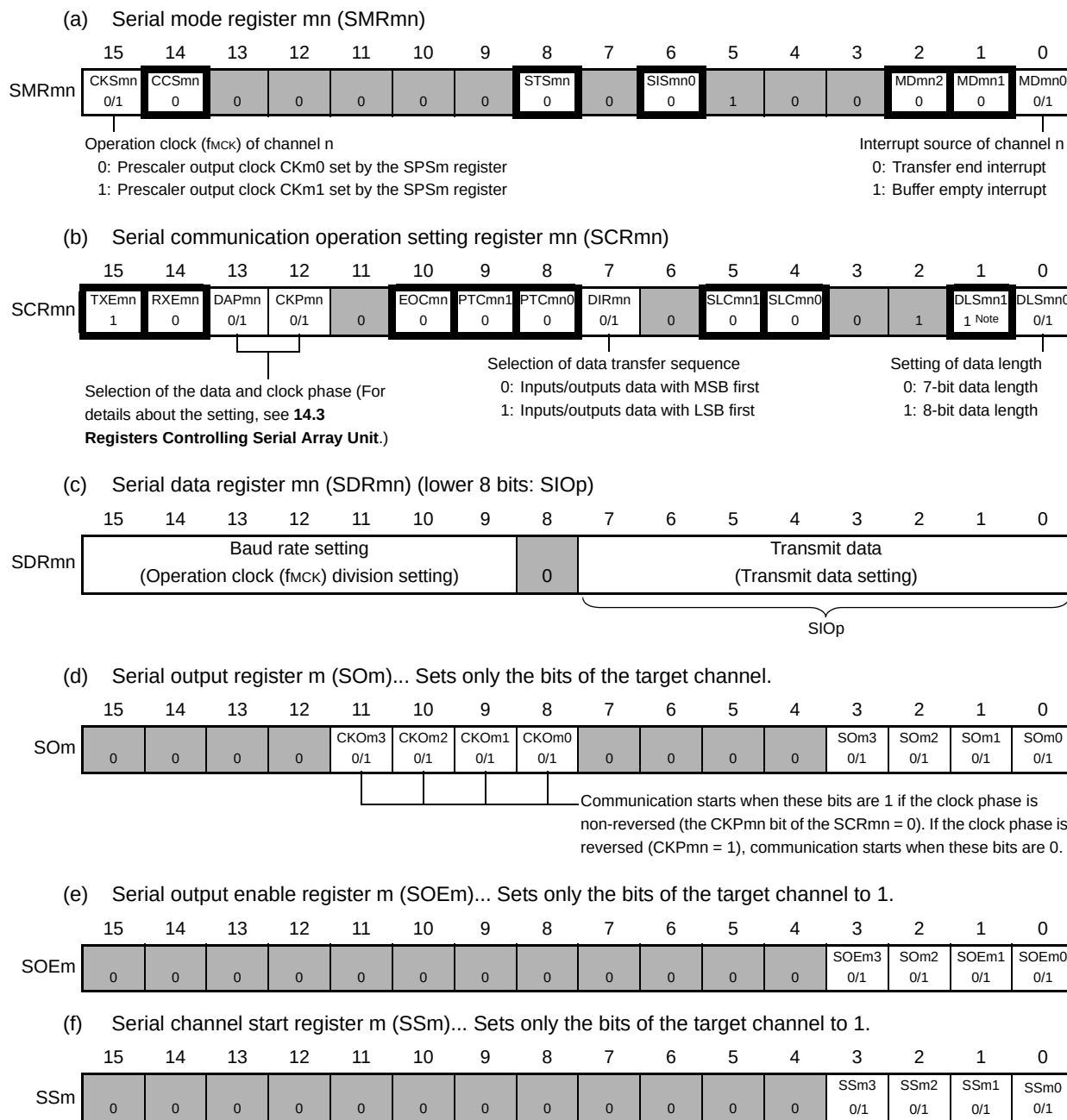
Figure 14 - 28 Example of Contents of Registers for Master Transmission of 3-Wire Serial I/O (CSI00, CSI01, CSI10, CSI11, CSI20, CSI21)
