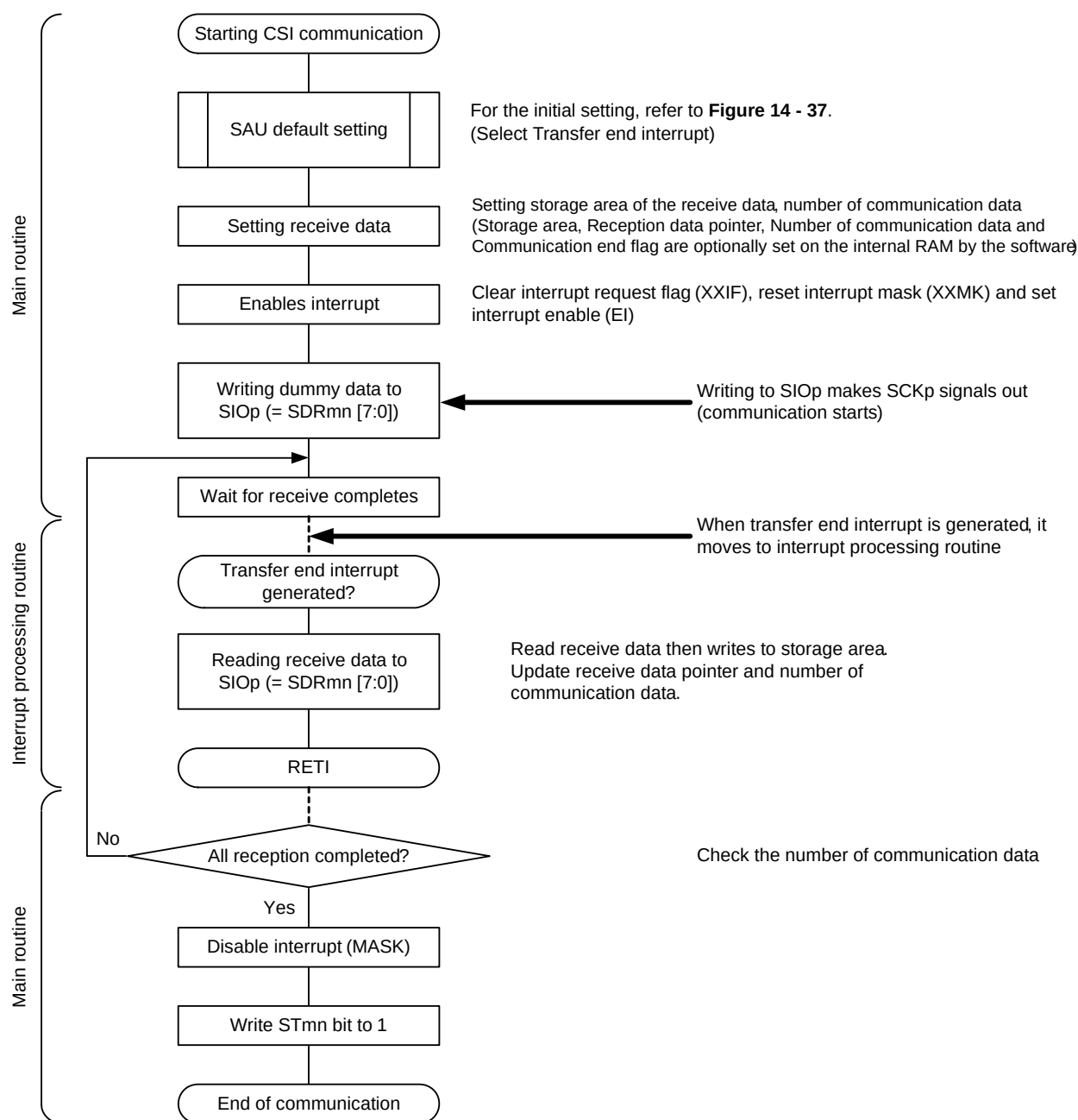
Figure 14 - 41 Flowchart of Master Reception (in Single-Reception Mode)
