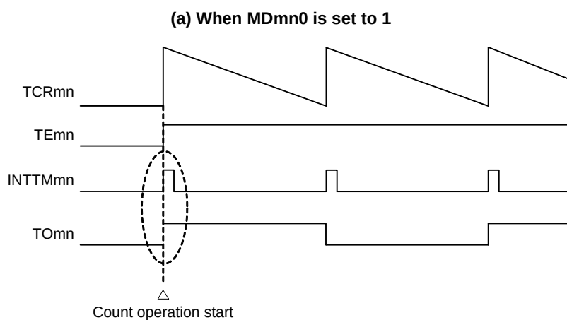
Figure 6 - 42 Operation examples of timer interrupt at count operation start and TOMn output
