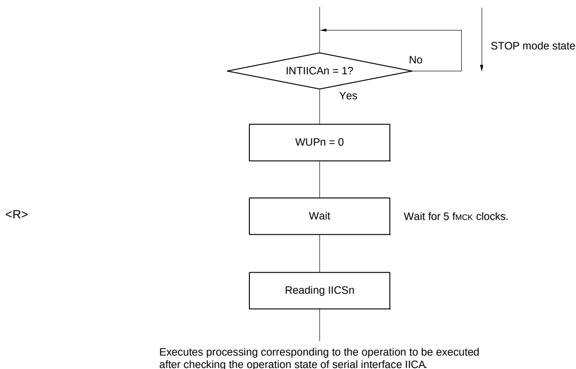
Figure 15 - 30 Flow When Setting WUPn = 0 upon Address Match (Including Extension Code Reception)
