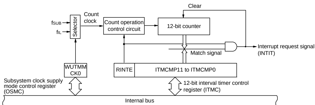
Figure 10 - 1 Block Diagram of 12-bit Interval Timer
