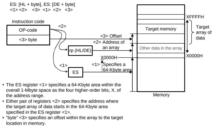
Figure 3 - 27 Example of ES:[HL + byte], ES:[DE + byte]
