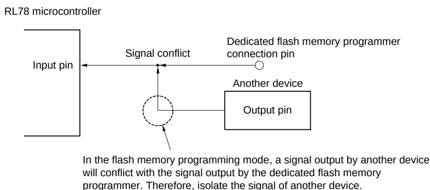
Figure 27 - 5 Signal Conflict ( RESET Pin)
