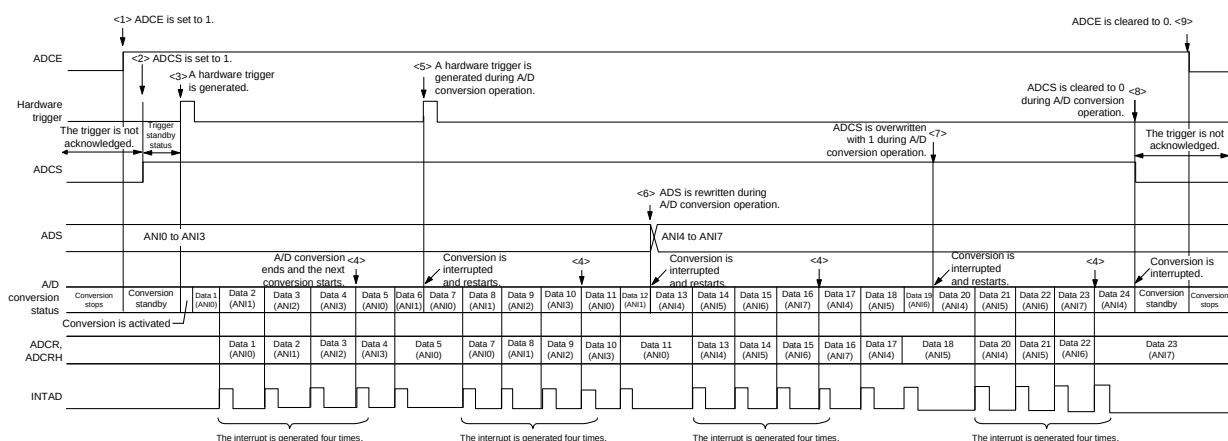
Figure 13 - 25 Example of Hardware Trigger No-Wait Mode (Scan Mode, Sequential Conversion Mode) Operation
