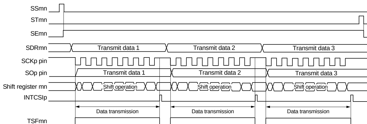
Figure 14 - 32 Timing Chart of Master Transmission (in Single-Transmission Mode)
