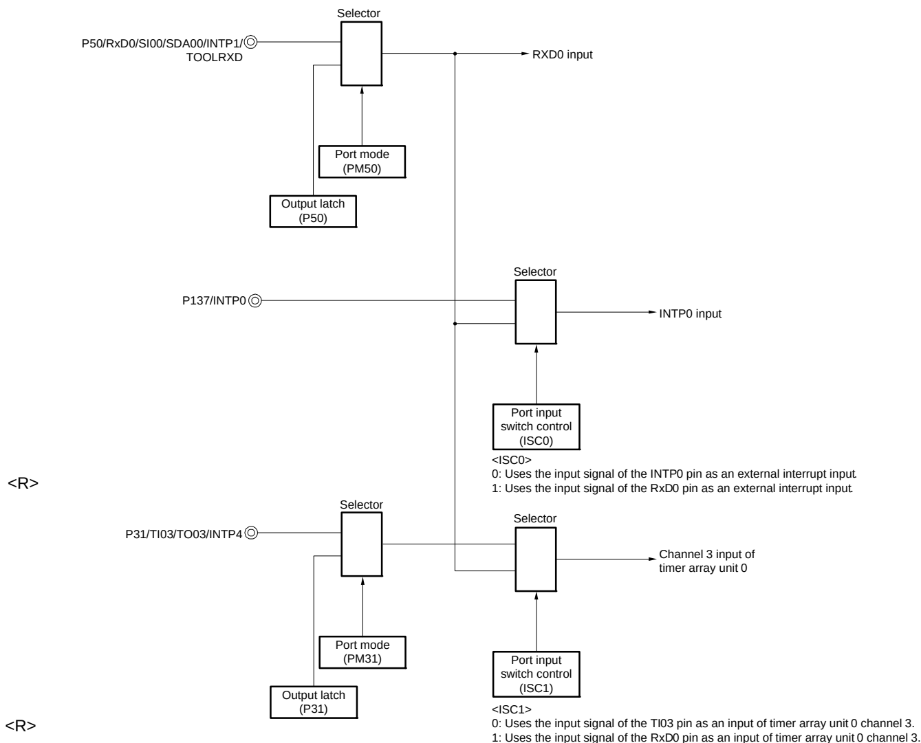
Figure 14 - 135 Port Configuration for Manipulating Reception of LIN
