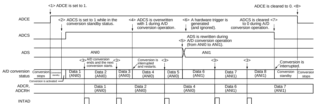
<R> Figure 13 - 19 Example of Software Trigger Mode (Select Mode, Sequential Conversion Mode) Operation Timing
