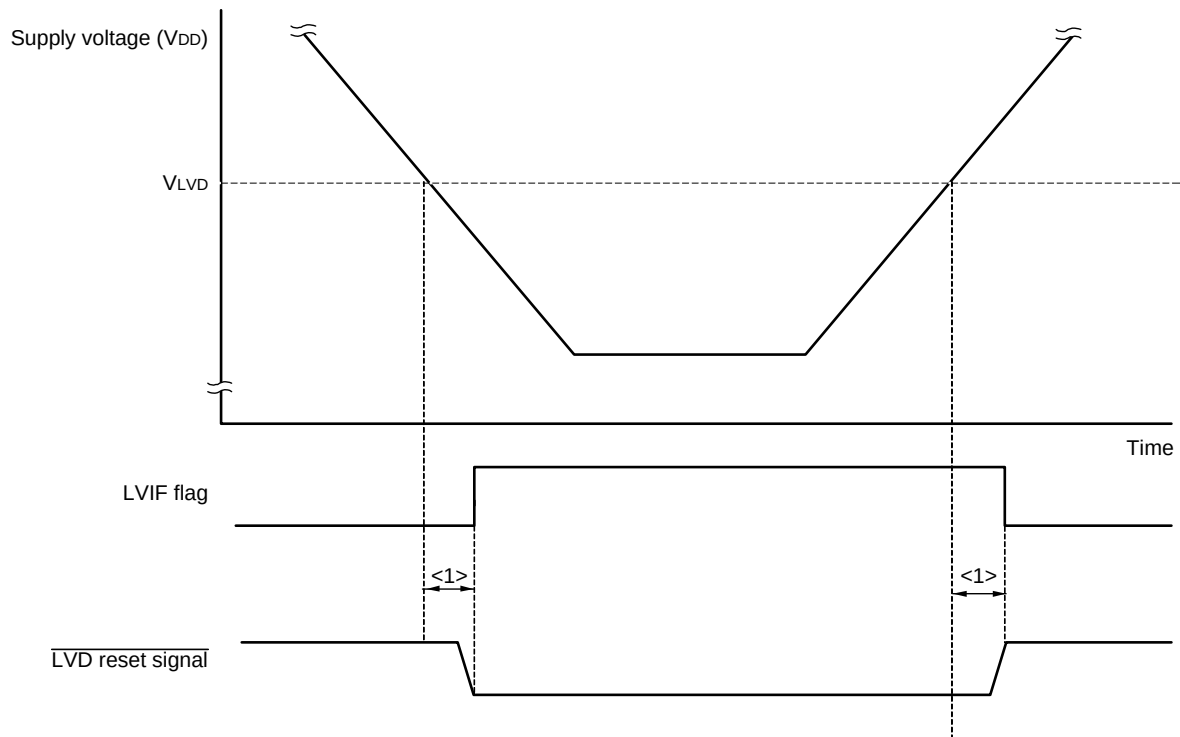
Figure 23 - 10 Delay from the time LVD reset source is generated until the time LVD reset has been generated or released
