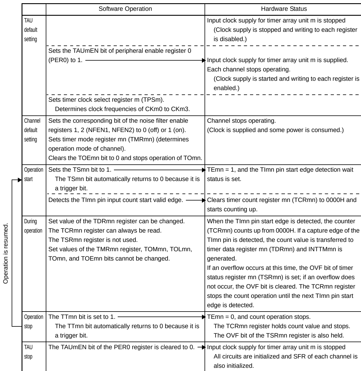
Figure 6 - 65 Operation Procedure When Input Signal High-/Low-Level Width Measurement Function Is Used
