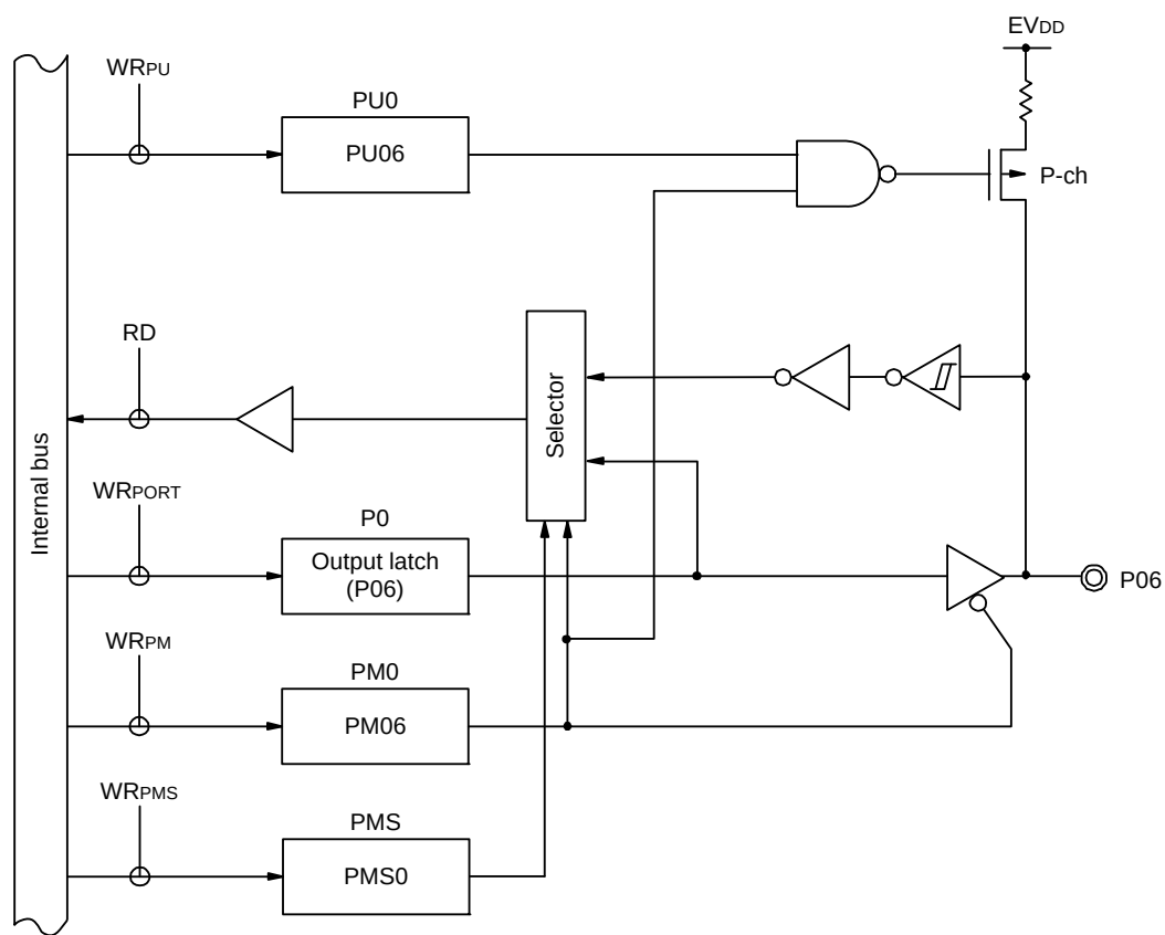
Figure 4 - 7 Block Diagram of P06
