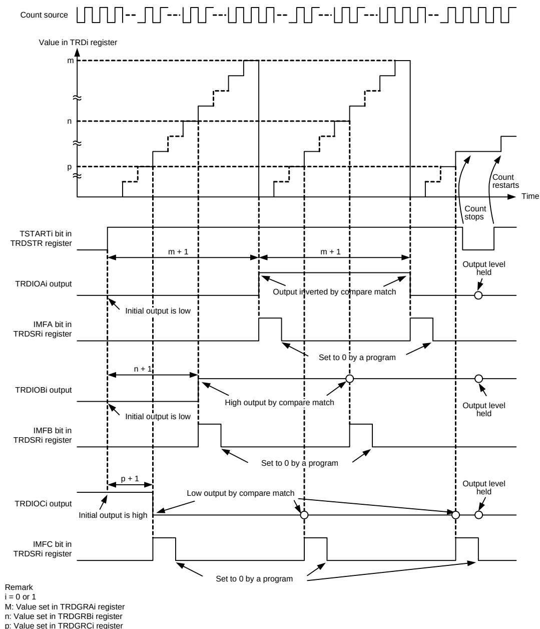
Figure 8 - 50 Operation Example of Output Compare Function
