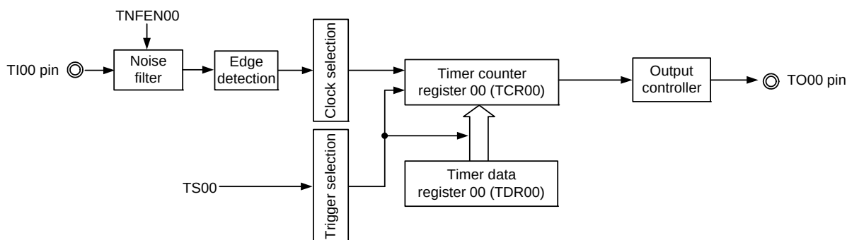
Figure 6 - 54 Block Diagram of Operation as Frequency Divider
