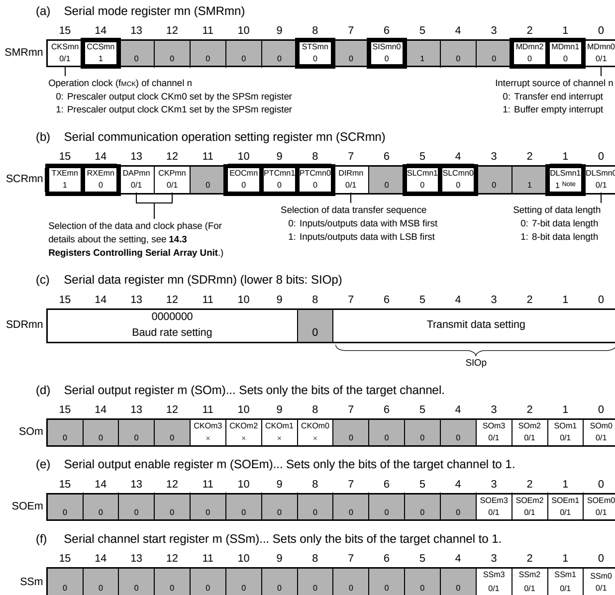
Figure 14 - 52 Example of Contents of Registers for Slave Transmission of 3-Wire Serial I/O (CSI00, CSI01, CSI10, CSI11, CSI20, CSI21)
