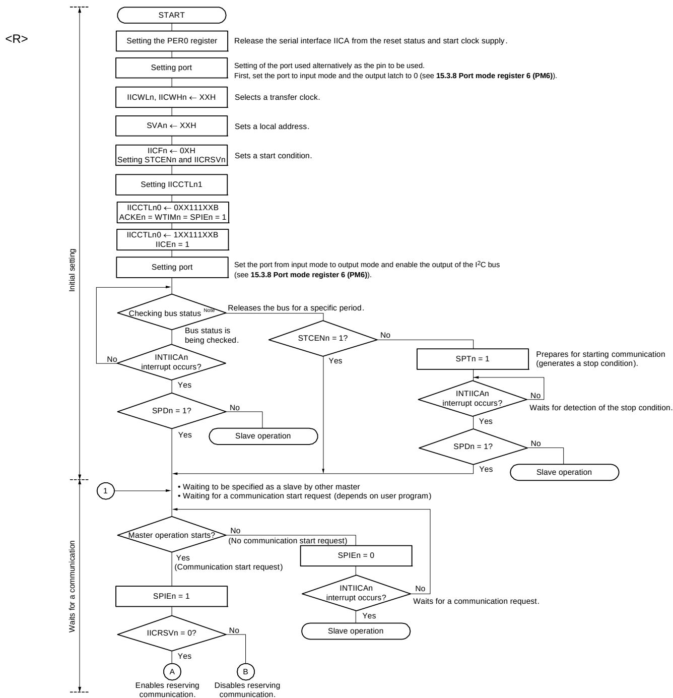
Figure 15 - 36 Master Operation in Multi-Master System (1/3)
