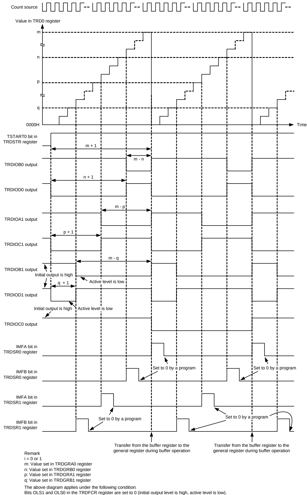
Figure 8 - 57 Operation Example in Reset Synchronous PWM Mode
