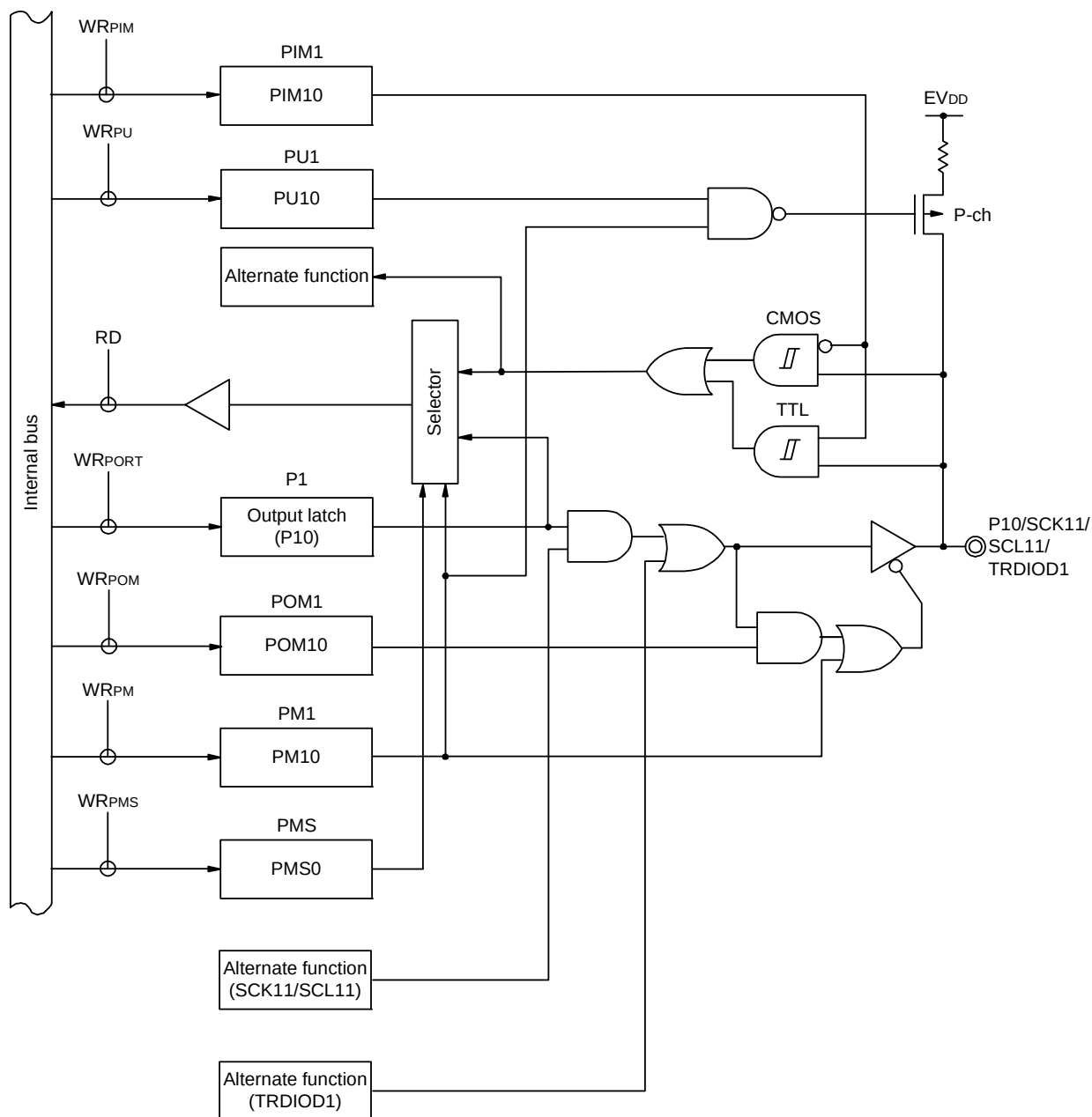
Figure 4 - 8 Block Diagram of P10
