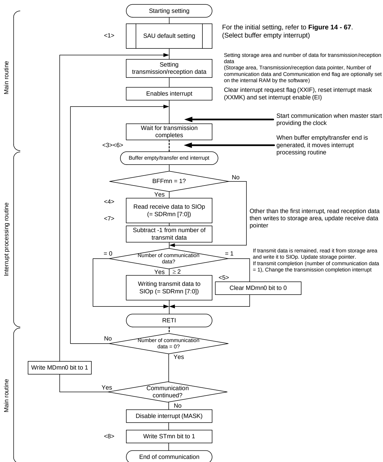
<R> Figure 14 - 73 Flowchart of Slave Transmission/Reception (in Continuous Transmission/Reception Mode)
