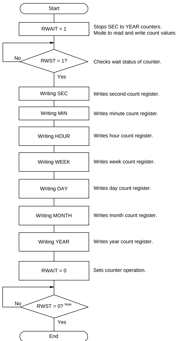
Figure 9 - 23 Procedure for Writing Real-time Clock
