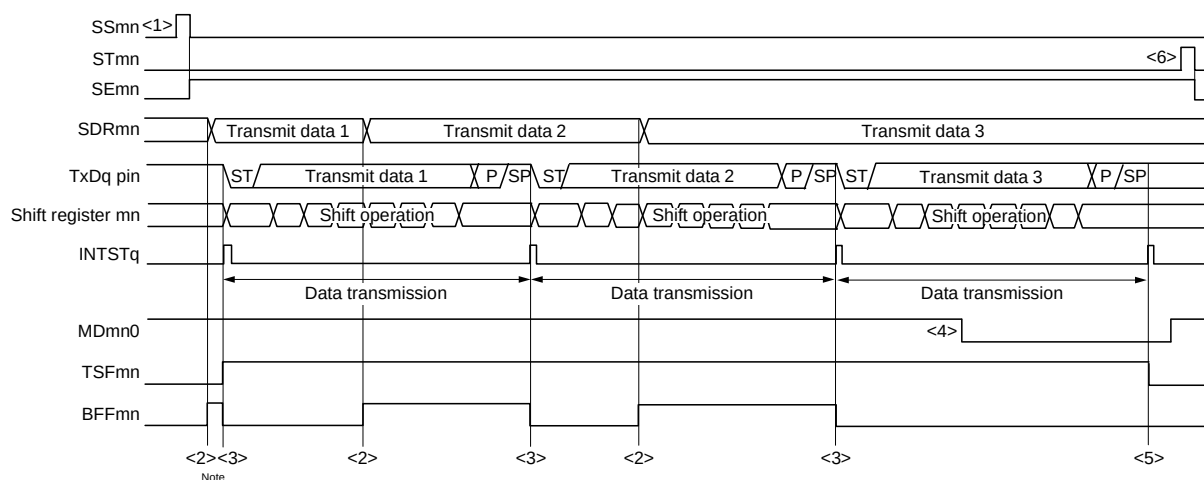
Figure 14 - 114 Timing Chart of UART Transmission (in Continuous Transmission Mode)
