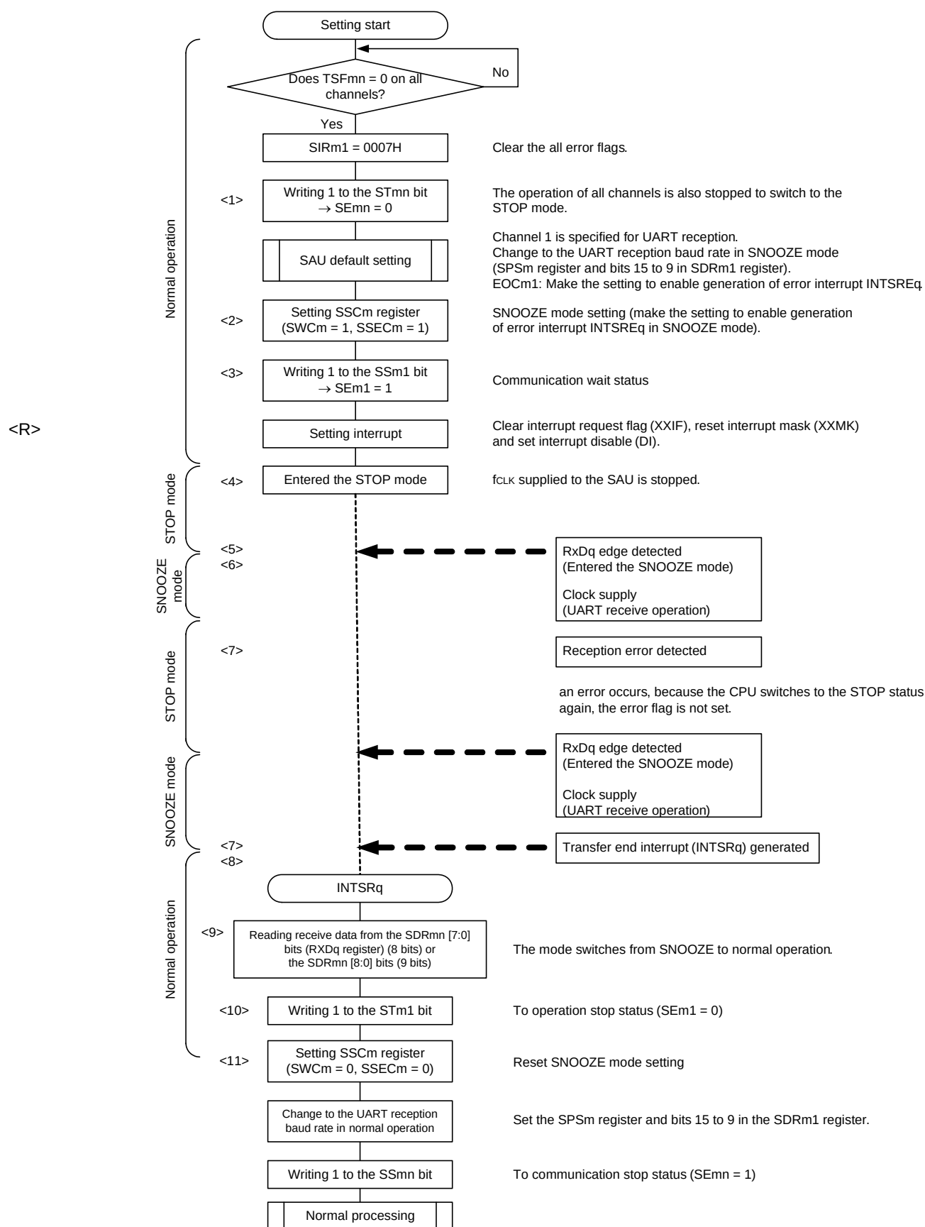
Figure 14 - 127 Flowchart of SNOOZE Mode Operation (EOCm1 = 1, SSECm = 1)
