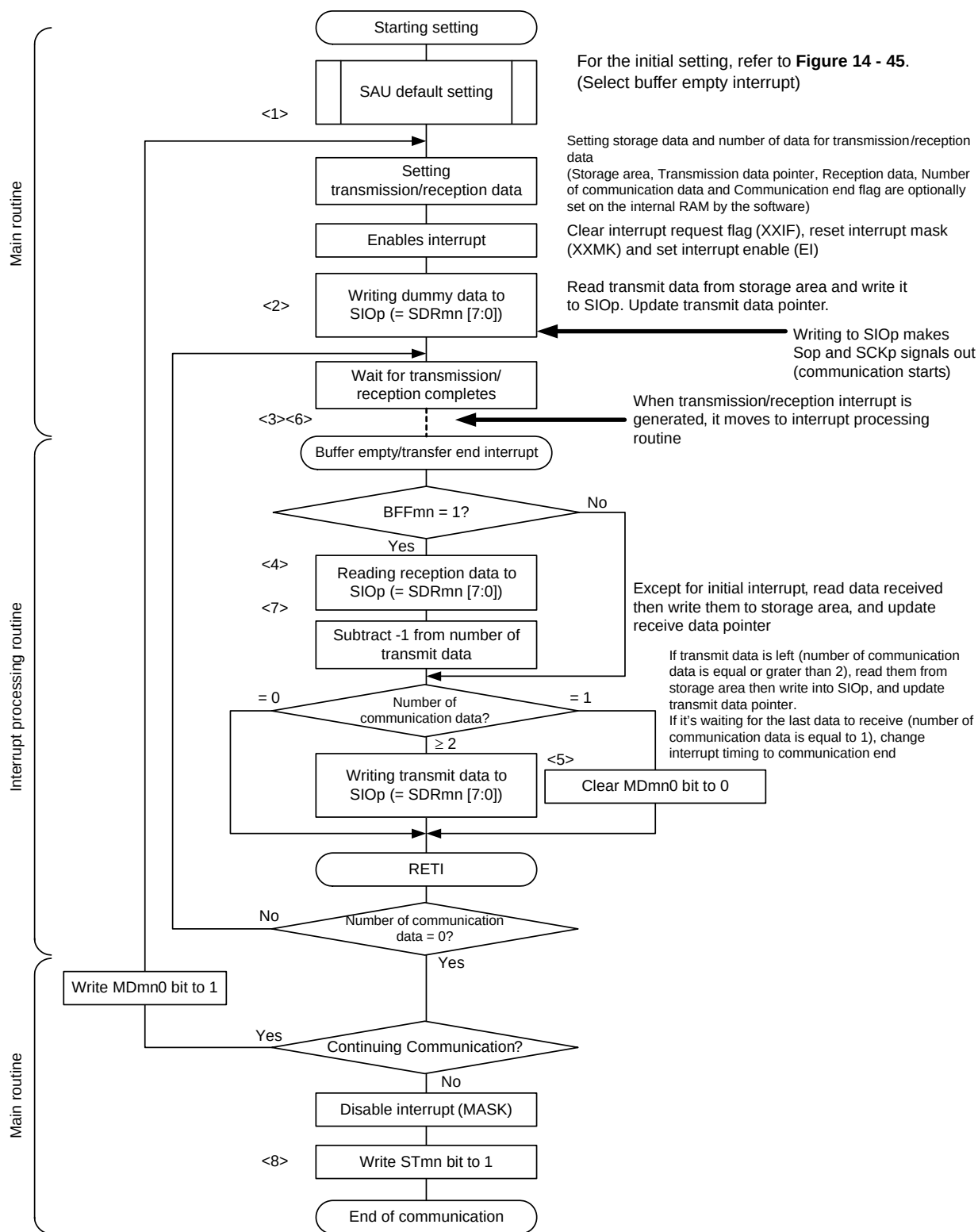
Figure 14 - 51 Flowchart of Master Transmission/Reception (in Continuous Transmission/Reception Mode)
