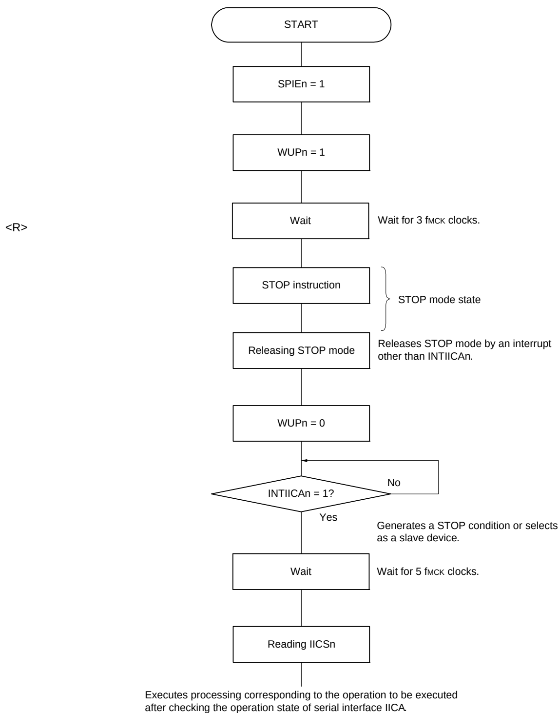
Figure 15 - 31 When Operating as Master Device after Releasing STOP Mode other than by INTIICAn
