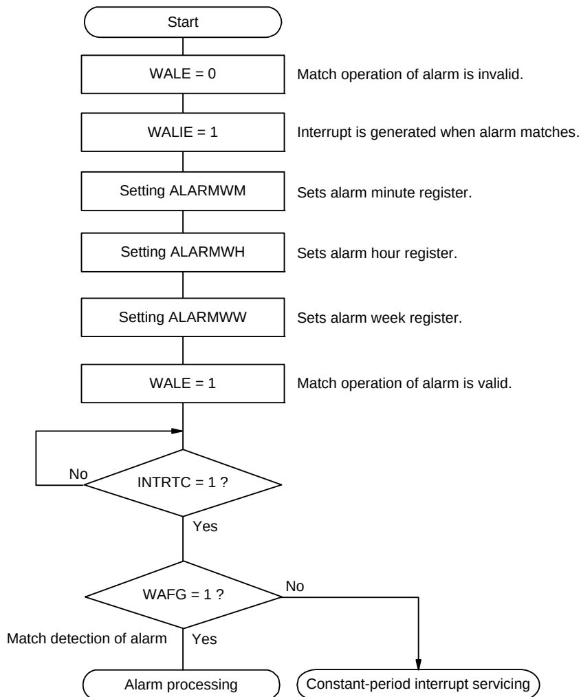
Figure 9 - 24 Alarm Setting Procedure
