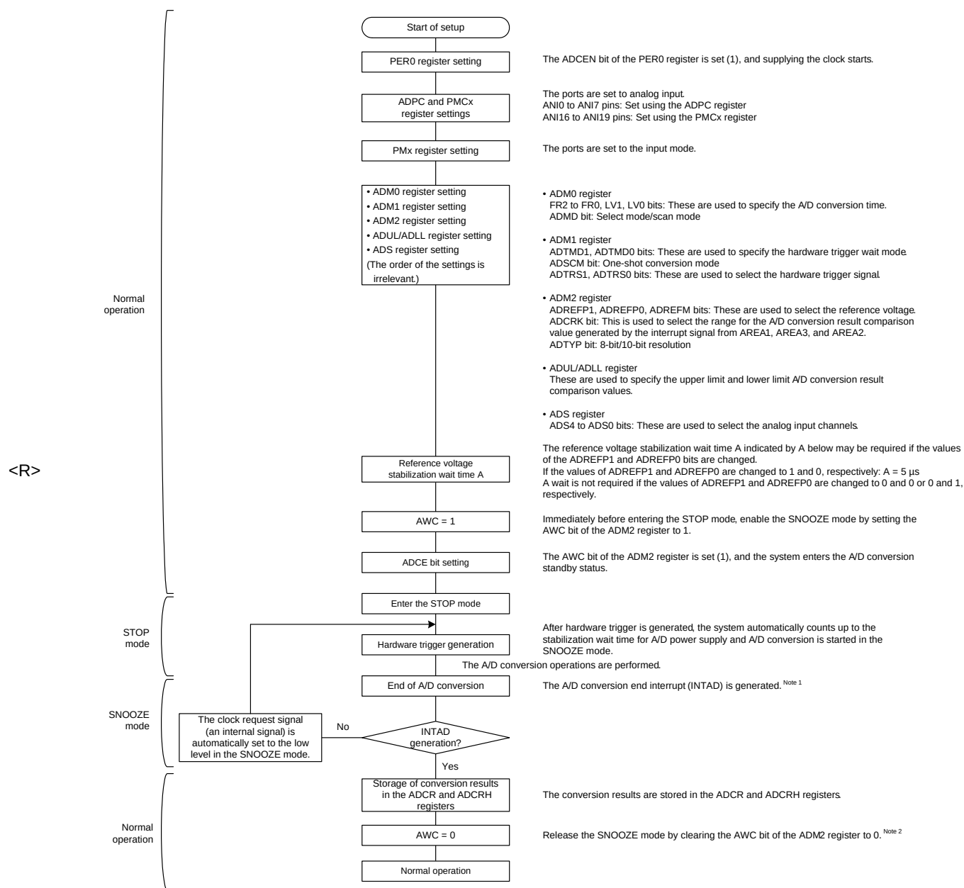
Figure 13 - 39 Flowchart for Setting up SNOOZE Mode
