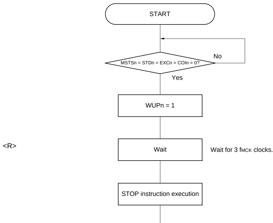
Figure 15 - 29 Flow When Setting WUPn = 1
