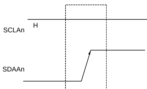
Figure 15 - 25 Stop Condition
