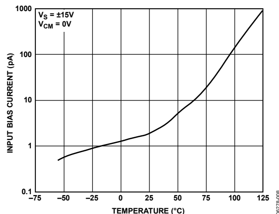
Figure 8. AD8682 Input Bias Current vs. Temperature
