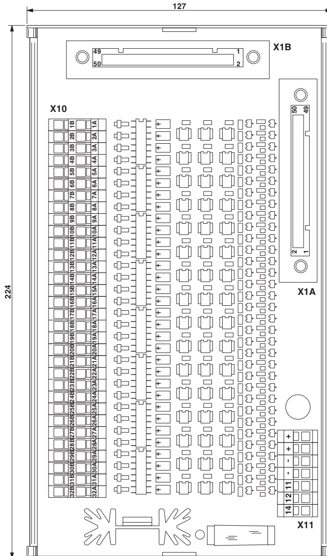
Dimensioned drawing
