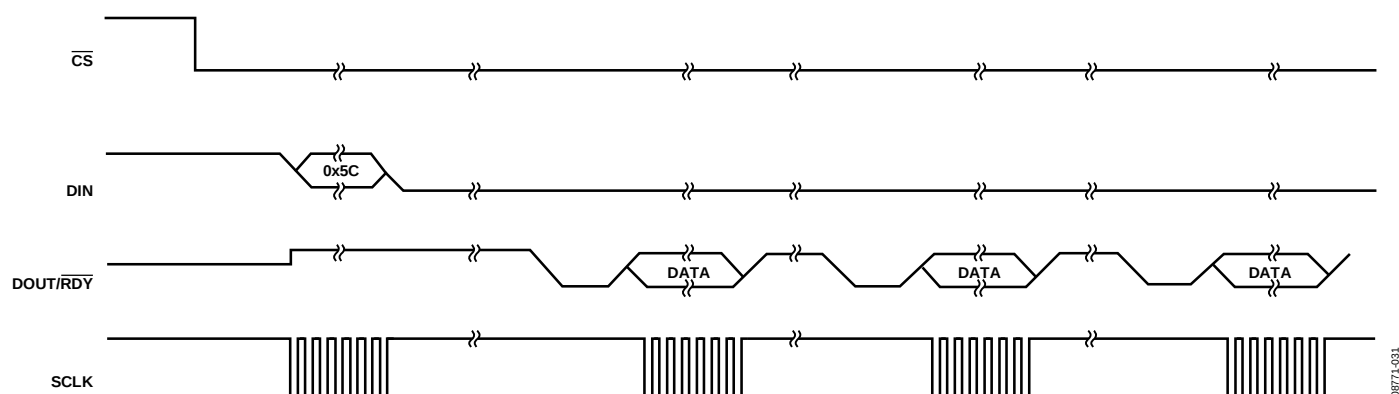
Figure 23. Continuous Read
