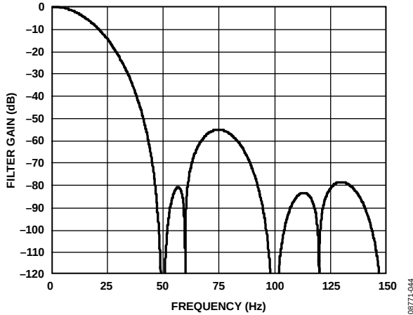
Figure 31. Sinc 4 Filter Response (FS[9:0] = 96, REJ60 = 1)
