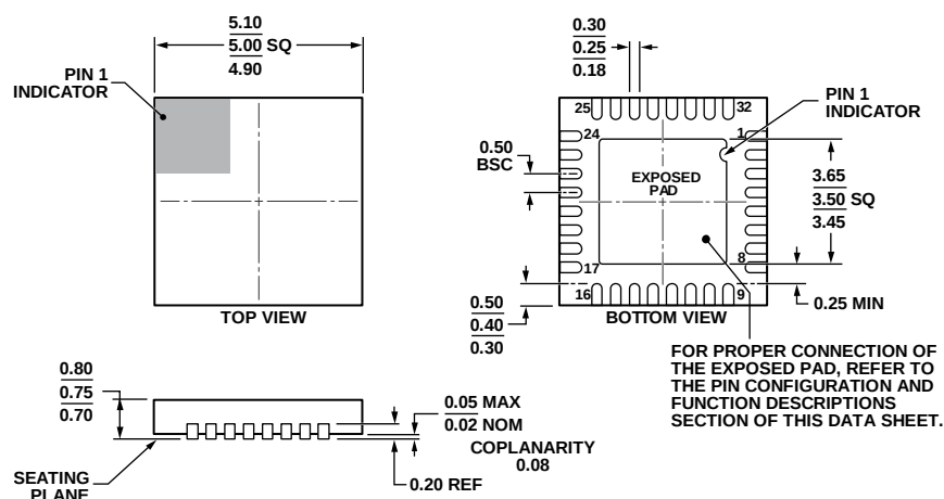
Figure 51. 32-Lead Lead Frame Chip Scale Package [LFCSP-WQ] 5 mm × 5 mm Body, Very Very Thin Quad (CP-32-11)
