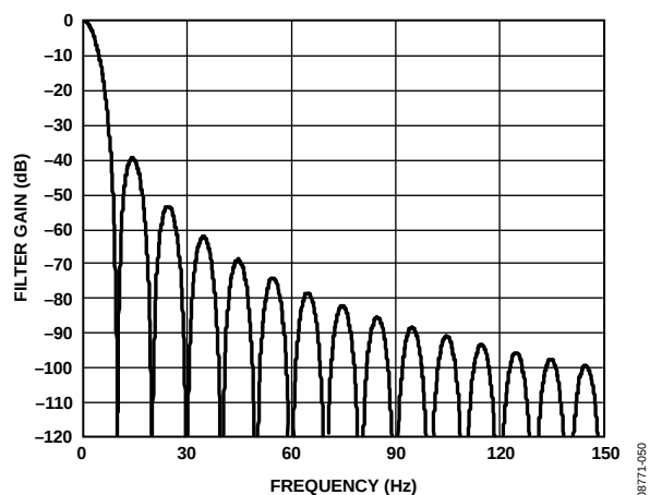
Figure 38. Sinc 3 Filter Response (FS[9:0] = 480)
