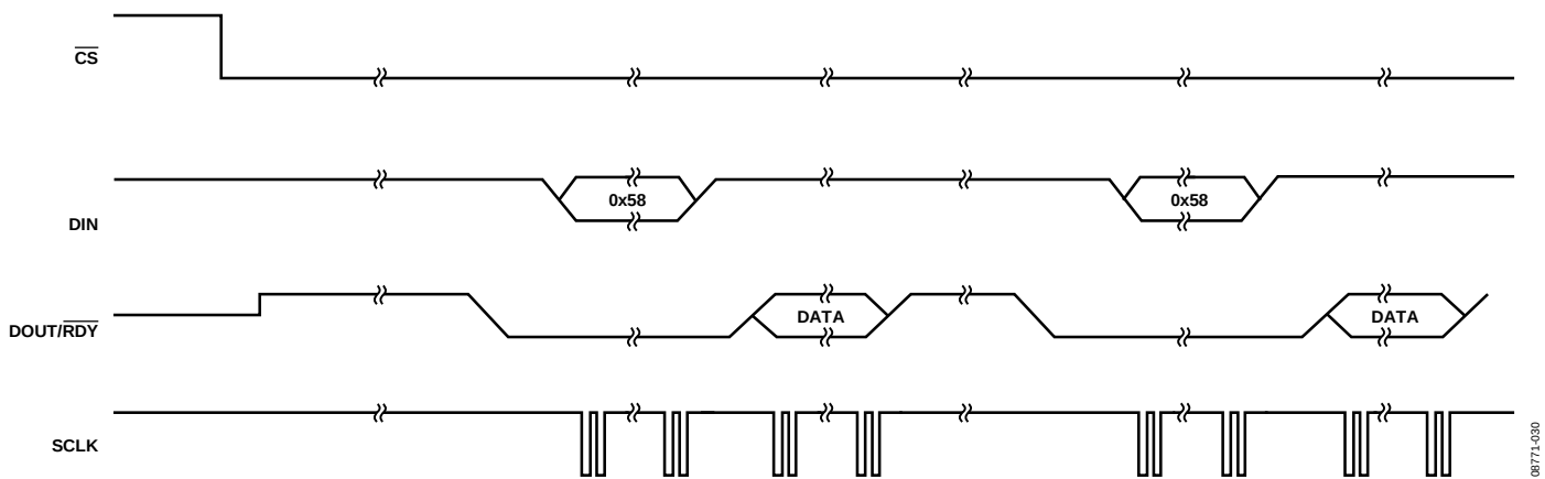
Figure 22. Continuous Conversion
