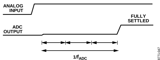
Figure 35. Sinc 3 Zero Latency Operation
