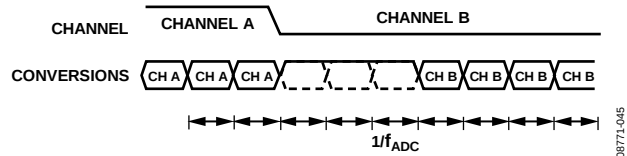
Figure 33. Sinc 3 Channel Change
