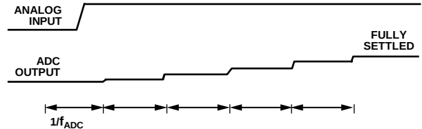
Figure 26. Asynchronous Step Change in Analog Input
