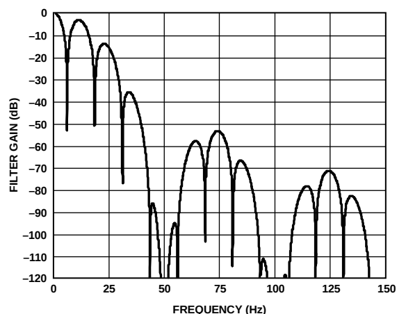
Figure 43. Sinc^4 Filter Response (FS[9:0] = 96, Chop Enabled)
