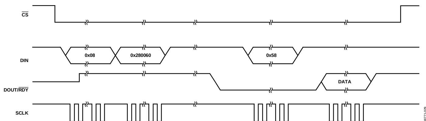
Figure 21. Single Conversion
