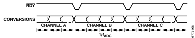
Figure 20. Channel Sequencer
