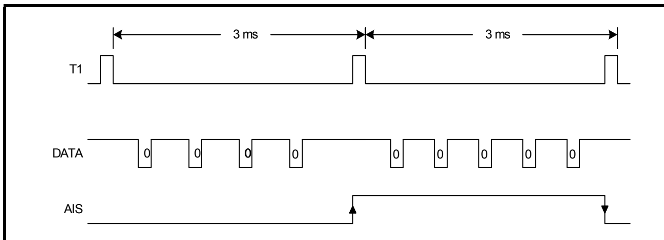
FIGURE 10. AIS DETECTION FOR T1 MODE
