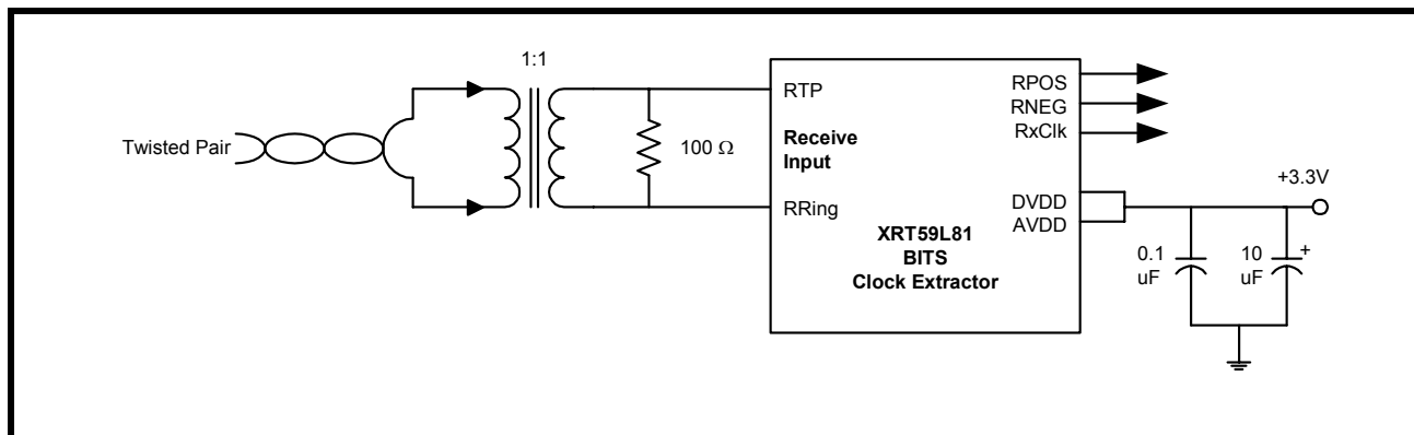
FIGURE 13. T1 APPLICATION FOR TWISTED PAIR INTERFACE
