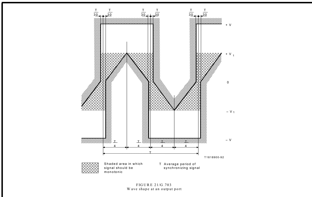
FIGURE 7. E1 CLOCK SIGNAL WAVE SHAPE - G.703
