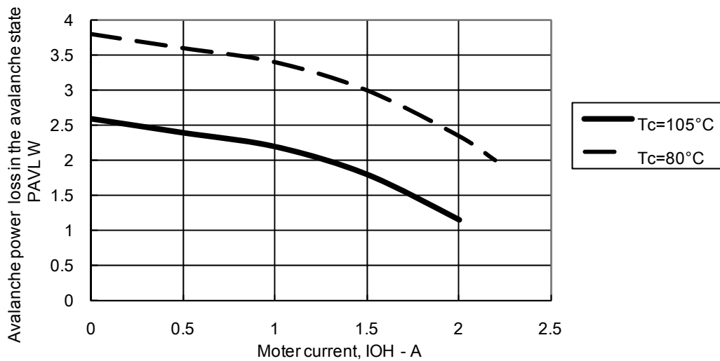
Figure 3 Allowable Loss Range, P_{AVL} - I_{OH} During STK672-430AN-E Avalanche Operations
