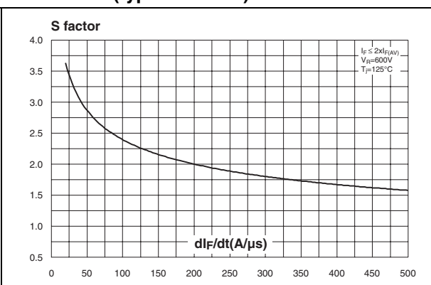
Figure 8. Softness factor versus dl_F/dt (typical values)
