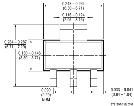
ST Package 3-Lead Plastic SOT-223 (LTC DWG # 05-08-1630)
