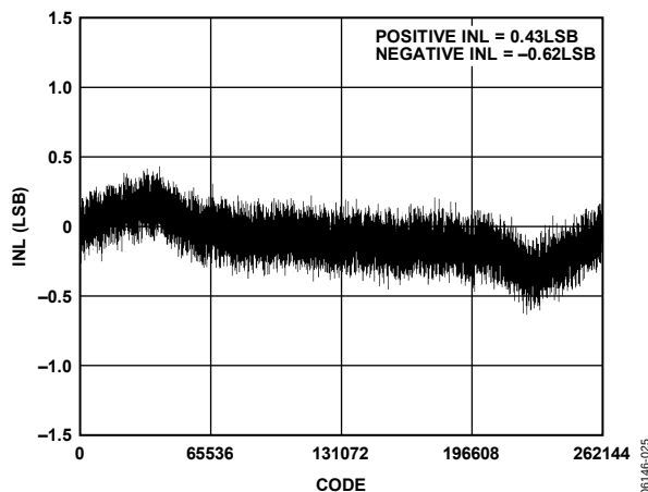
Figure 1. Integral Nonlinearity vs. Code, 5 V
