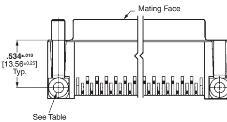
With Fixed Female Screwlock
