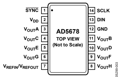
Figure 3. 14-Lead TSSOP (RU-14)
