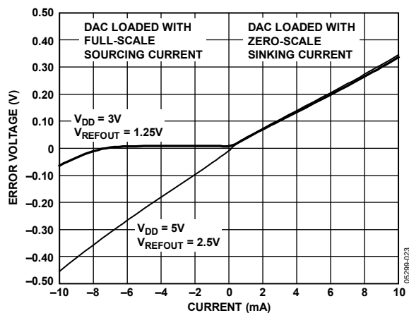
Figure 23. Headroom at Rails vs. Source and Sink
