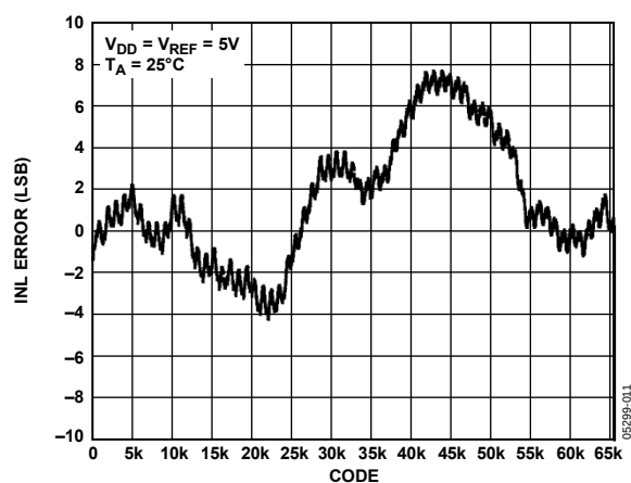
Figure 5. INL—16-Bit DAC
