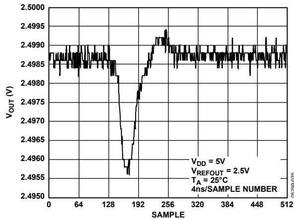
Figure 35. Analog Crosstalk
