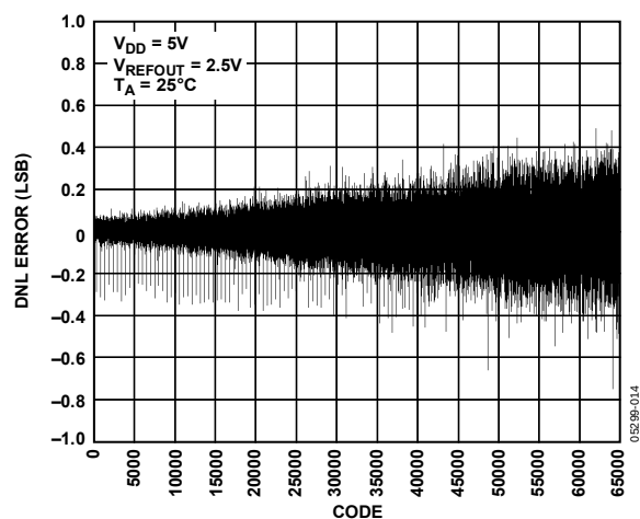
Figure 8. DNL 16-Bit DAC, 2.5 V Internal Reference
