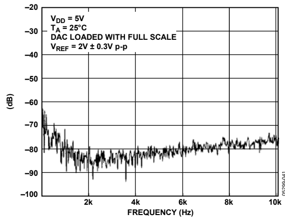
Figure 41. Total Harmonic Distortion
