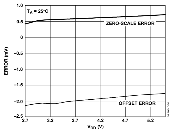
Figure 20. Zero-Scale Error and Offset Error vs. Supply Voltage
