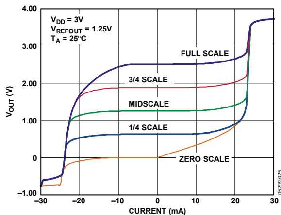
Figure 25. AD5678-1 Source and Sink Capability
