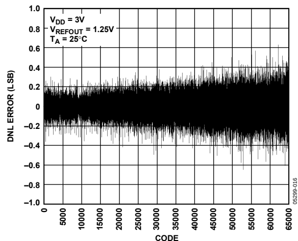
Figure 10. DNL—16-Bit DAC, 1.25 V Internal Reference
