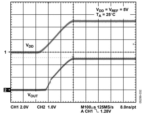
Figure 32. Power-On Reset to Midscale
