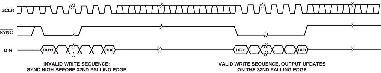
Figure 49. SYNC Interrupt Facility
