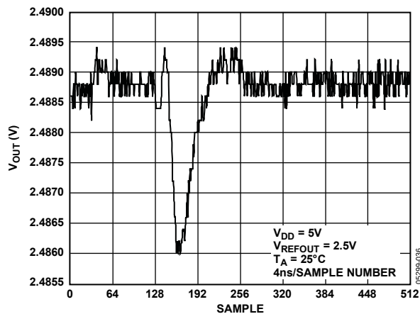
Figure 36. DAC-to-DAC Crosstalk
