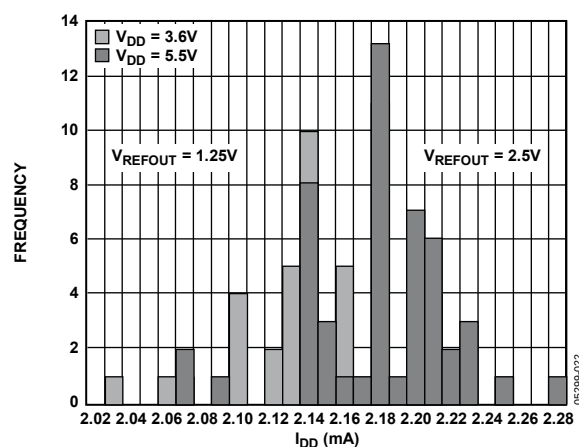
Figure 22. I_{DD} Histogram with Internal Reference
