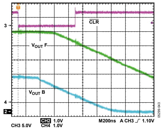
Figure 43. Hardware \overline{CLR}
