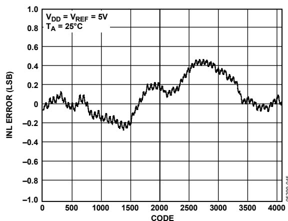
Figure 11. INL—12-Bit DAC
