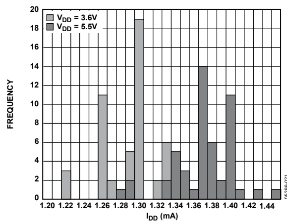
Figure 21. I_{DD} Histogram with External Reference
