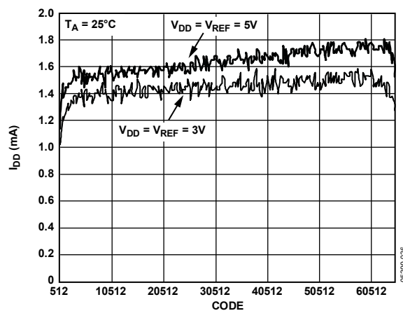
Figure 26. Supply Current vs. Code
