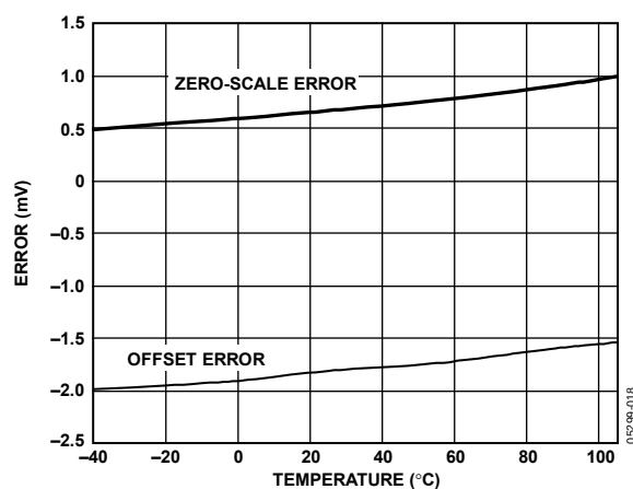
Figure 18. Zero-Scale Error and Offset Error vs. Temperature
