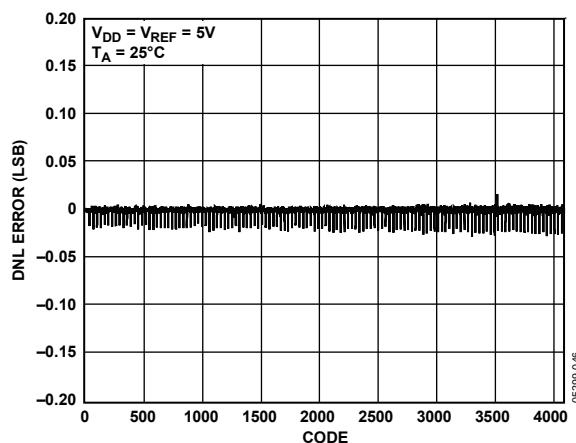
Figure 12. DNL—12-Bit DAC
