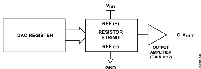
Figure 45. DAC Architecture
