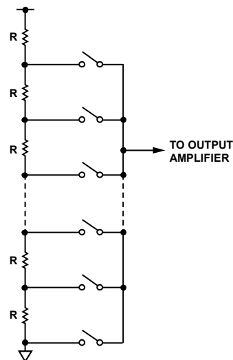
Figure 46. Resistor String
