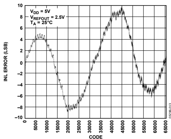
Figure 7. INL—16-Bit DAC, 2.5 V Internal Reference
