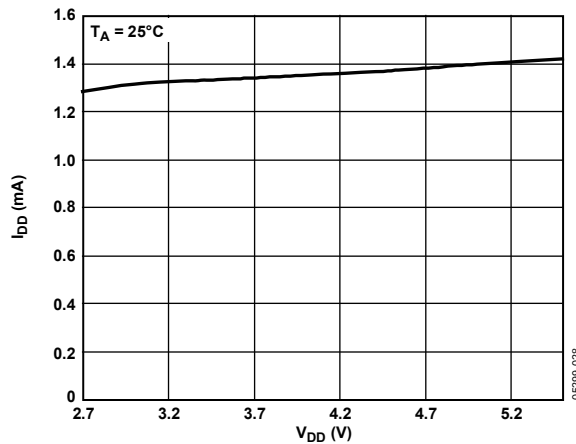
Figure 28. Supply Current vs. Supply Voltage
