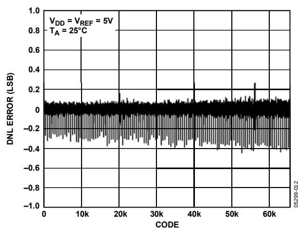
Figure 6. DNL—16-Bit DAC
