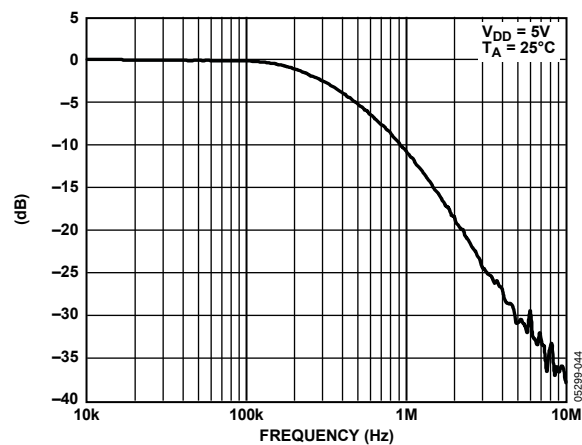
Figure 44. Multiplying Bandwidth
