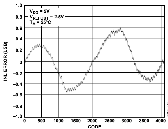
Figure 13. INL—12-Bit DAC, 2.5 V Internal Reference
