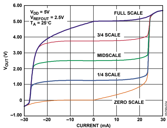
Figure 24. AD5678-2 Source and Sink Capability
