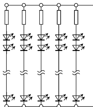
Circuit Example
