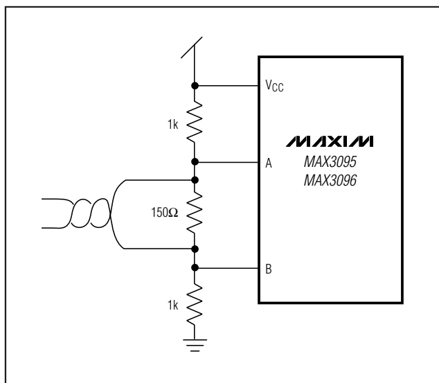
Figure 6. External Fail-Safe Implementation
