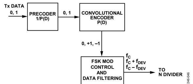
Figure 43. 3FSK Encoding
