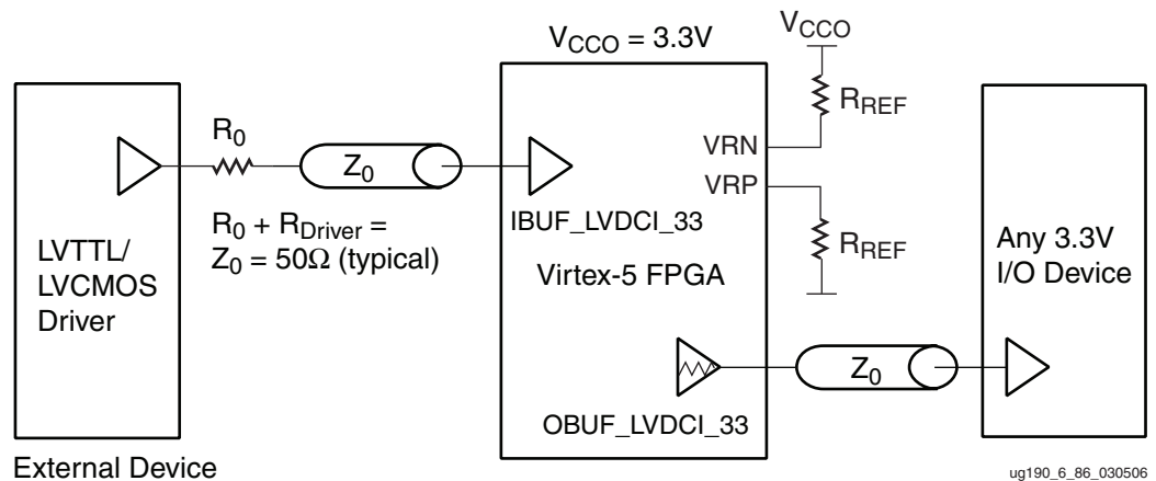
Figure 6-92: Connecting LVTTL or LVCMOS Using the LVDCI_33 Standard
