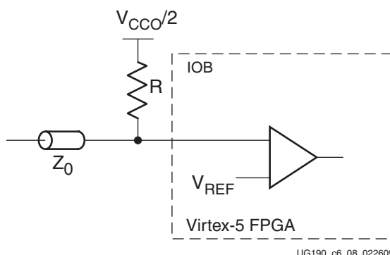
Figure 6-10: Input Termination to V_{CCQ}/2 without DCI
