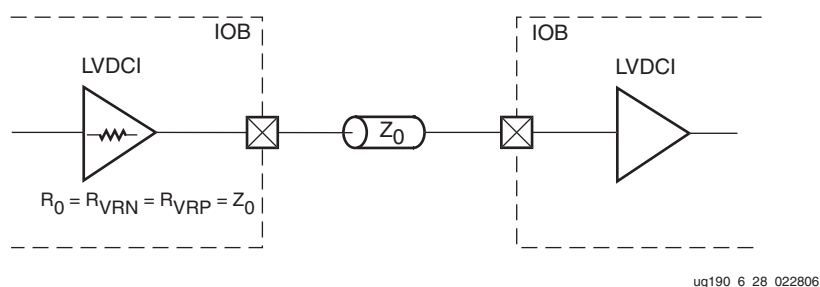
Figure 6-31: Controlled Impedance Driver with Unidirectional Termination
