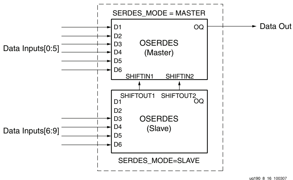
Figure 8-16: Block Diagram of OSERDES Width Expansion
