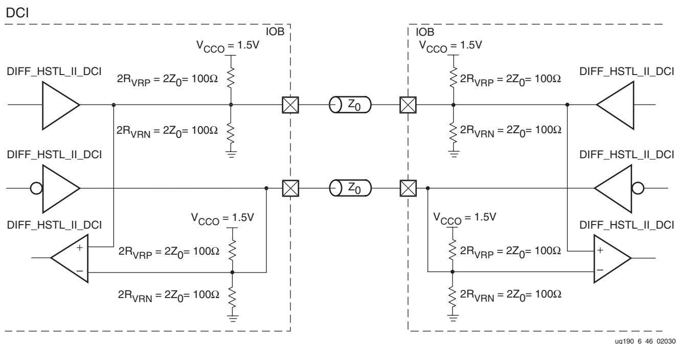
Figure 6-48: Differential HSTL (1.5V) Class II DCI Bidirectional Termination
