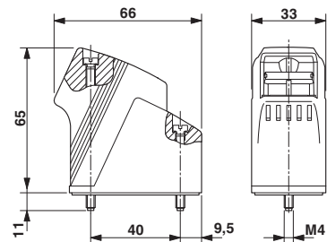
Dimensioned drawing
