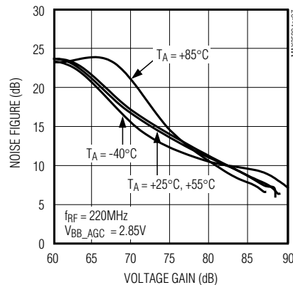
VHF MODE NOISE FIGURE vs. VOLTAGE GAIN
