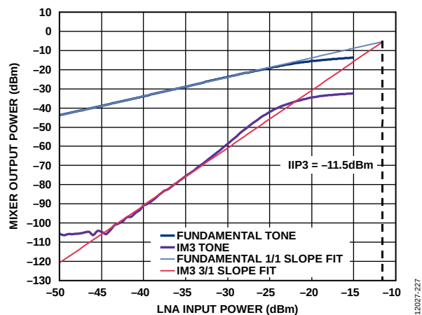
Figure 16. LNA/Mixer IIP3, V_{DD} = 3.0 V, Temperature = 25°C, RF Frequency = 915 MHz, LNA Gain = Low, Mixer Gain = Low, Source 1 Frequency = 915 MHz + 0.4 MHz, Source 2 Frequency = 915 MHz + 0.7 MHz
