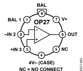
Figure 1. 8-Lead TO-99 (J-Suffix)
