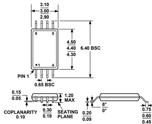
Figure 40. 8-Lead Thin Shrink Small Outline Package [TSSOP] (RU-8)
