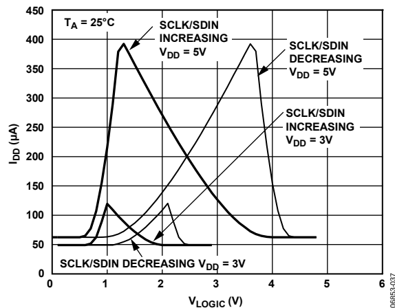
Figure 37. SCLK/SDIN vs. Logic Voltage
