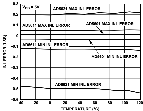
Figure 25. INL vs. Temperature (5 V)
