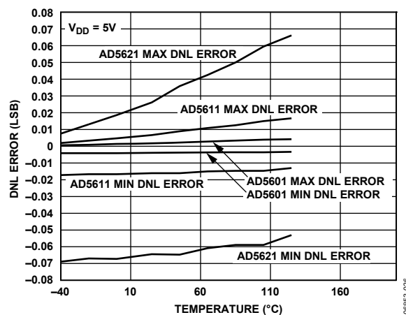
Figure 26. DNL vs. Temperature (5 V)
