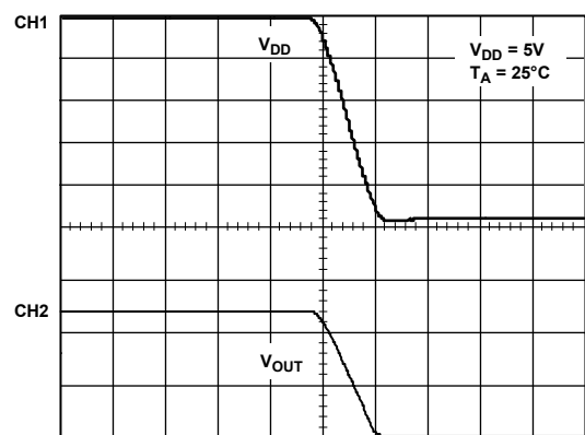
Figure 17. V_{DD} vs. V_{OUT}
