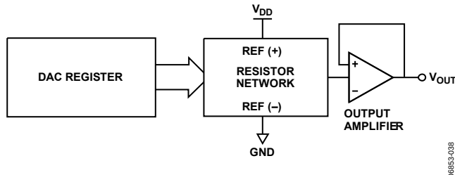
Figure 38. DAC Architecture
