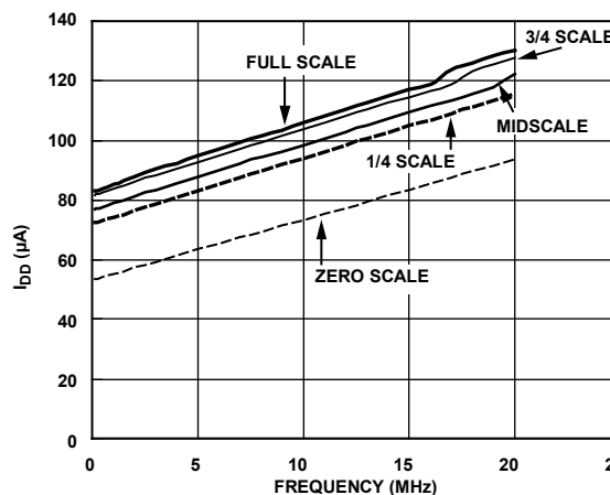
Figure 21. I_{DD} vs. SCLK vs. Code
