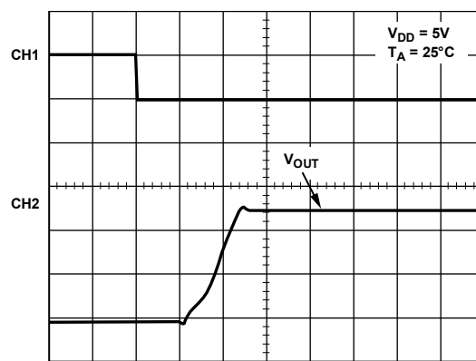
Figure 20. Exiting Power-Down Mode
