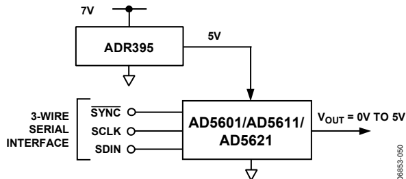
Figure 50. ADR395 as Power Supply to the AD5601/AD5611/AD5621
