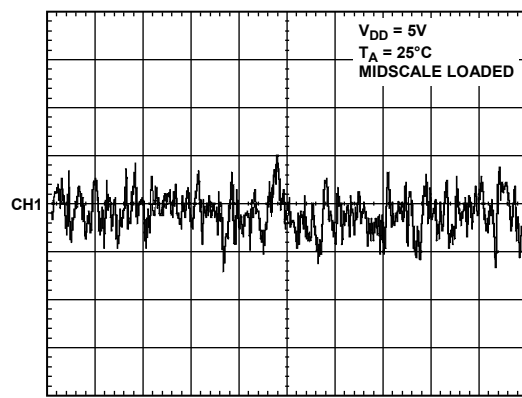
Figure 19. 1/f Noise, 0.1 Hz to 10 Hz Bandwidth
