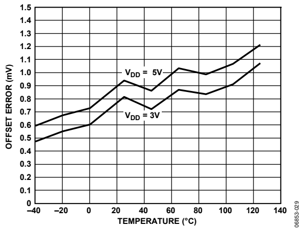
Figure 29. Offset Error vs. Temperature (3 V/5 V Supply)
