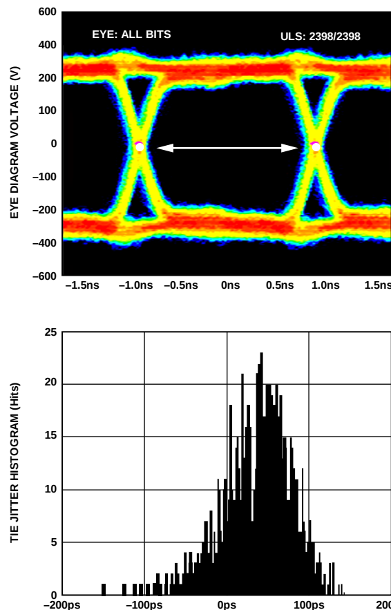
Figure 60. Data Eye for LVDS Outputs in ANSI-644 Mode with Trace Lengths of Less Than 24 Inches on Standard FR-4
