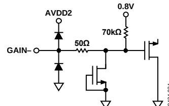
Figure 34. Equivalent GAIN- Input Circuit
