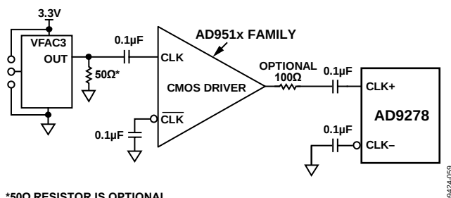
Figure 54. Single-Ended 3.3 V CMOS Sample Clock
