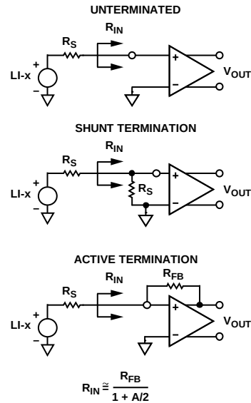
Figure 44. Input Configurations
