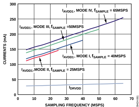
Figure 56. Supply Current vs. f_{\text{SAMPLE}} for f_{\text{IN}} = 5 \text{ MHz}
