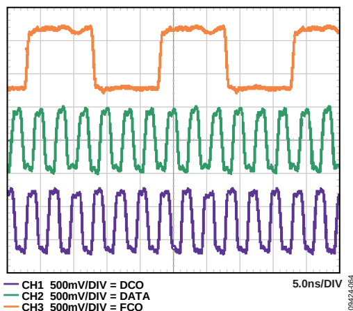
Figure 59. LVDS Output Timing Example in ANSI-644 Mode (Default)
