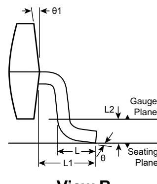
View B
