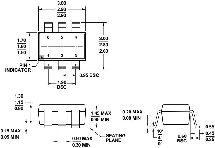
Figure 48. 6-Lead Small Outline Transistor Package [SOT-23] (RJ-6) Dimensions shown in millimeters
