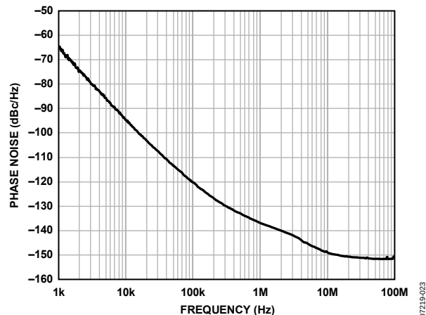
Figure 23. Internal VCO Phase Noise (Absolute), LVDS Output @ 633 MHz
