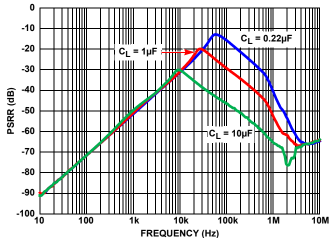
FIGURE 13. RIPPLE REJECTION AT DIFFERENT CAPACITIVE LOADS
