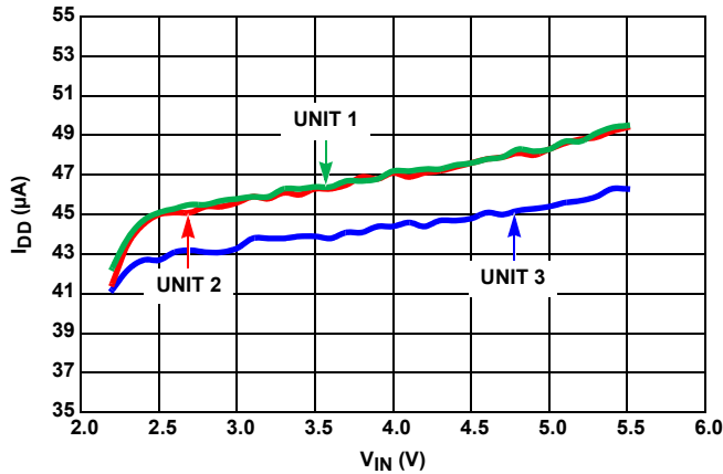
FIGURE 19. I_{IN} vs V_{IN} , THREE UNITS
