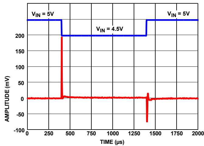
FIGURE 125. LINE TRANSIENT RESPONSE WITH 0.1µF LOAD
