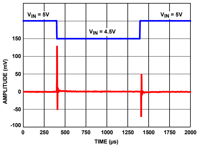
FIGURE 40. LINE TRANSIENT RESPONSE WITH 0.1µF LOAD
