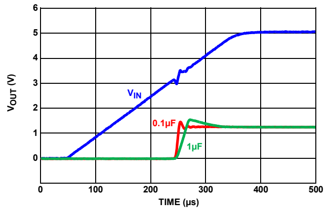
FIGURE 28. TURN-ON TIME
