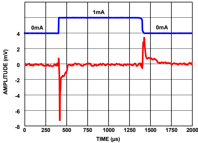
FIGURE 44. LOAD TRANSIENT RESPONSE AT 1mA LOAD AT 1μF
