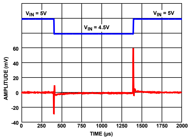
FIGURE 6. LINE TRANSIENT RESPONSE WITH 0.22µF LOAD
