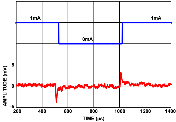
FIGURE 95. LOAD TRANSIENT RESPONSE AT 1mA LOAD AT 1μF
