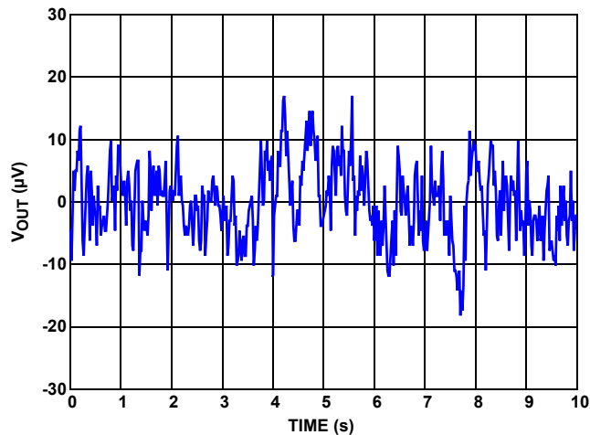
FIGURE 52. V_{OUT} vs NOISE, 0.1Hz TO 10Hz
