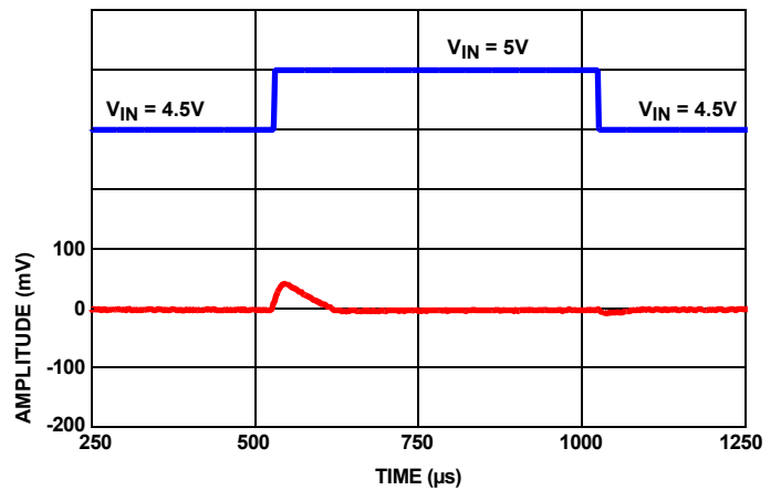
FIGURE 109. LINE TRANSIENT RESPONSE WITH 10µF LOAD
