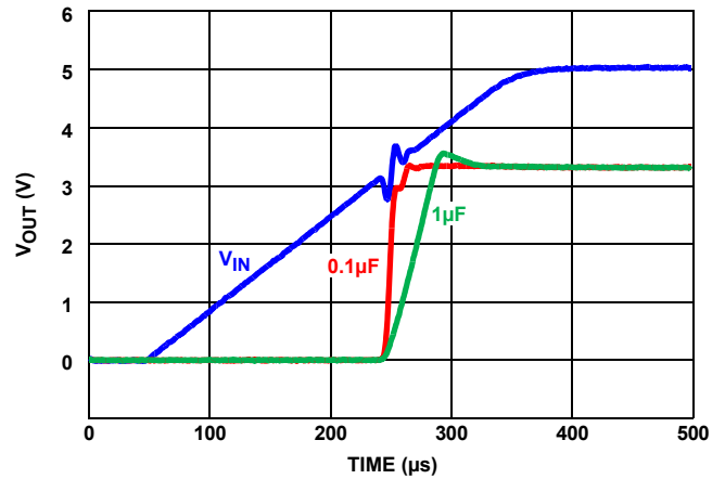
FIGURE 113. TURN-ON TIME
