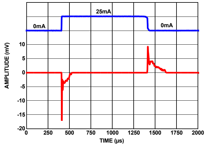
FIGURE 9. LOAD TRANSIENT RESPONSE AT 25mA LOAD AT 1μF
