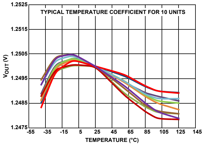
FIGURE 33. V_{OUT} vs TEMPERATURE
