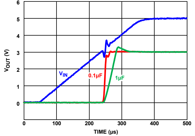
FIGURE 96. TURN-ON TIME
