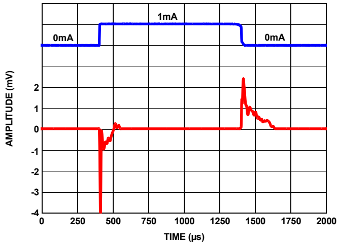
FIGURE 10. LOAD TRANSIENT RESPONSE AT 1mA LOAD AT 1μF
