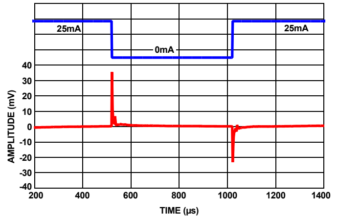
FIGURE 60. LOAD TRANSIENT RESPONSE AT 25mA LOAD AT 1μF
