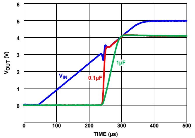
FIGURE 130. TURN-ON TIME
