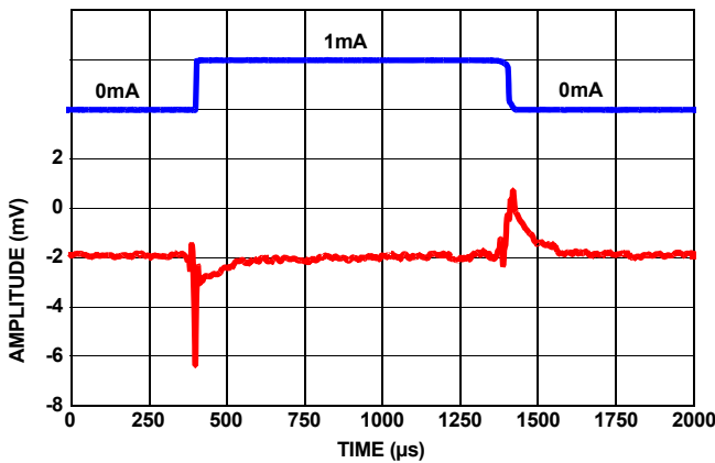
FIGURE 27. LOAD TRANSIENT RESPONSE AT 1mA LOAD AT 1μF
