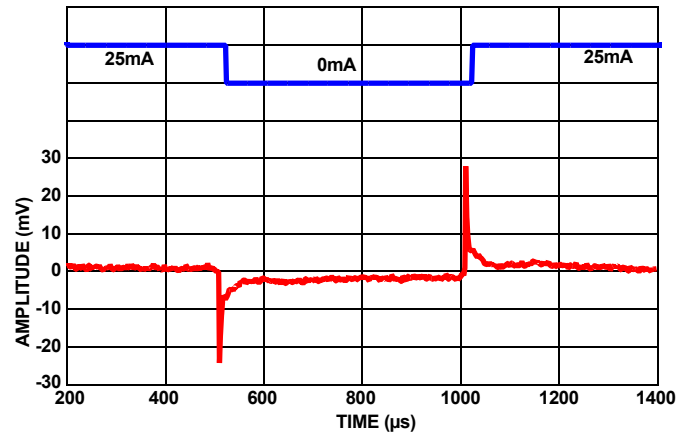
FIGURE 94. LOAD TRANSIENT RESPONSE AT 25mA LOAD AT 1μF
