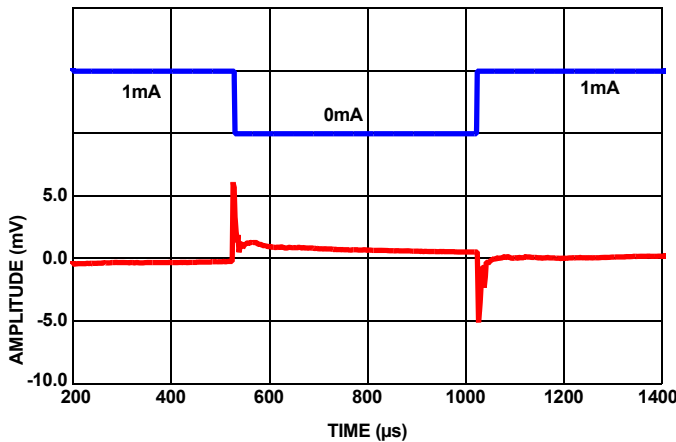
FIGURE 112. LOAD TRANSIENT RESPONSE AT 1mA LOAD AT 1μF
