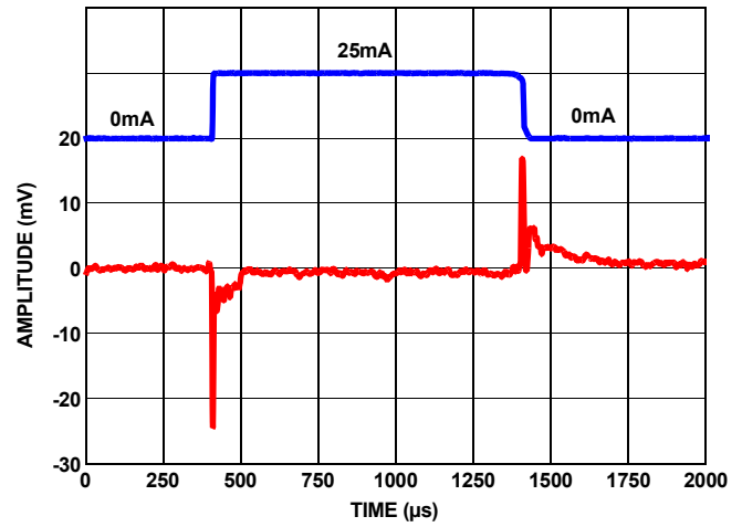
FIGURE 43. LOAD TRANSIENT RESPONSE AT 25mA LOAD AT 1μF
