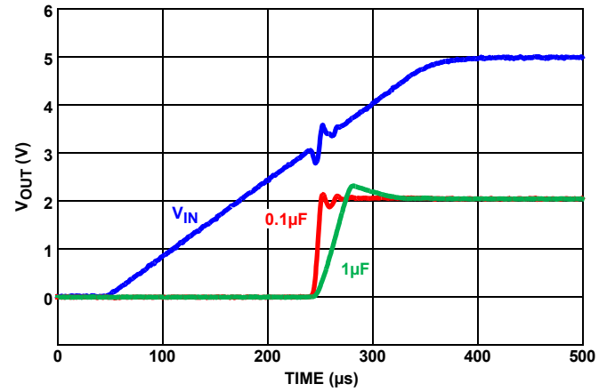
FIGURE 62. TURN-ON TIME
