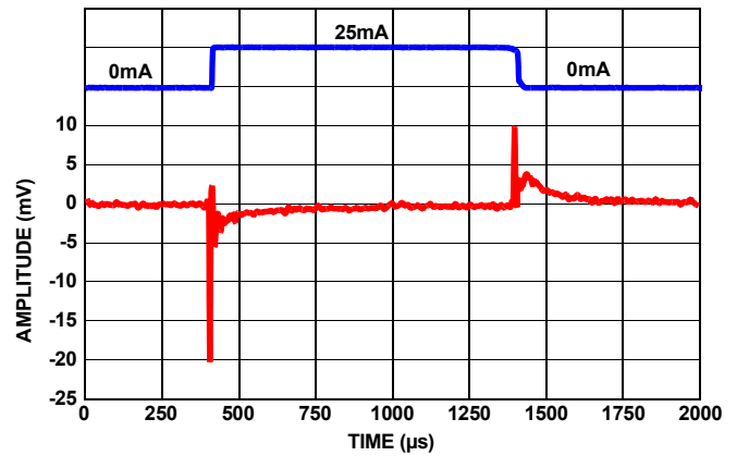
FIGURE 26. LOAD TRANSIENT RESPONSE AT 25mA LOAD AT 1μF
