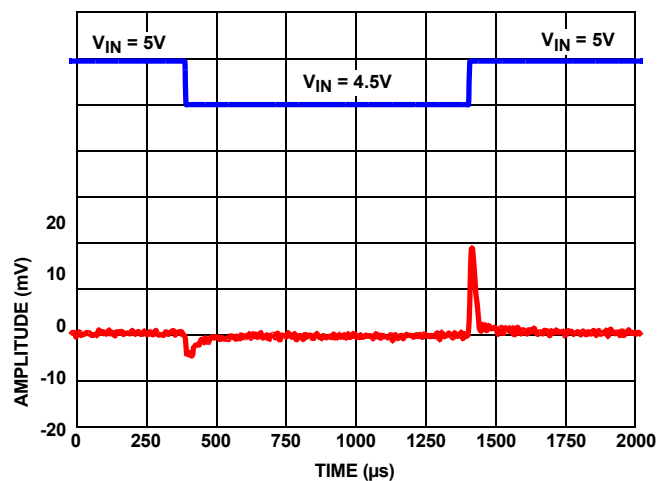
FIGURE 7. LINE TRANSIENT RESPONSE WITH 10µF LOAD
