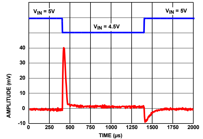
FIGURE 126. LINE TRANSIENT RESPONSE WITH 10µF LOAD
