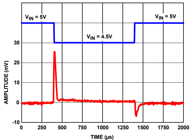
FIGURE 41. LINE TRANSIENT RESPONSE WITH 10µF LOAD
