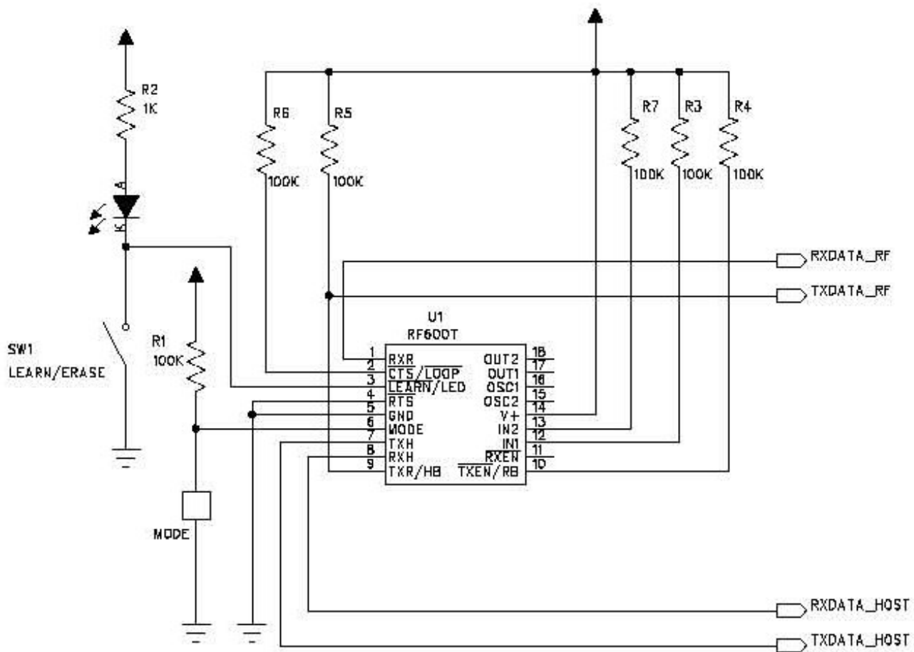
RF600T application circuit – minimum implementation.
