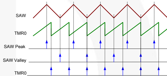
Figure 25. ADC Trigger Mode
