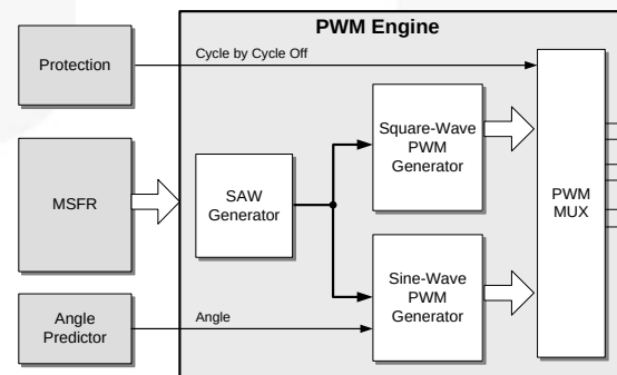
Figure 15. PWM Engine Block Diagram
