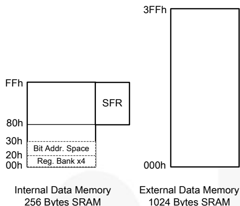
Figure 22. Data Memory Map
