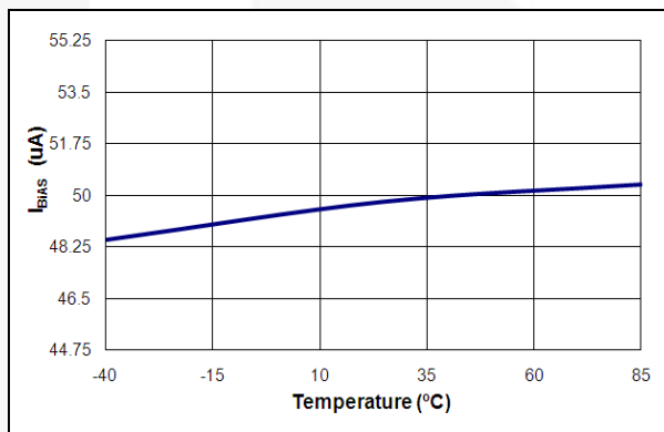
Figure 12. Current Source of IA/IB/IC ( I_{BIAS} ) vs. Temperature
