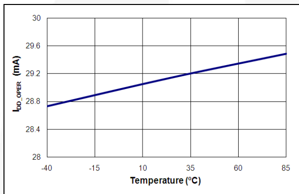
Figure 11. V_{DD} Operation Current ( I_{DD\_OPPE} ) vs. Temperature
