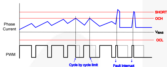
Figure 26. Current Protection (Square-Wave)
