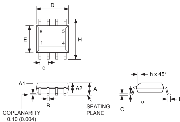
Figure 14.1 : Physical dimensions, 8-lead SOIC package
