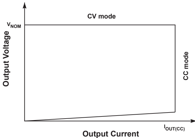
Figure 9.5 : Power Envelope
