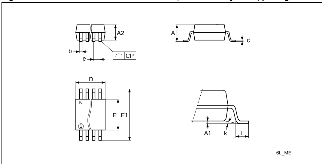
Figure 31. SO8W 8 lead Plastic Small Outline, 208 mils body width, package outline
