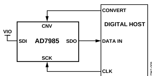
Figure 26. \overline{\text{CS}} Mode, 3-Wire Without Busy Indicator Connection Diagram ( \text{SDI} High)
