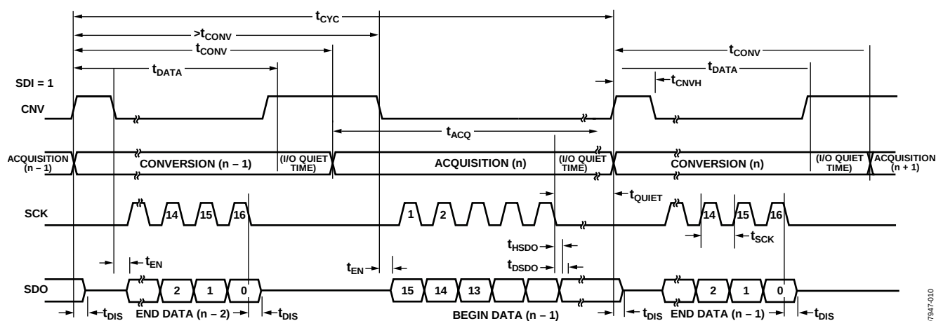
Figure 27. \overline{\text{CS}} Mode, 3-Wire Without Busy Indicator Serial Interface Timing ( \text{SDI} High)
