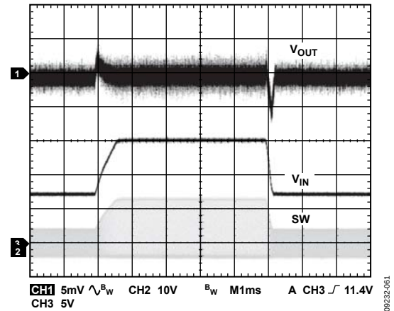
Figure 11. ADP2301 Line Transient, 7 V to 15 V, V_{OUT} = 3.3 V, I_{OUT} = 1.2 A, f_{SW} = 1.4 MHz
