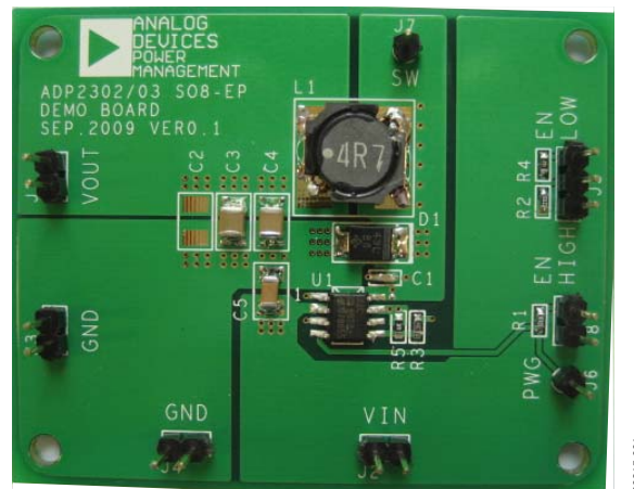
Figure 1. ADP2302/ADP2303 Evaluation Board
