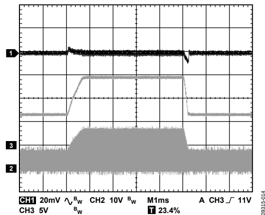
Figure 14. ADP2303 Line Transient, 7 V to 15 V, V_{OUT} = 3.3 V, I_{OUT} = 3 A, L = 4.7 \mu H, C_{OUT} = 2 \times 47 \mu F
