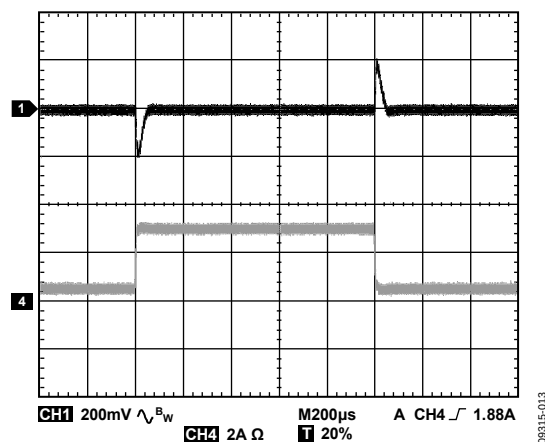
Figure 13. ADP2303 Load Transient, 0.5 A to 3.0 A, V_{OUT} = 3.3 V, V_{IN} = 12 V, L = 4.7 \mu H, C_{OUT} = 2 \times 47 \mu F
