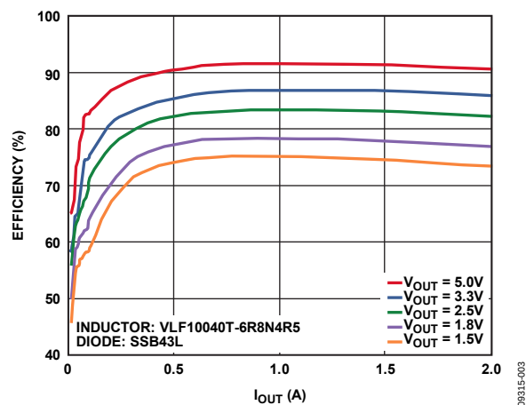
Figure 3. ADP2302 Efficiency, V_{IN} = 12\text{ V}
