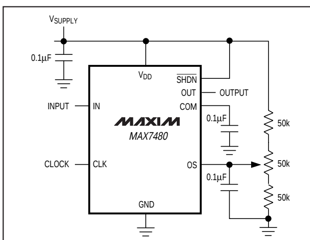
Figure 3. Offset Adjustment Circuit
