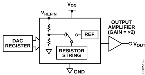
Figure 55. DAC Architecture
