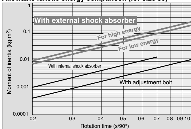
Allowable kinetic energy comparison (for size 30)
