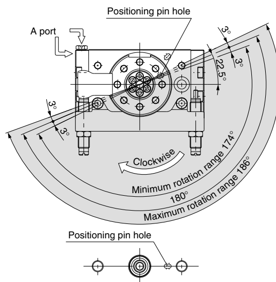
Position of bottom positioning pin hole
