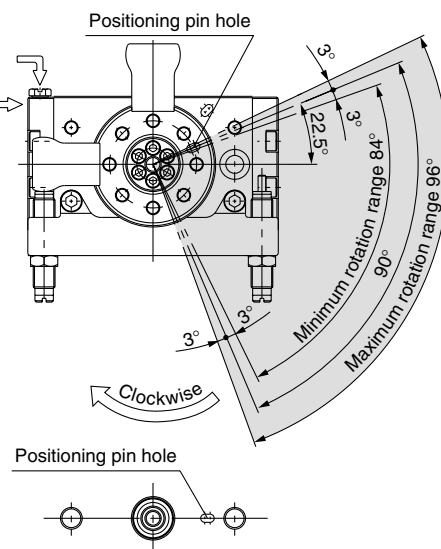
Position of bottom positioning pin hole
