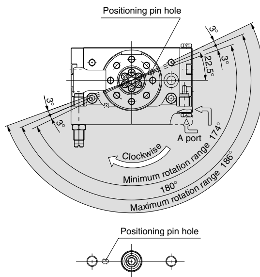
Position of bottom positioning pin hole
