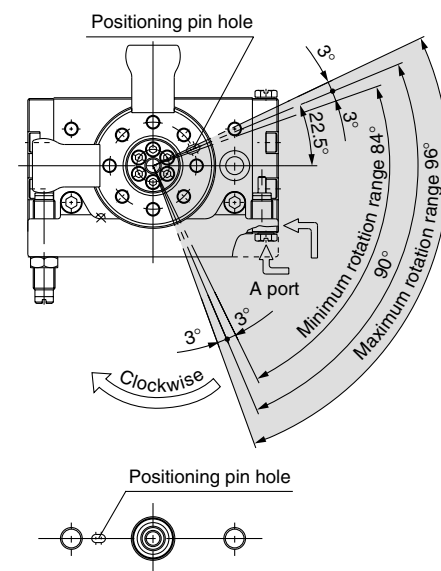
Position of bottom positioning pin hole
