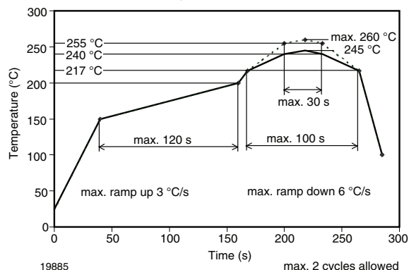
Fig. 12 - Vishay Lead (Pb)-free Reflow Soldering Profile (acc. to J-STD-020)
