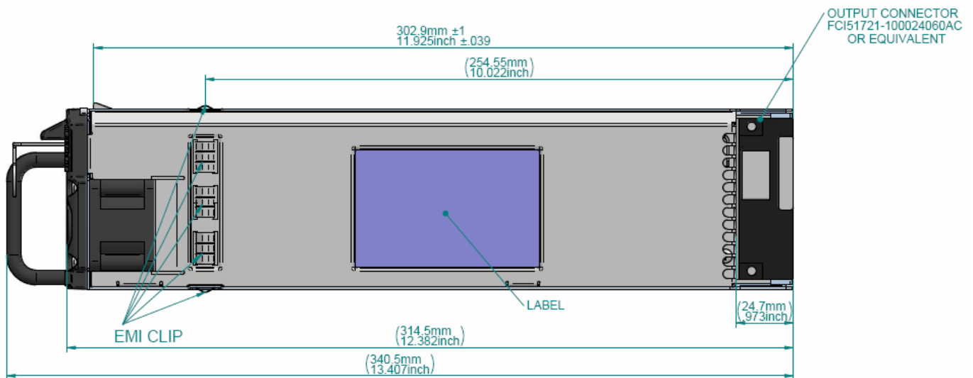
TOP VIEW
