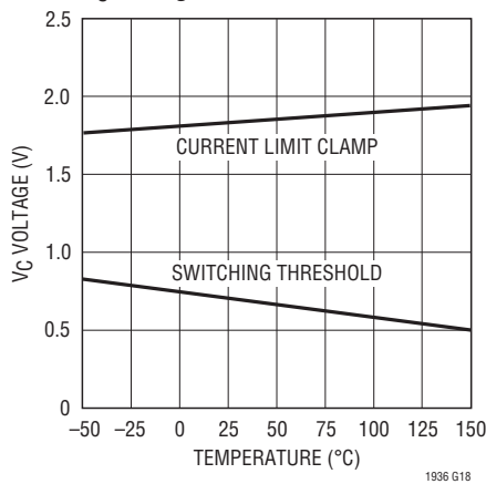
V_C Voltages
