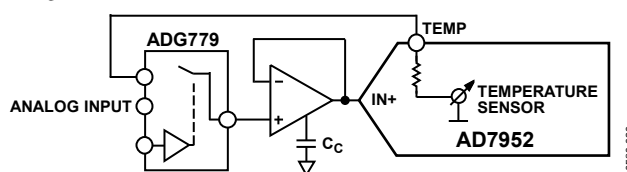
Figure 31. Use of the Temperature Sensor
