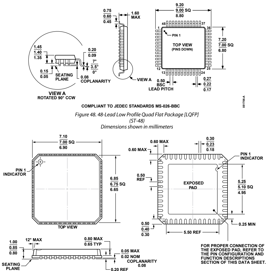
Figure 49. 48-Lead Lead Frame Chip Scale Package [LFCSP_VQ] 7 mm × 7 mm Body, Very Thin Quad (CP-48-1)
