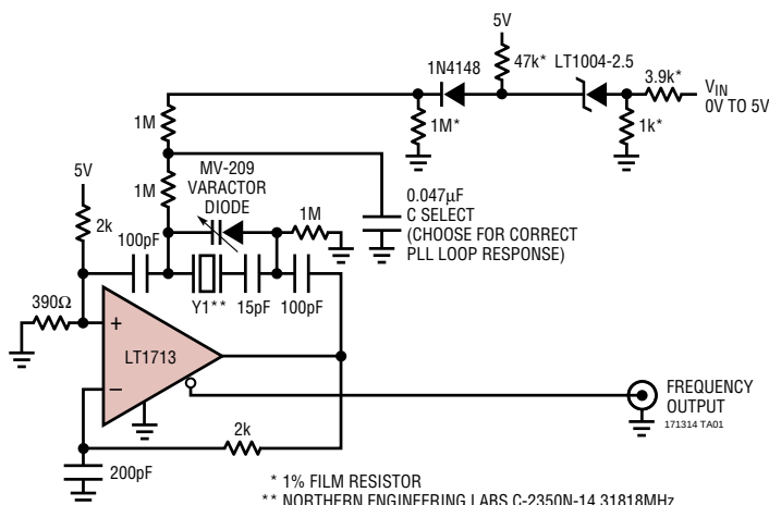
A 4 \times NTSC Subcarrier Voltage-Tunable Crystal Oscillator
