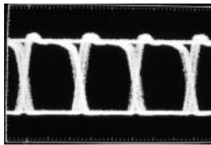
Figure 5. Performance When Operated Simultaneously Bidirectionally (Full Duplex). Crosstalk Appears as Noise. Eye is Slightly Shut But Performance is Still Excellent
