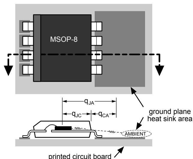
Figure 1. Thermal Resistance
