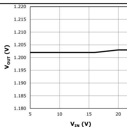
Figure 2: XR76112 Line Regulation
