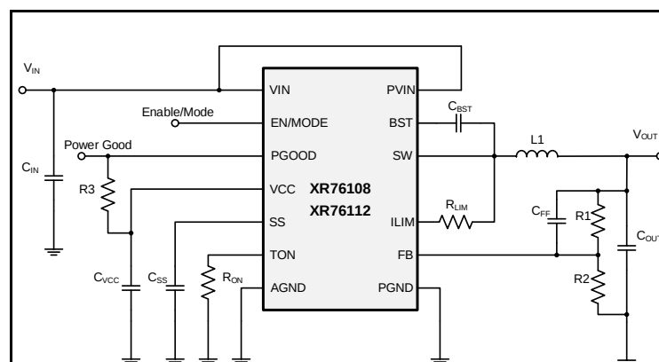
Figure 1: XR76108/12 Application Diagram
