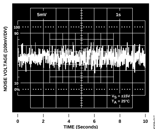
Figure 16. 0.1 Hz to 10 Hz Noise Voltage
