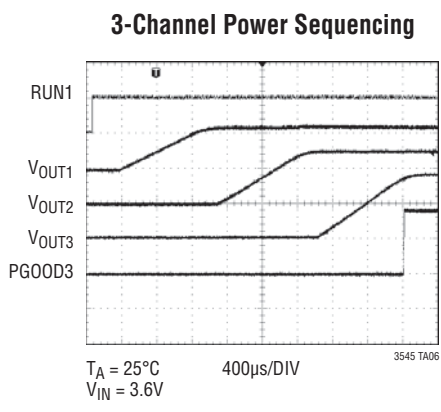
Figure 5. LTC3545-1 Three PG00Ds and Power Sequencing
