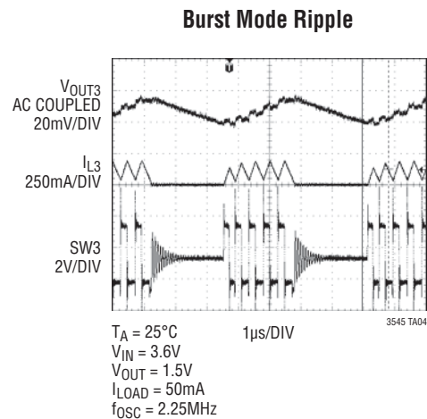
Figure 4. LTC3545 Low Ripple Burst Mode Operation
