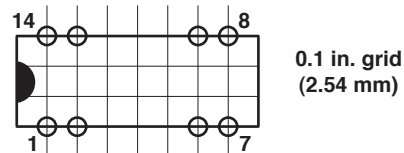
Circuit board pin spacing viewed from component side
