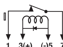
Figure D SPST-NC With diode
