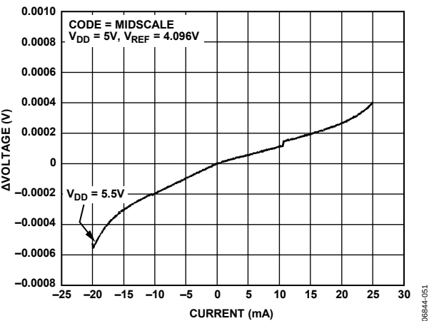
Figure 33. Typical Output Load Regulation
