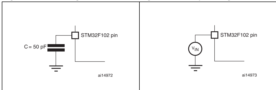
Figure 7. Pin input voltage
