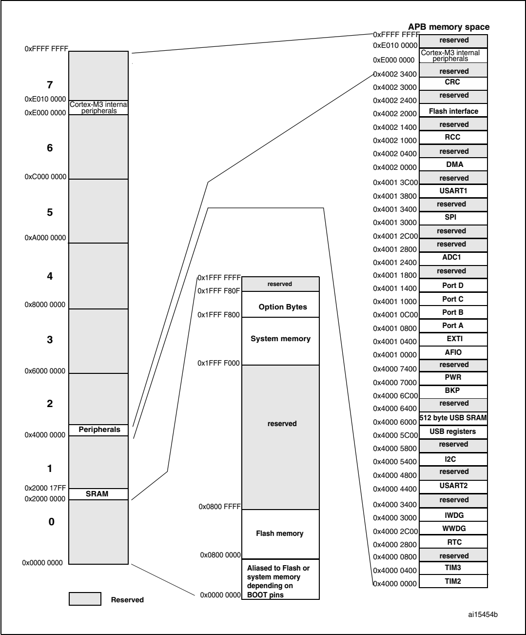
Figure 5. Memory map
