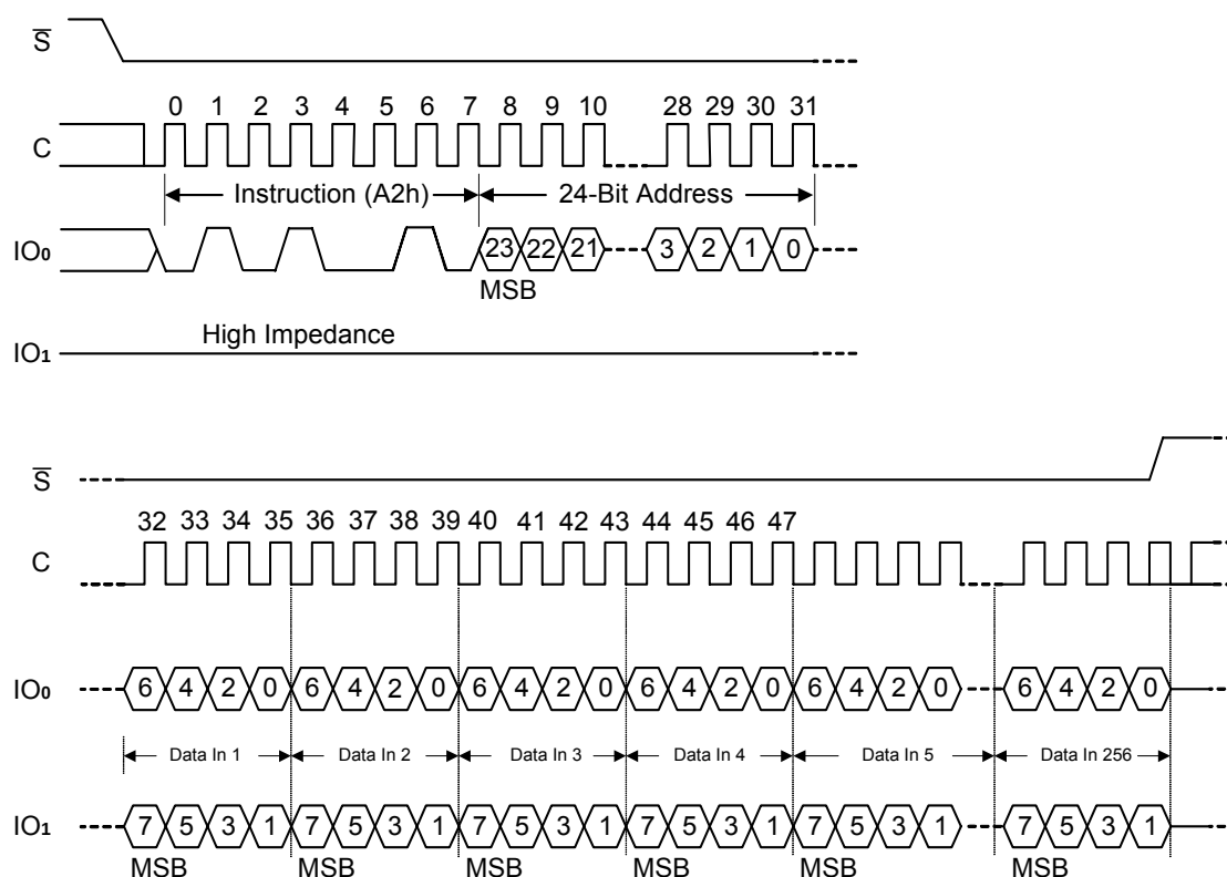
Figure 17. Dual Input Fast Program (DIFP) instruction sequence
