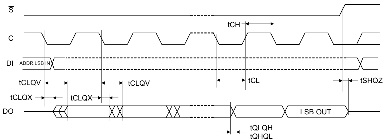
Figure 37. Output Timing
