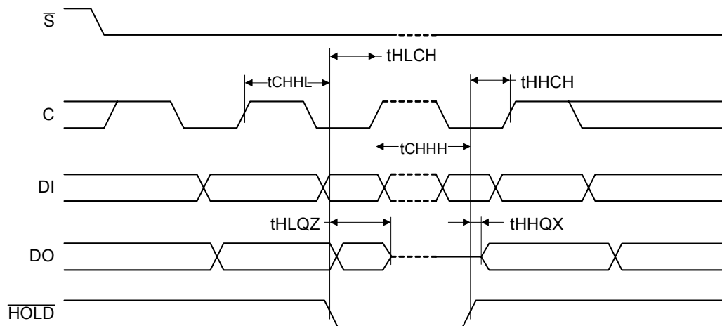
Figure 36. Hold Timing
