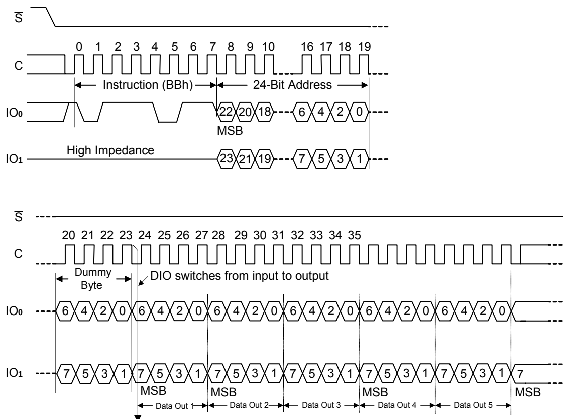
Figure 10. FAST_READ_DUAL_INPUT_OUTPUT Instruction Sequence and Data-Out Sequence
