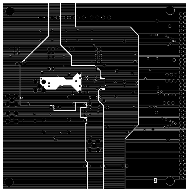
Figure 44. PCB Split Power Plane
