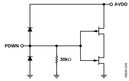
Figure 26. Power-Down Input
